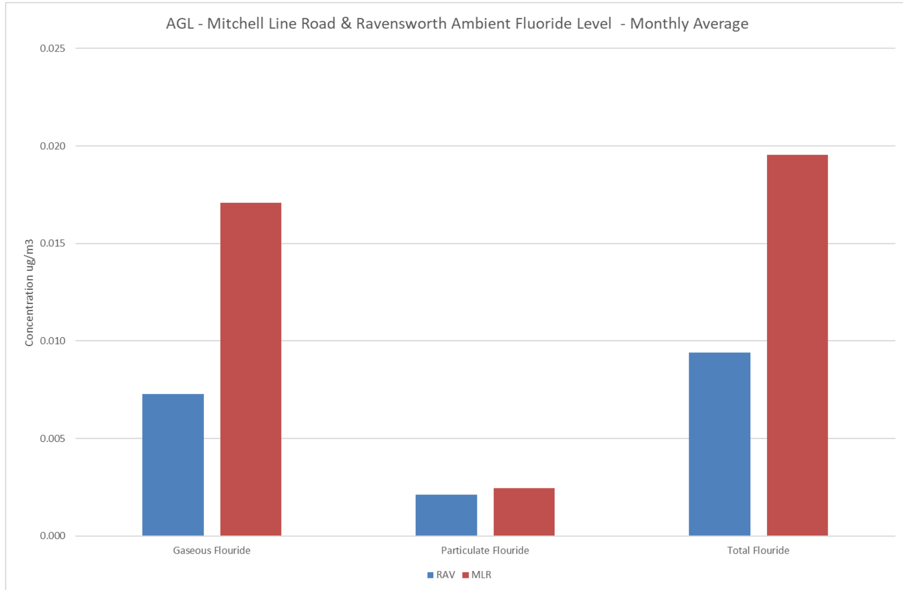
Graph 4 Fluoride monthly averages.
