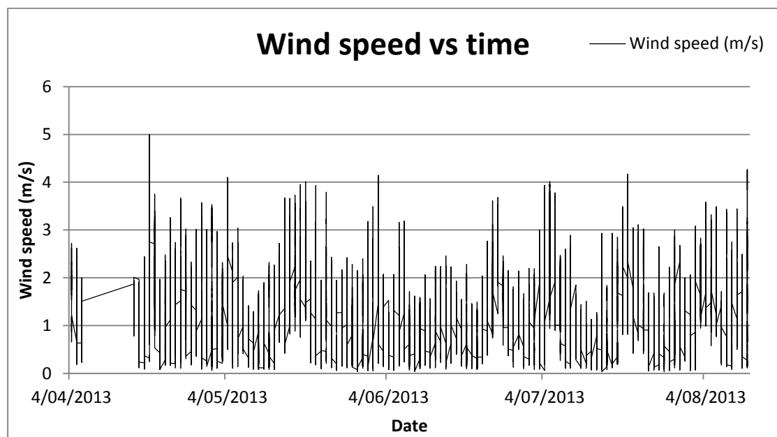
Figure 2: Wind speed for 3 April 2013 - 12 August 2013
