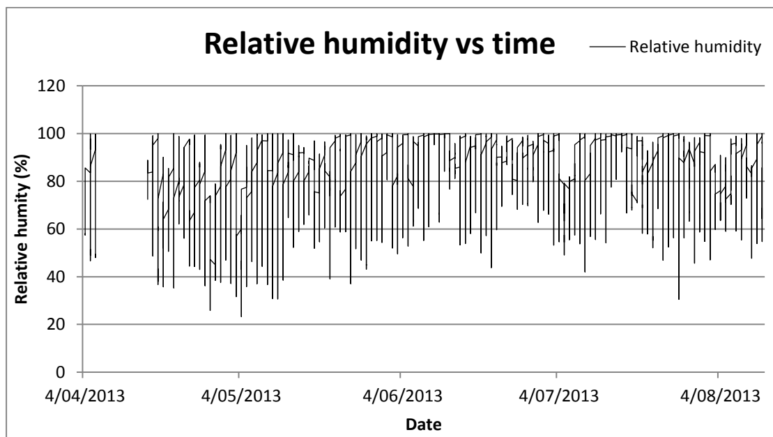
Figure 8: Relative humidity for 3 April 2013 - 12 August 2013
