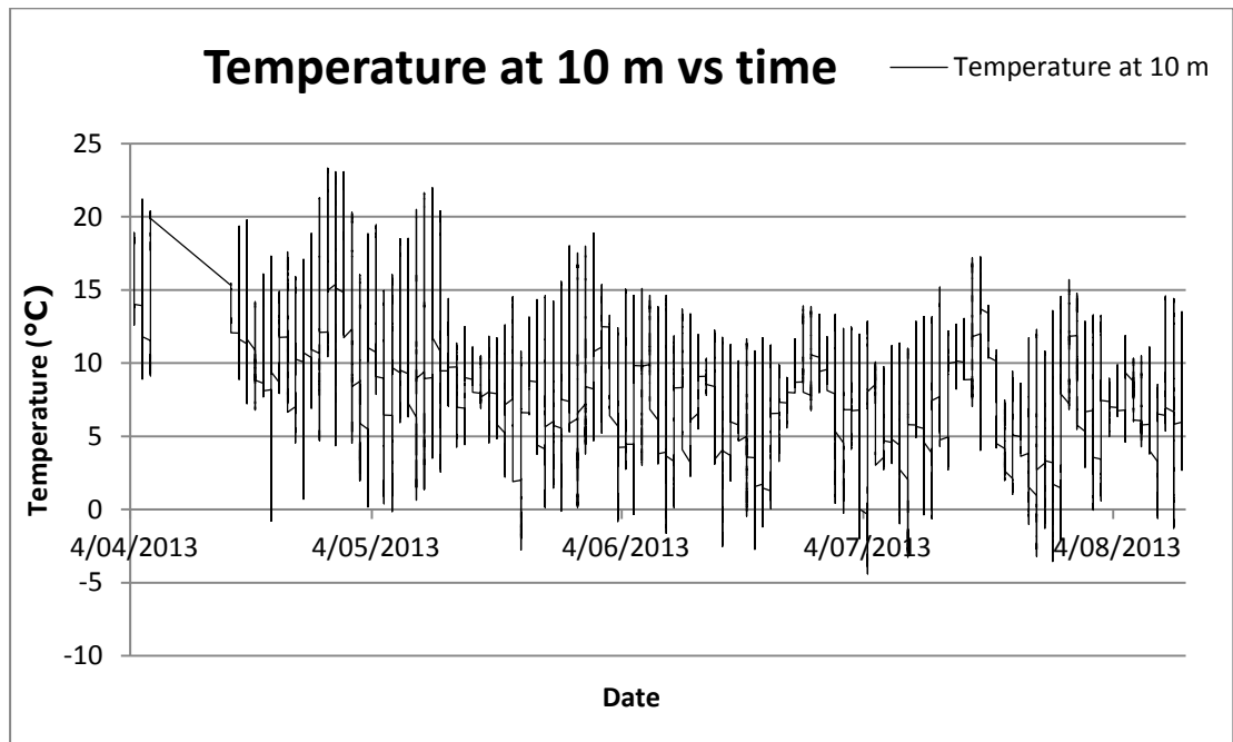
Figure 6: Temperature at 10 m for 3 April 2013 - 12 August 2013
