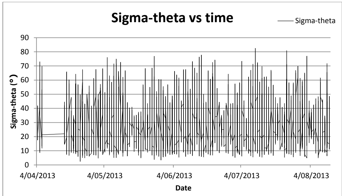
Figure 7: Sigma-theta for 3 April 2013 - 12 August 2013
