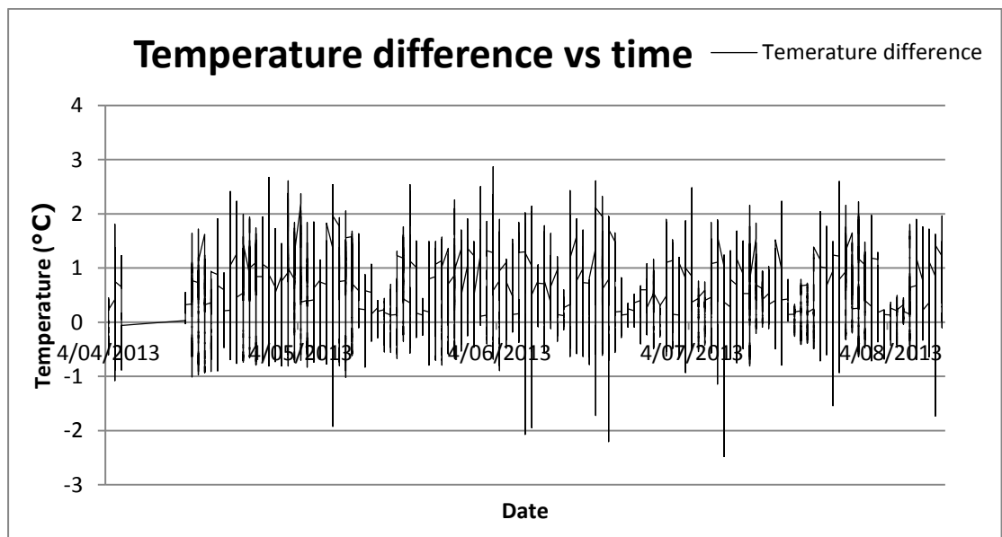
Figure 4: Measured temperature difference for 3 April 2013 - 12 August 2013 (temperature at 10 metres subtracting temperature at 2 metres – a positive value indicates an inversion over this range).
