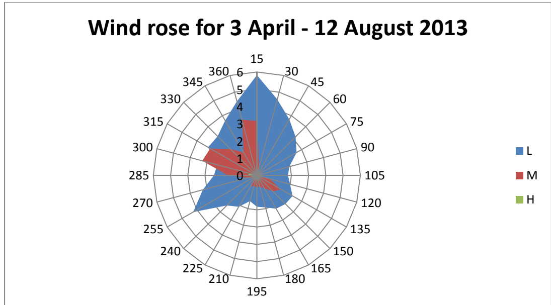
Figure 3: Wind rose for 3 April 2013 - 12 August 2013. In this figure, L represents speeds below 1.5 m/s, M between 1.5 and 3.0 m/s and H above 4.5 m/s. The central axes are percentages of occurrence.
