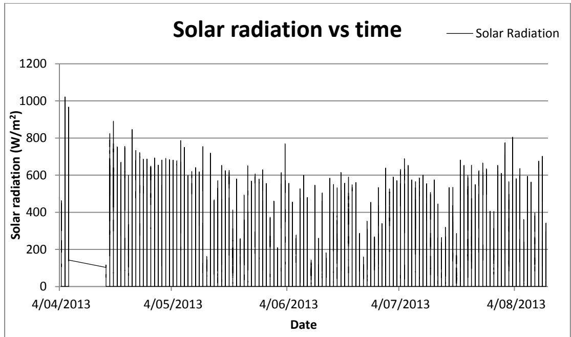
Figure 9: Solar radiation for 3 April 2013 - 12 August 2013
