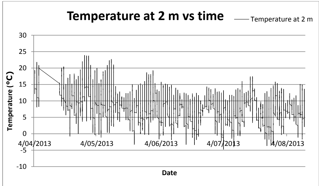
Figure 5: Temperature at 2 m for 3 April 2013 - 12 August 2013
