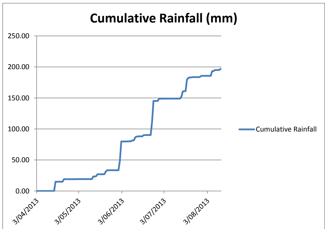
Figure 10: Rainfall for 3 April 2013 - 12 August 2013
