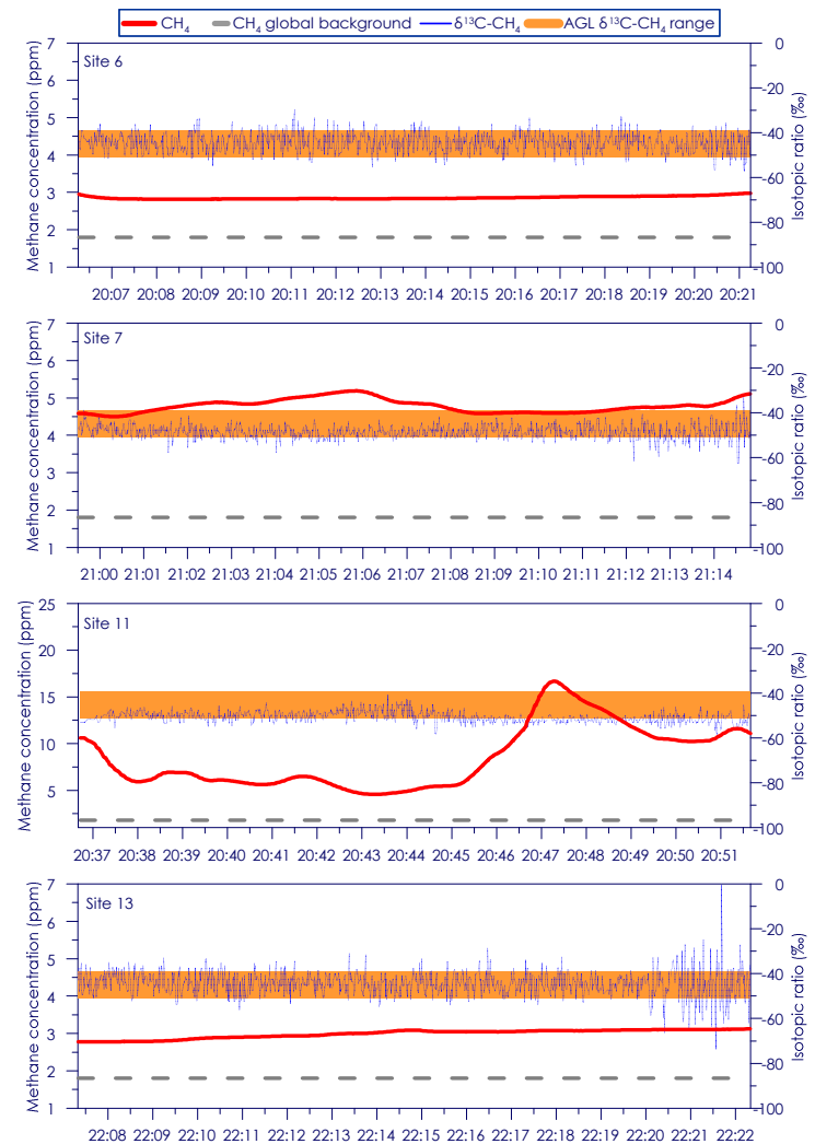
Figure D - 2: Time series of CH 4 concentration and isotopic ratio for Site 6, Site 7, Site 11 and Site 13 - Week 11 night monitoring
