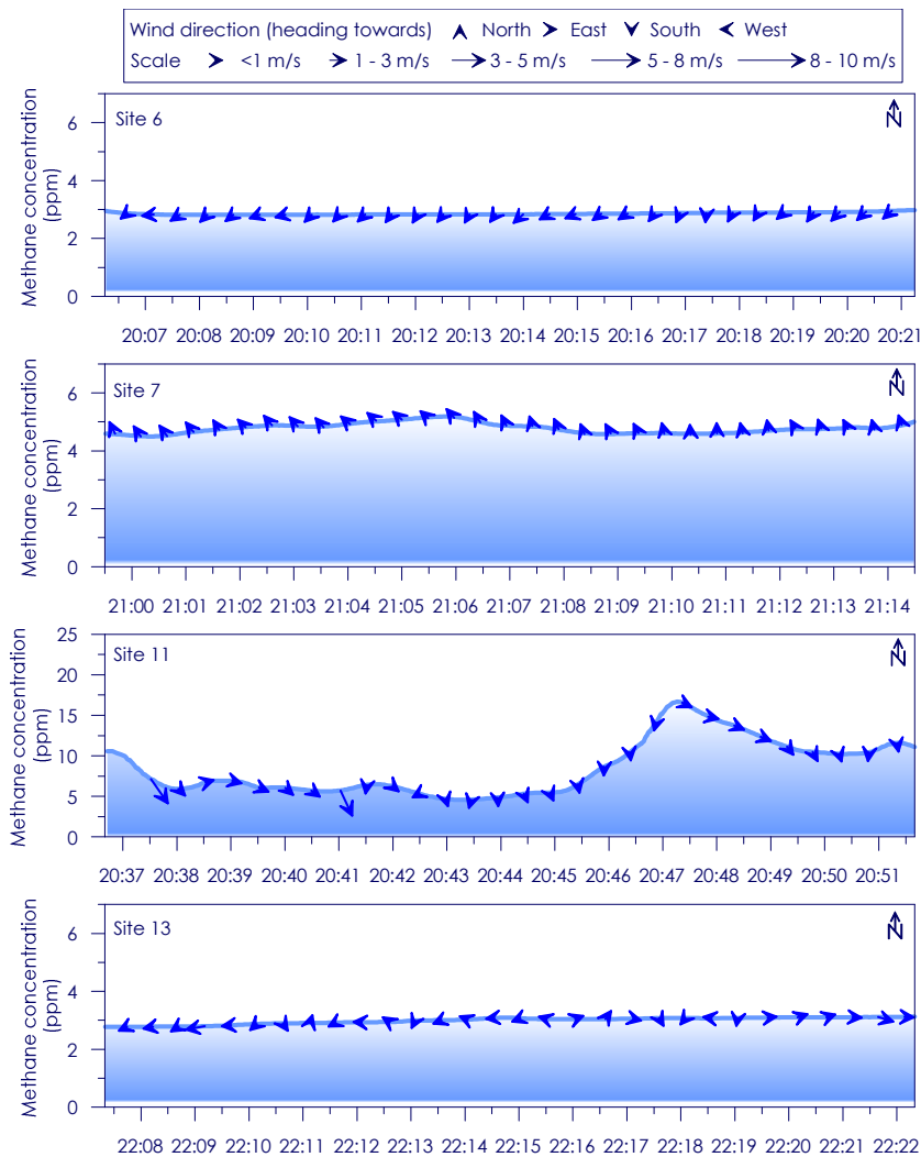
Figure D - 1: Time series of CH 4 concentration, wind speed and wind direction for Site 6, Site 7, Site 11 and Site 13 - Week 11 night monitoring
