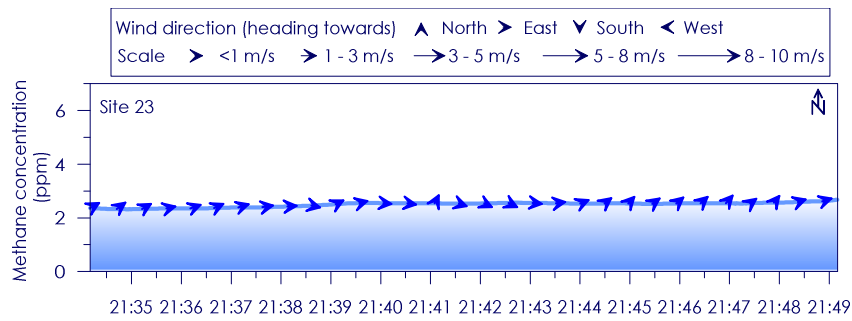
Figure D - 5: Time series of CH 4 concentration, wind speed and wind direction for Site 23 - Week 11 night monitoring
