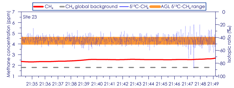
Figure D - 6: Time series of CH 4 concentration and isotopic ratio for Site 23 - Week 11 night monitoring
