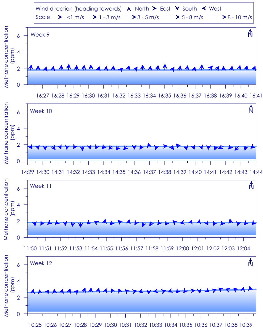
Figure C - 23: Time series of CH 4 concentration, wind speed and wind direction for Site 4 Weeks 9 - 12
