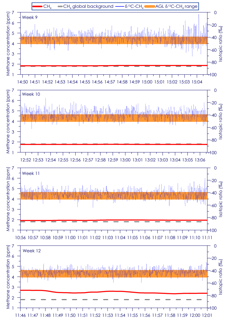
Figure C - 36: Time series of CH 4 concentration and isotopic ratio for Site 6 Weeks 9 - 12
