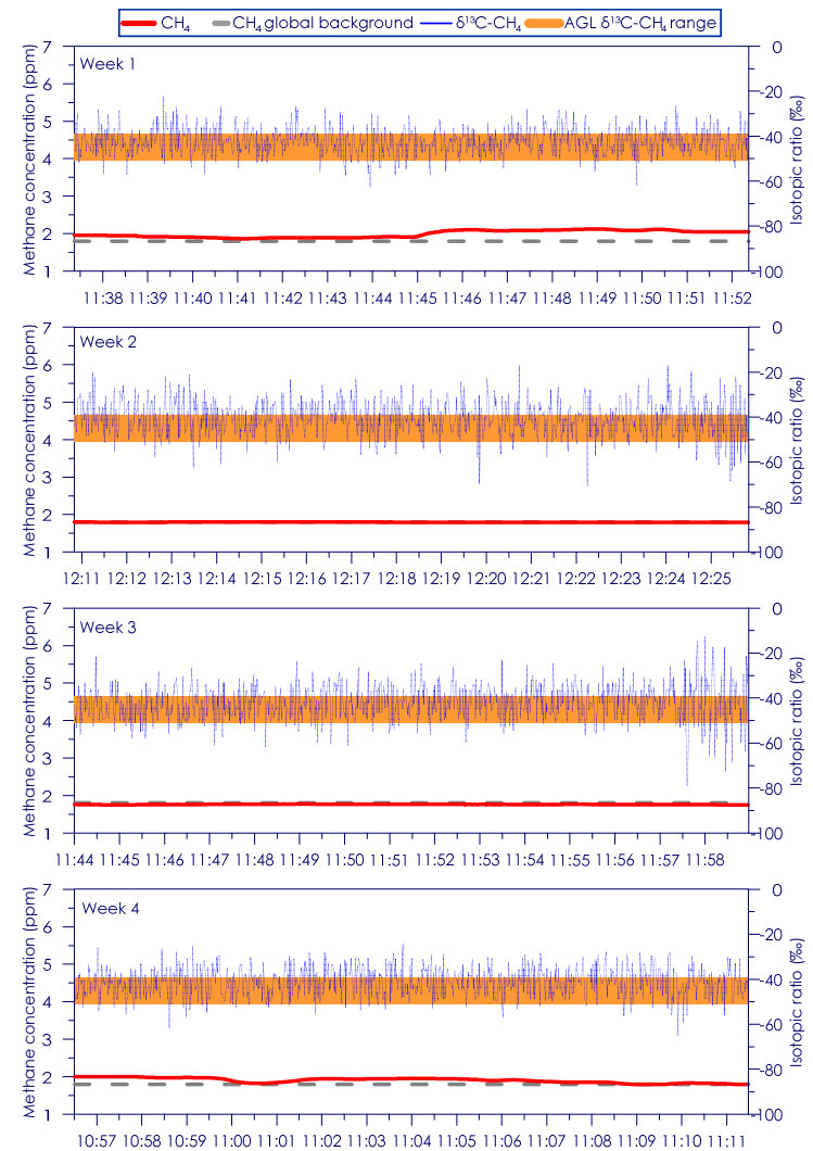
Figure C - 38: Time series of CH 4 concentration and isotopic ratio for Site 7 Weeks 1 - 4
