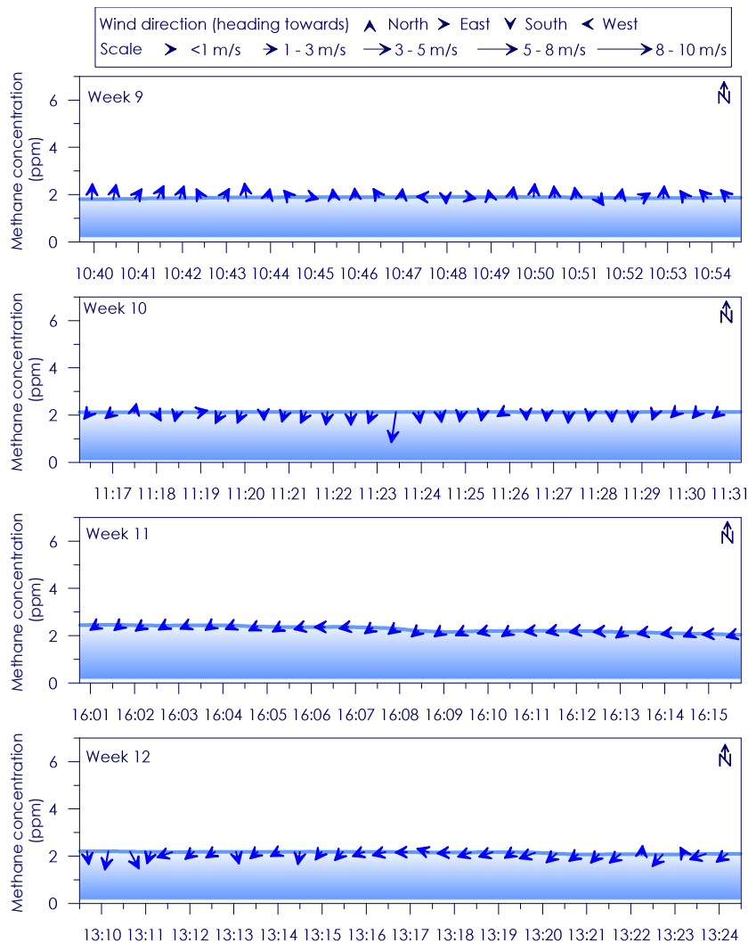
Figure C - 95: Time series of CH 4 concentration, wind speed and wind direction for Site 16 Weeks 9 - 12
