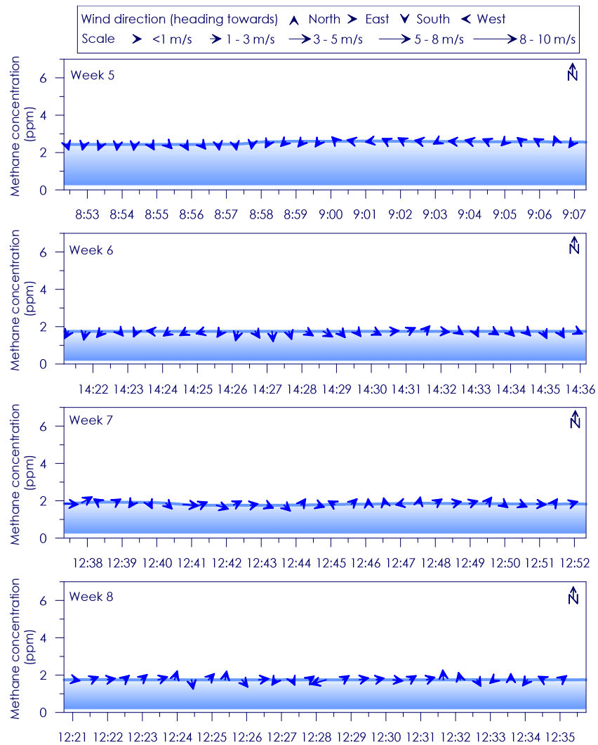
Figure C - 147: Time series of CH 4 concentration, wind speed and wind direction for Site 25 Weeks 5- 8
