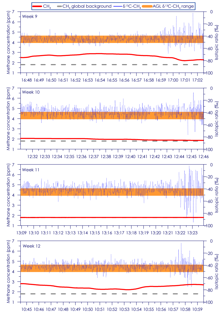
Figure C - 132: Time series of CH 4 concentration and isotopic ratio for Site 22 Weeks 9 - 12
