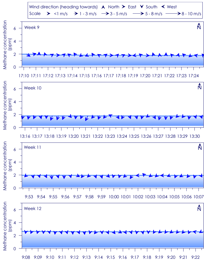
Figure C - 17: Time series of CH 4 concentration, wind speed and wind direction for Site 3 Weeks 9 - 12
