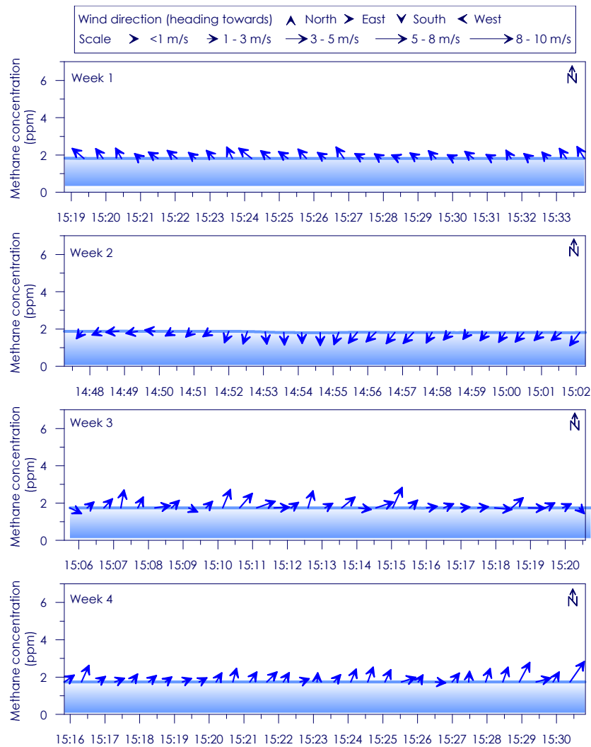
Figure C - 115: Time series of CH 4 concentration, wind speed and wind direction for Site 20 Weeks 1 - 4
