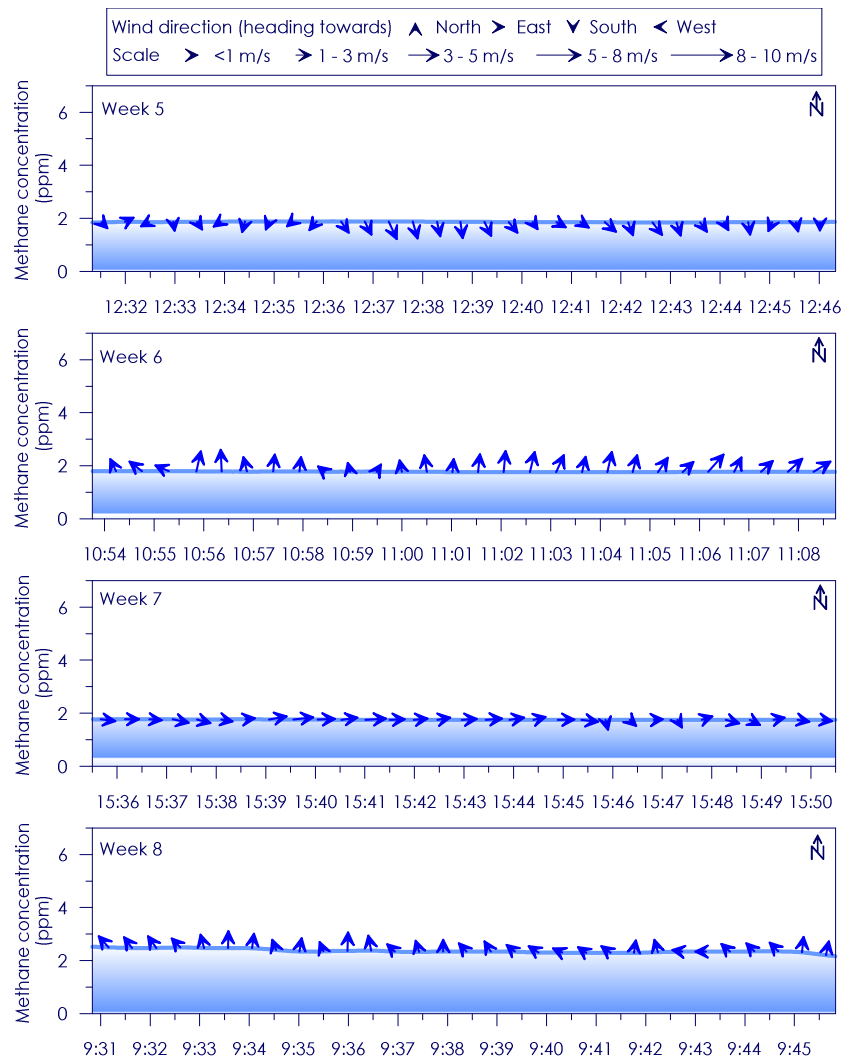
Figure C - 3: Time series of CH 4 concentration, wind speed and wind direction for Site 1 Weeks 5 - 8
