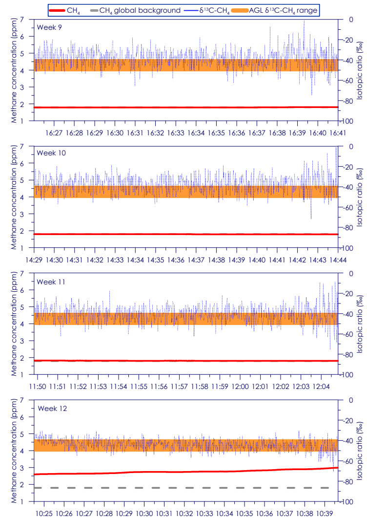
Figure C - 24: Time series of CH 4 concentration and isotopic ratio for Site 4 Weeks 9 - 12
