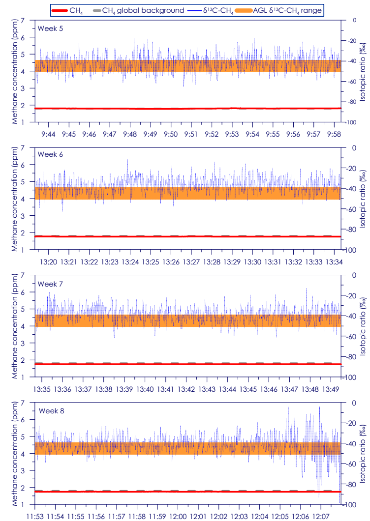
Figure C - 28: Time series of CH 4 concentration and isotopic ratio for Site 5 Weeks 5 - 8
