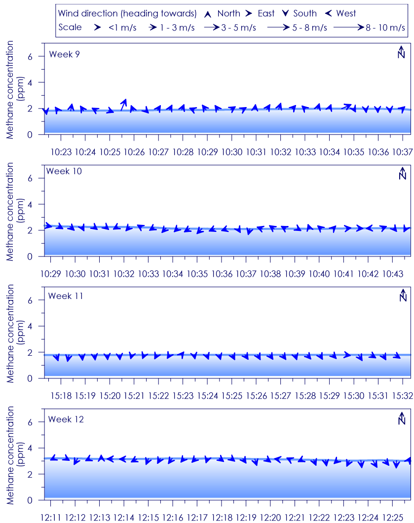
Figure C - 113: Time series of CH 4 concentration, wind speed and wind direction for Site 19 Weeks 9 - 12
