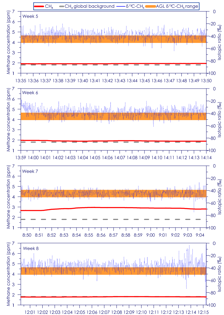
Figure C - 136: Time series of CH 4 concentration and isotopic ratio for Site 23 Weeks 5 - 8
