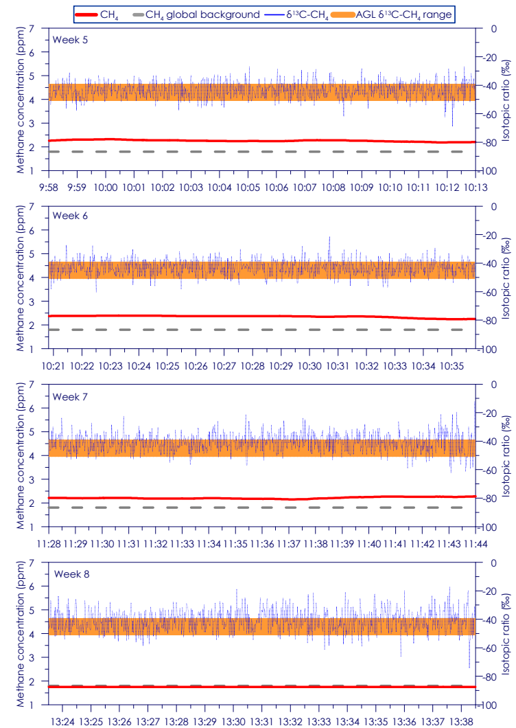
Figure C - 34: Time series of CH 4 concentration and isotopic ratio for Site 6 Weeks 5 - 8
