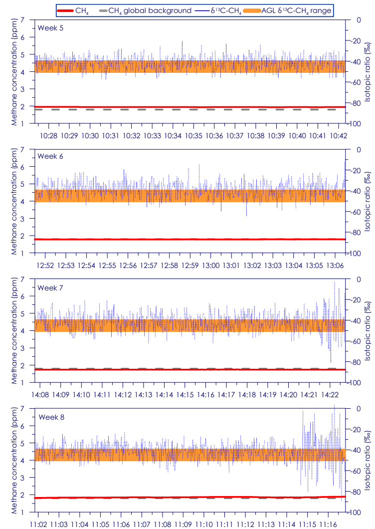
Figure C - 16: Time series of CH 4 concentration and isotopic ratio for Site 3 Weeks 5 - 8
