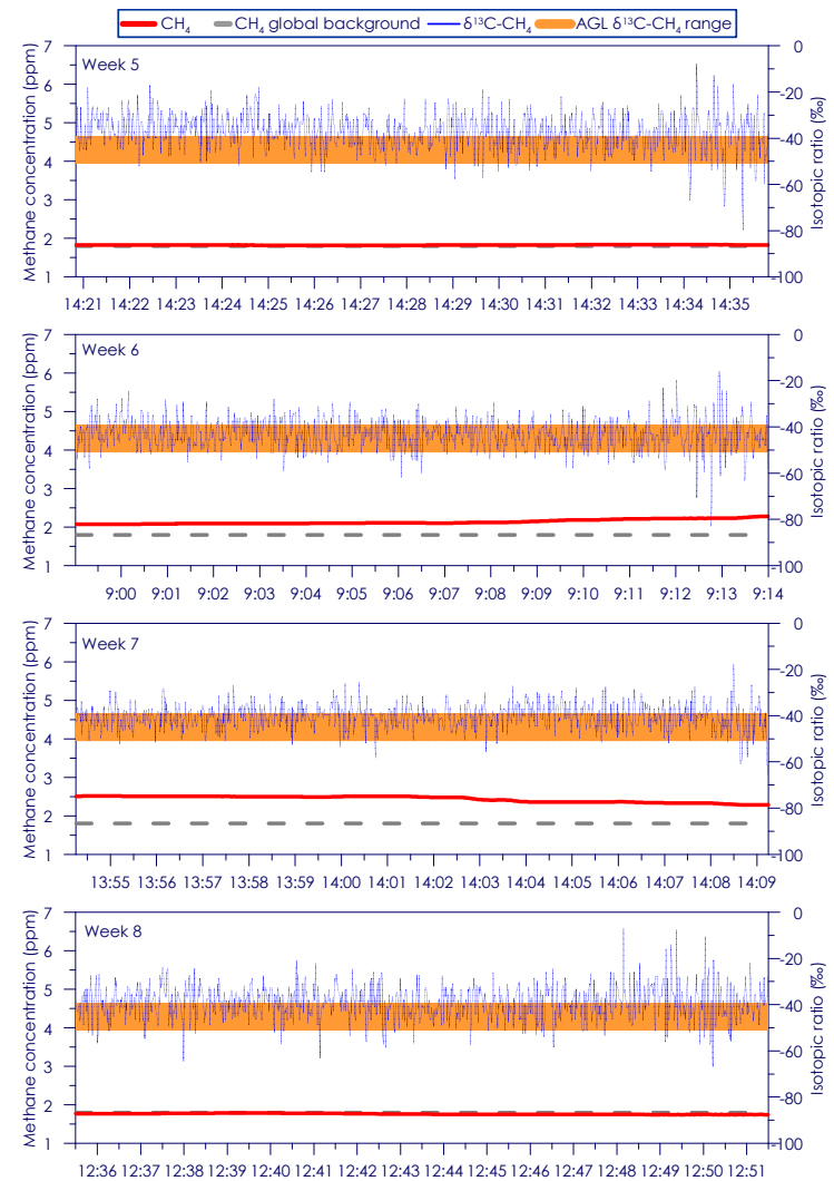
Figure C - 76: Time series of CH 4 concentration and isotopic ratio for Site 13 Weeks 5 - 8
