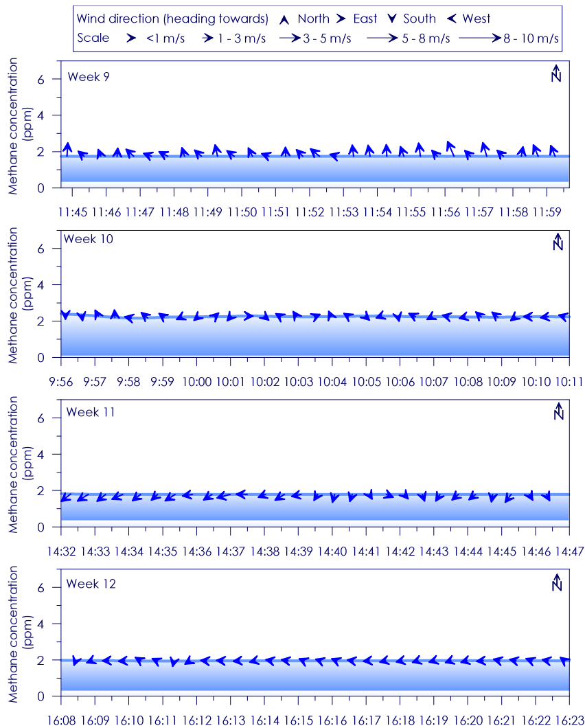
Figure C - 83: Time series of CH 4 concentration, wind speed and wind direction for Site 14 Weeks 9 - 12
