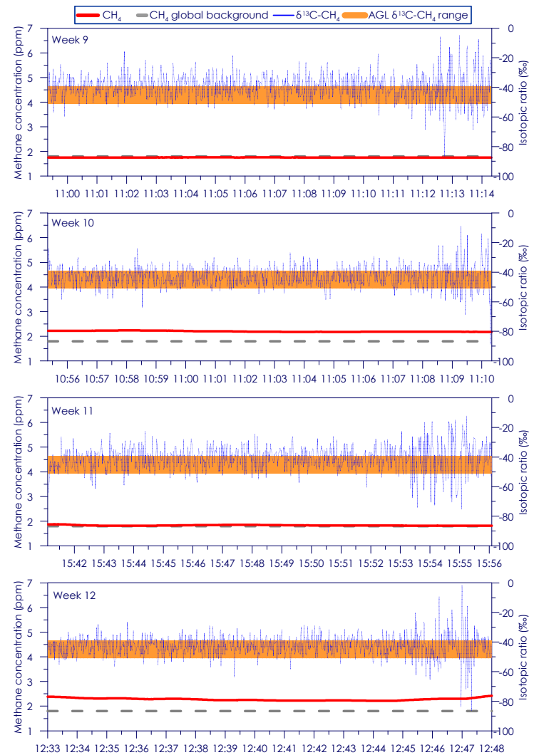
Figure C - 90: Time series of CH 4 concentration and isotopic ratio for Site 15 Weeks 9 - 12
