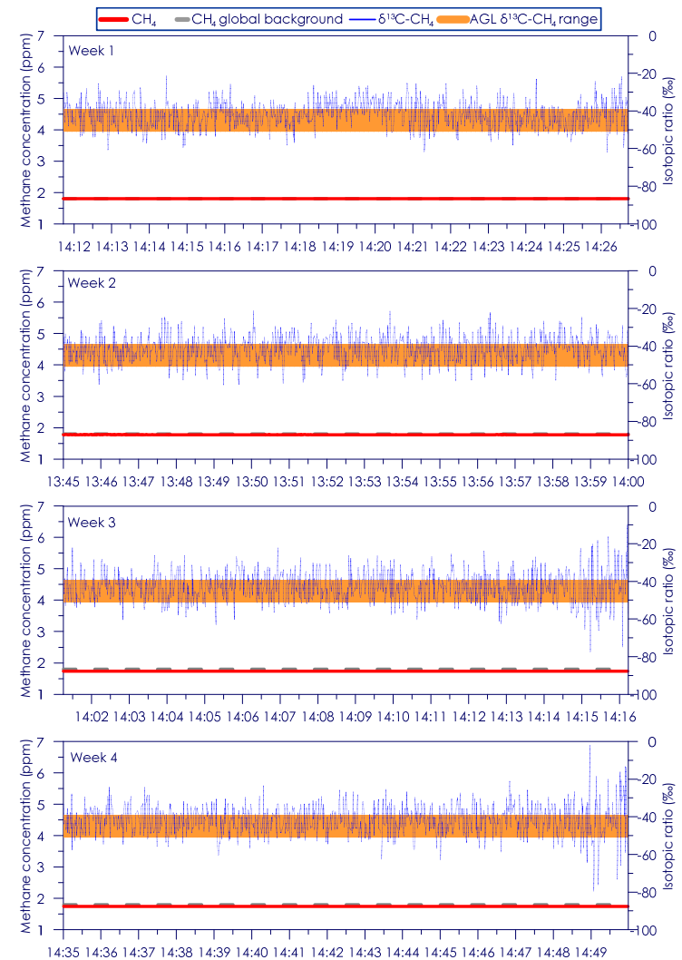
Figure C - 146: Time series of CH 4 concentration and isotopic ratio for Site 25 Weeks 1 - 4
