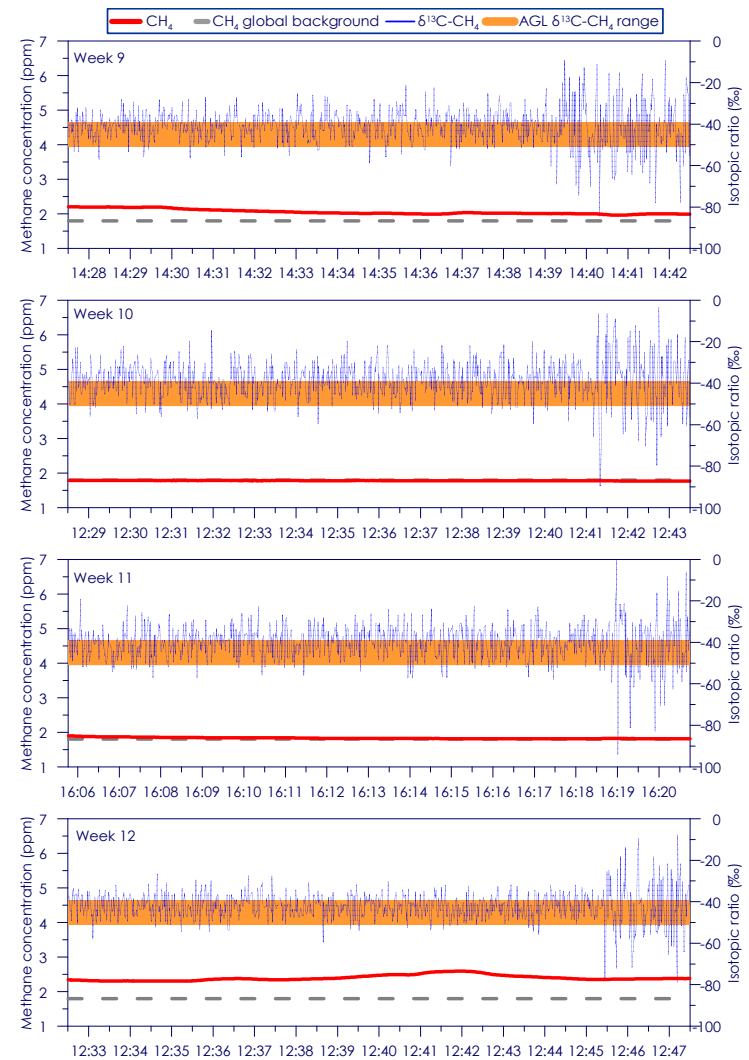
Figure C - 72: Time series of CH 4 concentration and isotopic ratio for Site 12 Weeks 9 - 12
