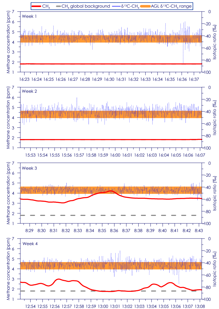
Figure C - 98: Time series of CH 4 concentration and isotopic ratio for Site 17 Weeks 1 - 4
