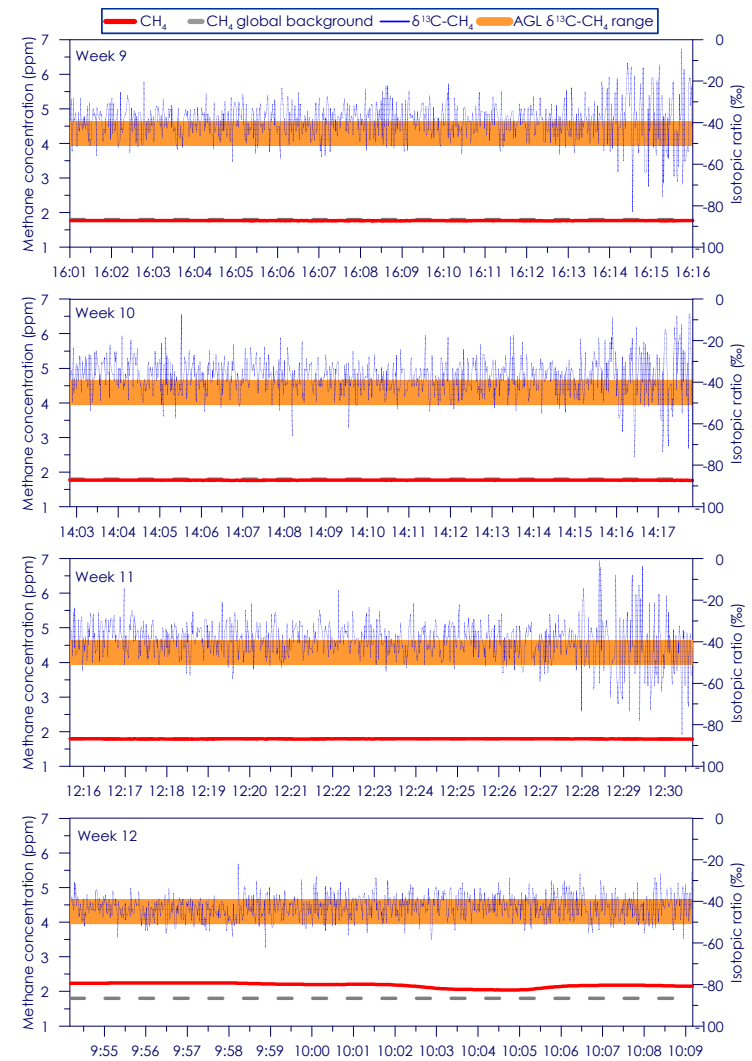
Figure C - 30: Time series of CH 4 concentration and isotopic ratio for Site 5 Weeks 9 - 12
