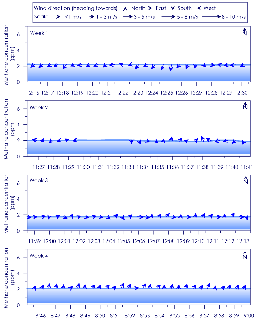
Figure C - 79: Time series of CH 4 concentration, wind speed and wind direction for Site 14 Weeks 1 - 4
