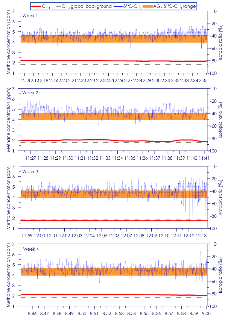
Figure C - 80: Time series of CH 4 concentration and isotopic ratio for Site 14 Weeks 1 - 4
