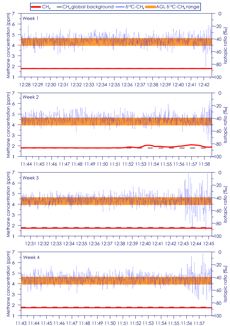
Figure C - 68: Time series of CH 4 concentration and isotopic ratio for Site 12 Weeks 1 - 4
