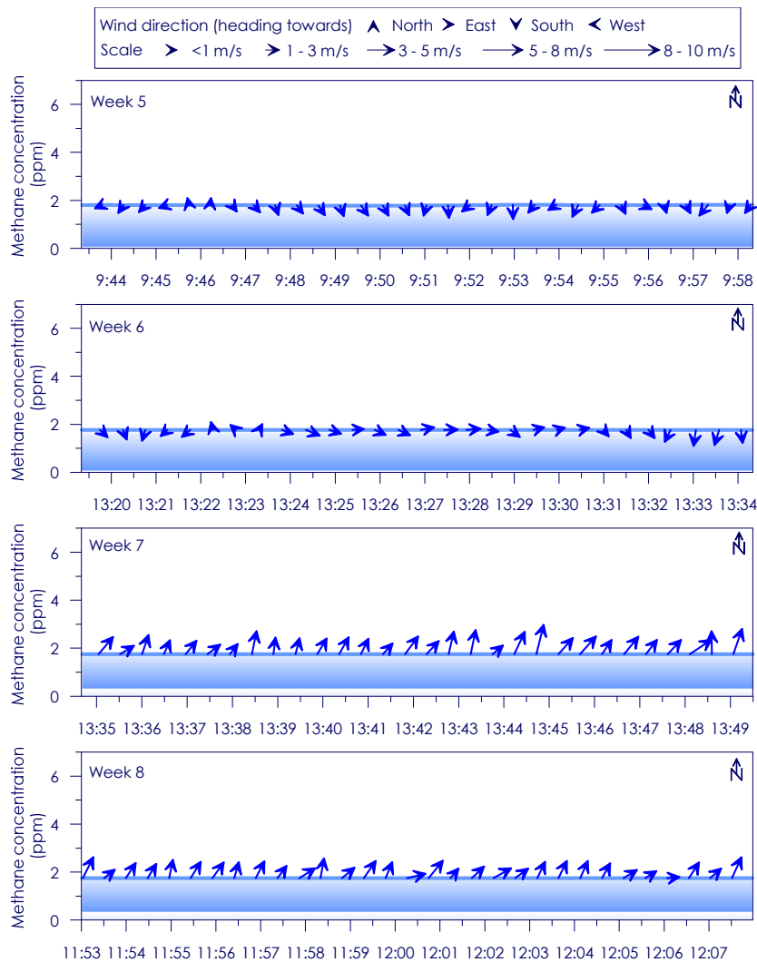
Figure C - 27: Time series of CH 4 concentration, wind speed and wind direction for Site 5 Weeks 5- 8
