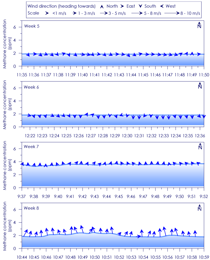
Figure C - 57: Time series of CH 4 concentration, wind speed and wind direction for Site 10 Weeks 5- 8
