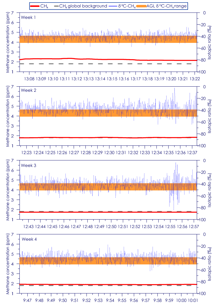
Figure C - 92: Time series of CH 4 concentration and isotopic ratio for Site 16 Weeks 1 - 4
