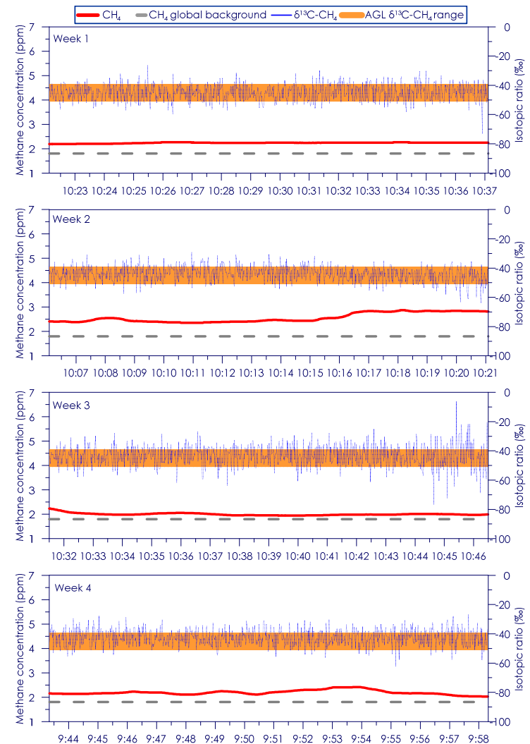
Figure C - 50: Time series of CH 4 concentration and isotopic ratio for Site 9 Weeks 1 - 4
