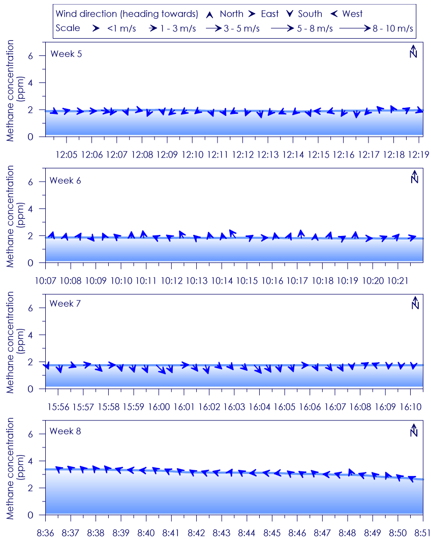
Figure C - 111: Time series of CH 4 concentration, wind speed and wind direction for Site 19 Weeks 5 - 8
