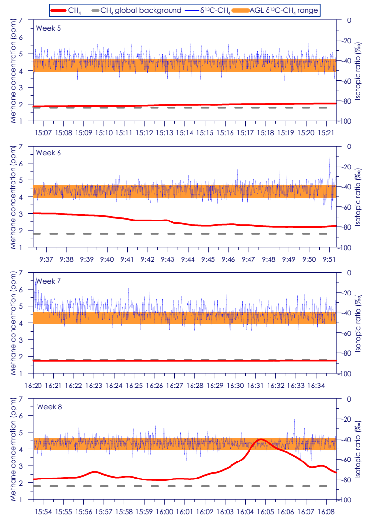
Figure C - 100: Time series of CH 4 concentration and isotopic ratio for Site 17 Weeks 5 - 8
