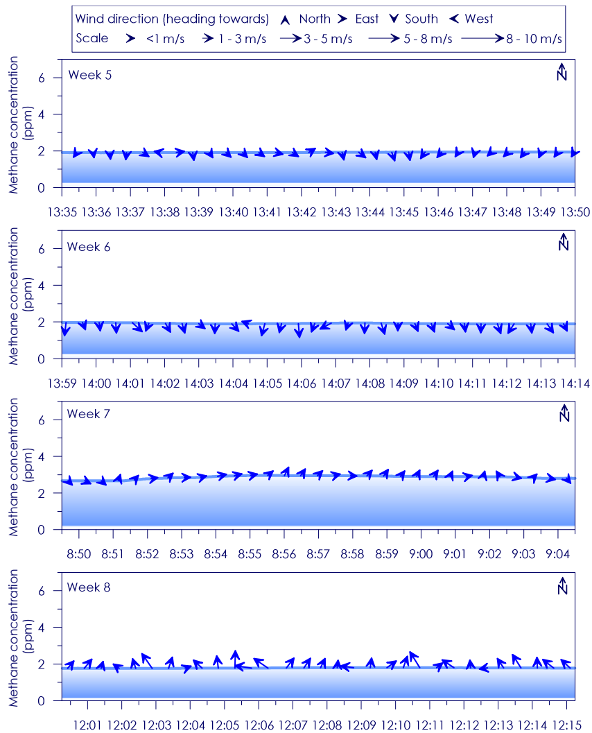
Figure C - 135: Time series of CH 4 concentration, wind speed and wind direction for Site 23 Weeks 5- 8
