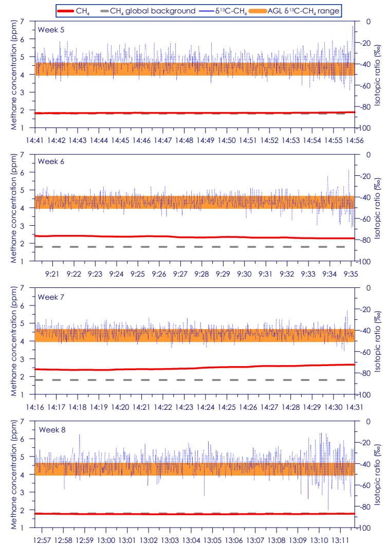
Figure C - 82: Time series of CH 4 concentration and isotopic ratio for Site 14 Weeks 5 - 8
