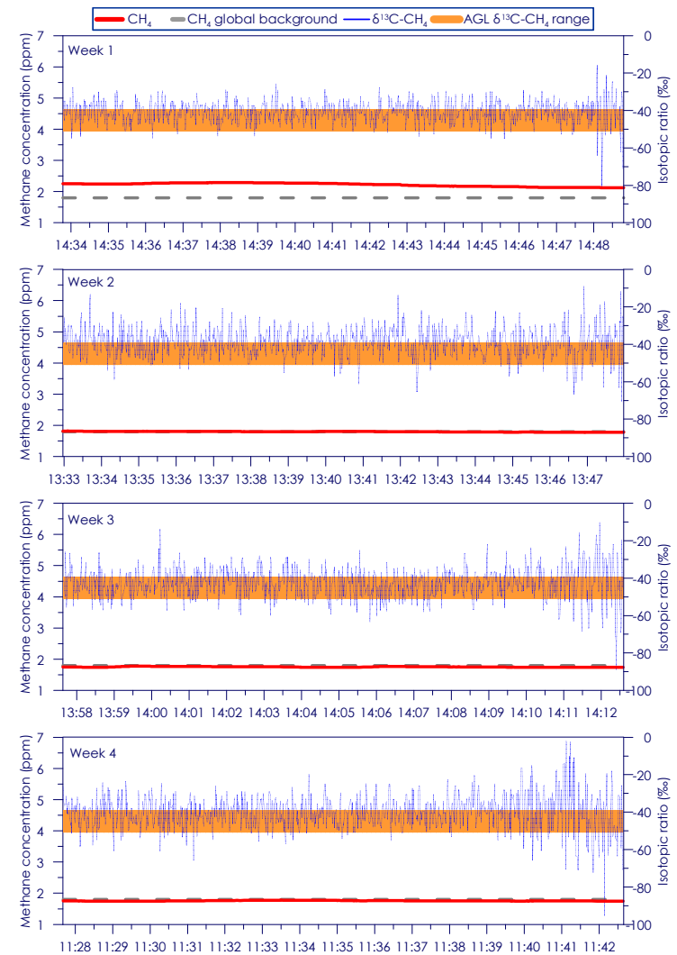
Figure C - 14: Time series of CH 4 concentration and isotopic ratio for Site 3 Weeks 1 - 4
