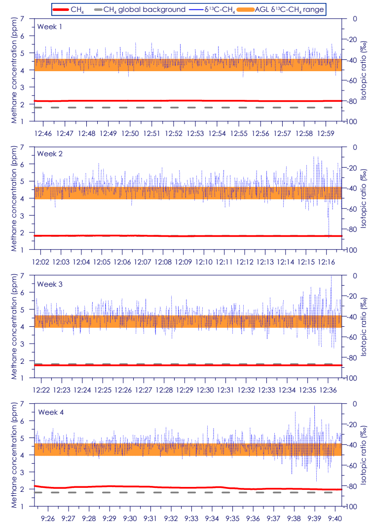
Figure C - 86: Time series of CH 4 concentration and isotopic ratio for Site 15 Weeks 1 - 4
