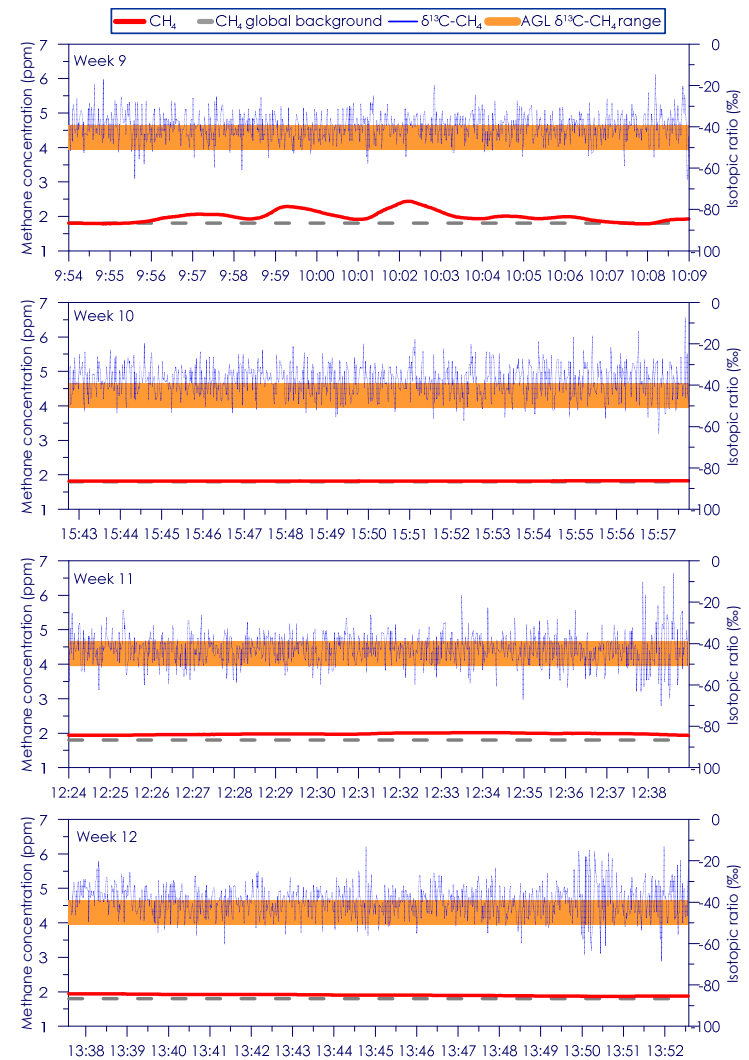
Figure C - 102: Time series of CH 4 concentration and isotopic ratio for Site 17 Weeks 9 - 12
