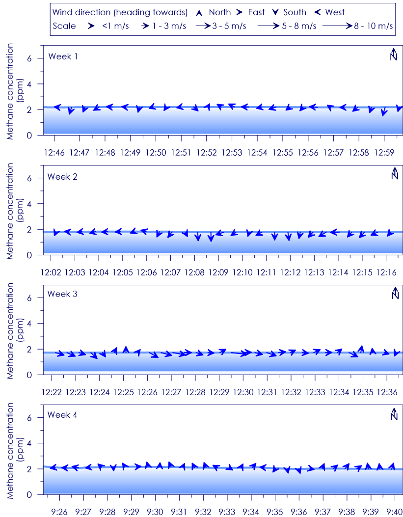
Figure C - 85: Time series of CH 4 concentration, wind speed and wind direction for Site 15 Weeks 1 - 4
