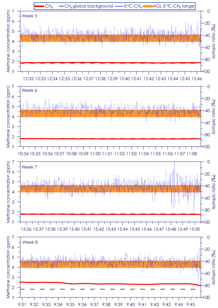
Figure C - 4: Time series of CH 4 concentration and isotopic ratio for Site 1 Weeks 5 - 8
