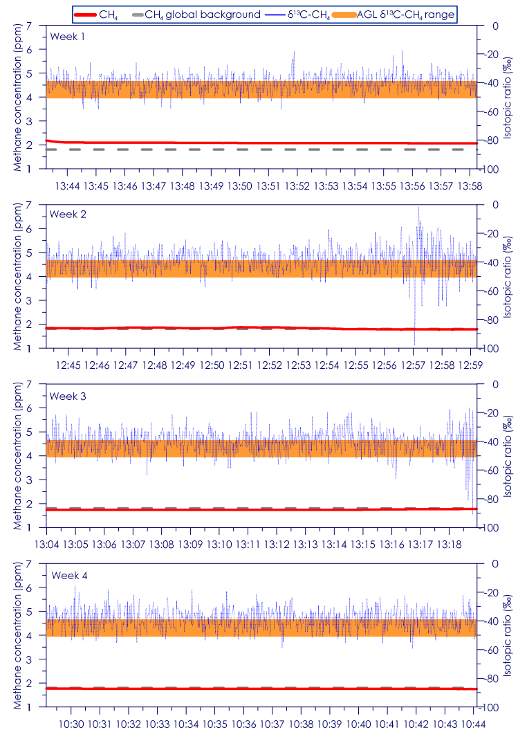
Figure C - 110: Time series of CH 4 concentration and isotopic ratio for Site 19 Weeks 1 - 4
