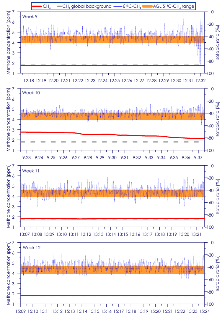
Figure C - 138: Time series of CH 4 concentration and isotopic ratio for Site 23 Weeks 9 - 12
