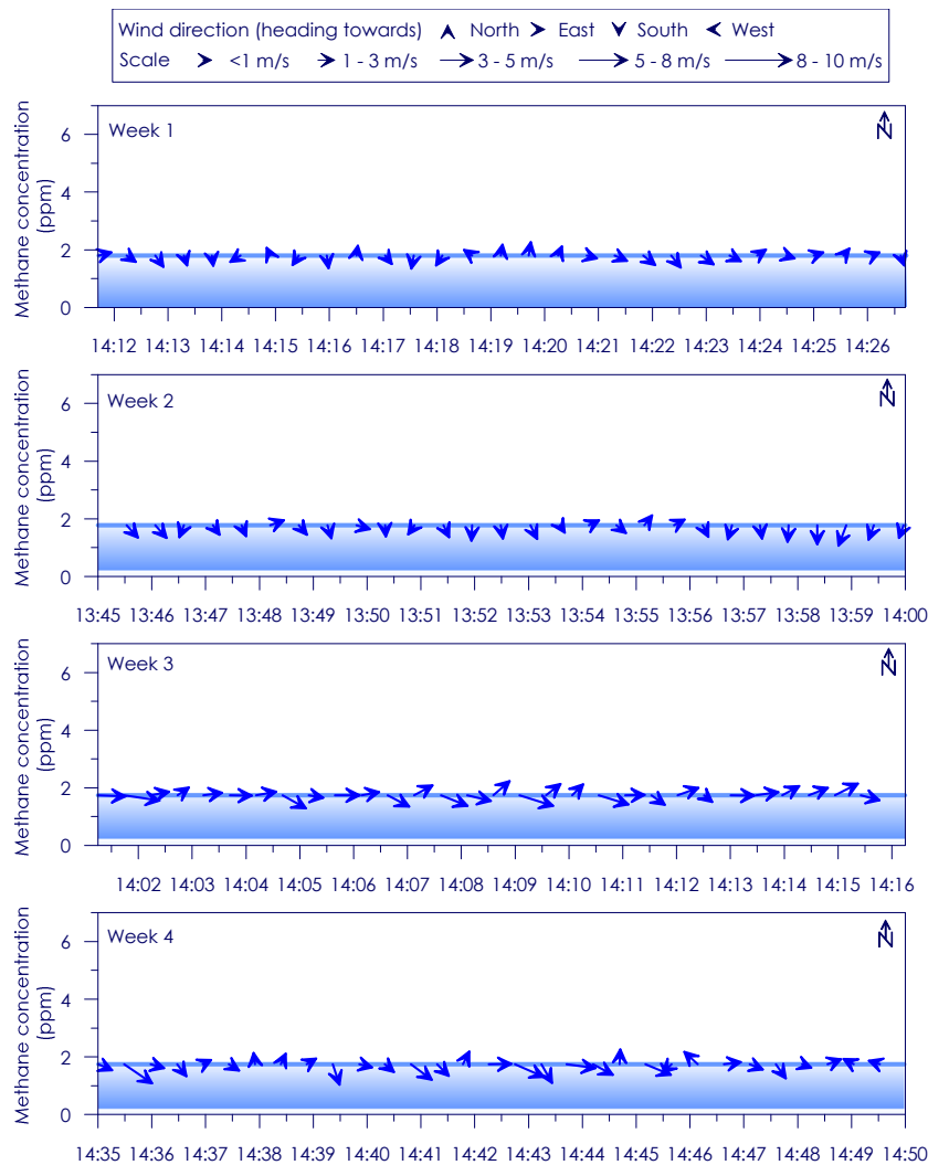
Figure C - 145: Time series of CH 4 concentration, wind speed and wind direction for Site 25 Weeks 1 - 4
