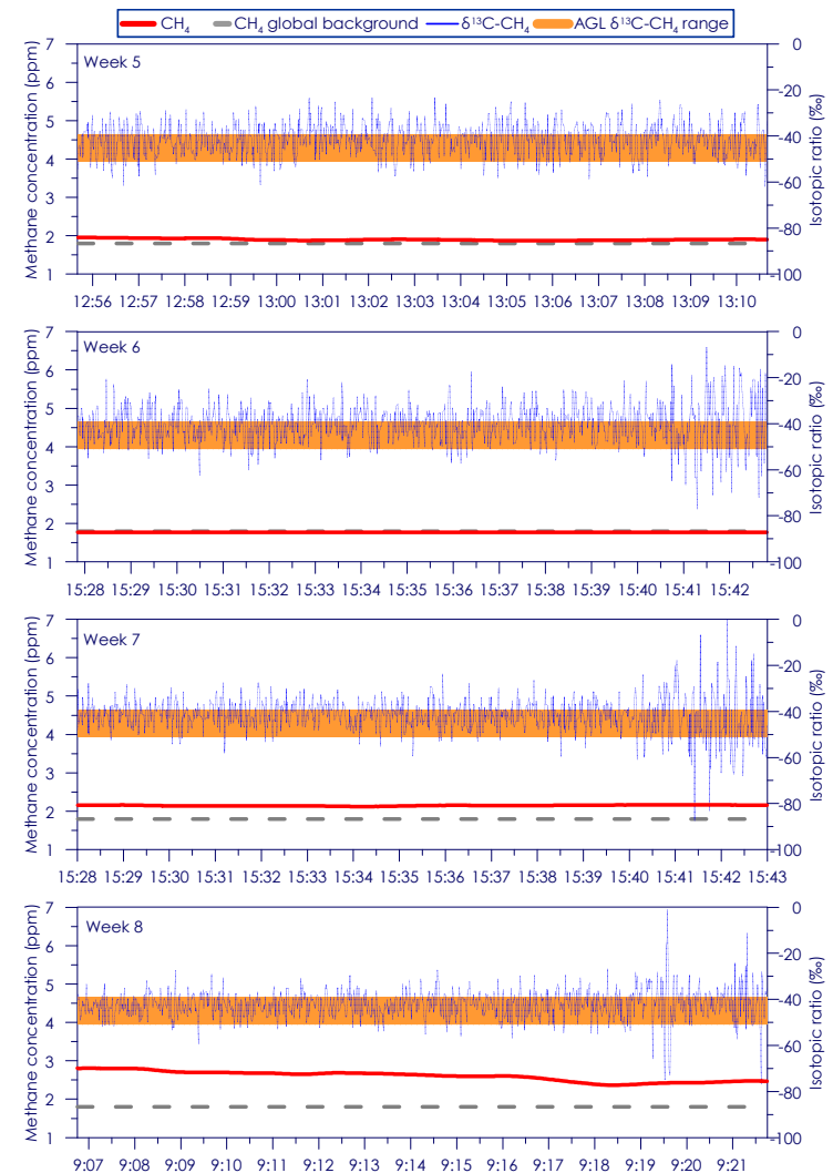
Figure C - 118: Time series of CH 4 concentration and isotopic ratio for Site 20 Weeks 5 - 8
