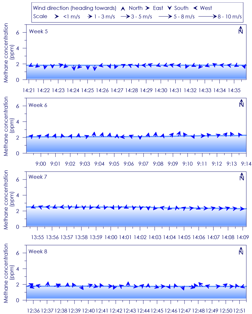
Figure C - 75: Time series of CH 4 concentration, wind speed and wind direction for Site 13 Weeks 5 - 8
