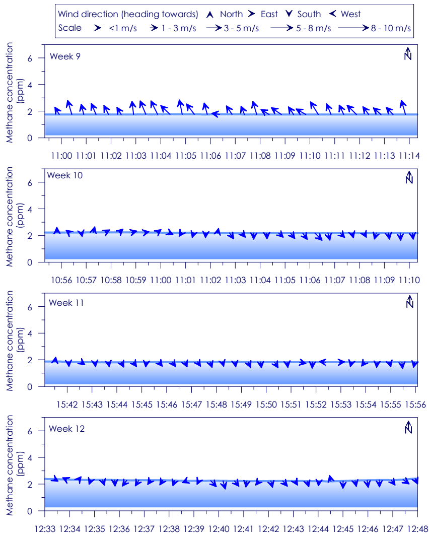
Figure C - 89: Time series of CH 4 concentration, wind speed and wind direction for Site 15 Weeks 9 - 12
