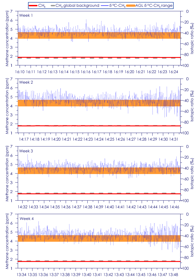
Figure C - 20: Time series of CH 4 concentration and isotopic ratio for Site 4 Weeks 1 - 4
