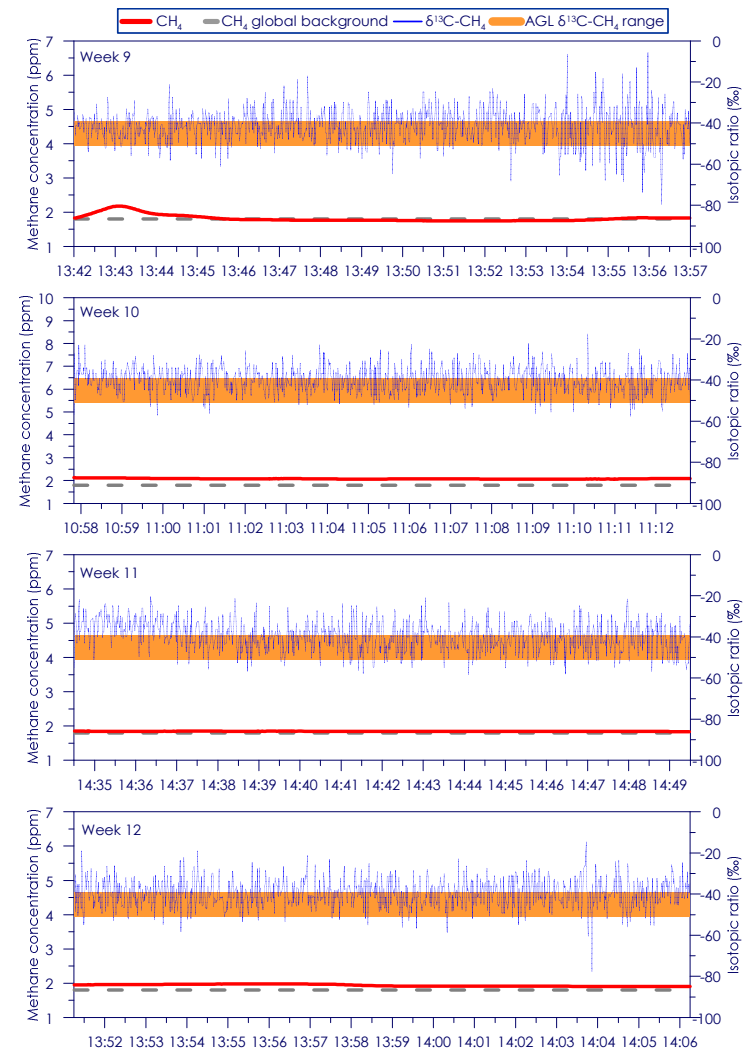
Figure C - 60: Time series of CH 4 concentration and isotopic ratio for Site 10 Weeks 9 - 12
