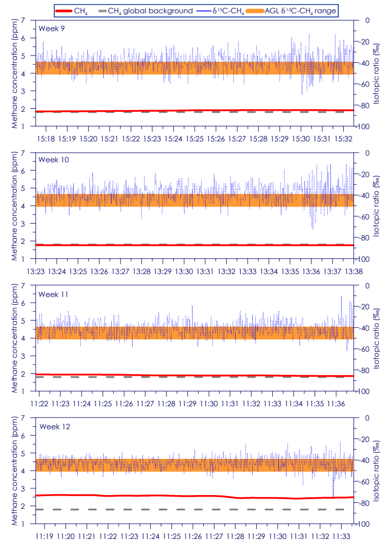
Figure C - 126: Time series of CH 4 concentration and isotopic ratio for Site 21 Weeks 9 - 12
