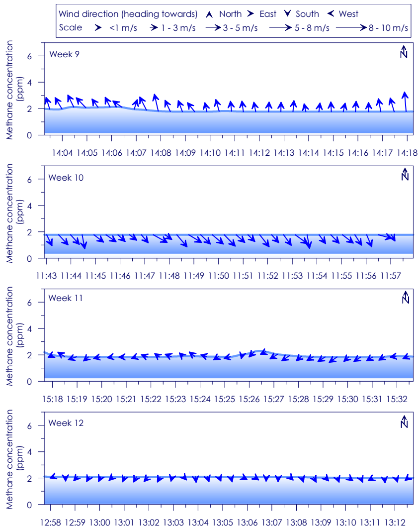
Figure C - 41: Time series of CH 4 concentration, wind speed and wind direction for Site 7 Weeks 9 - 12
