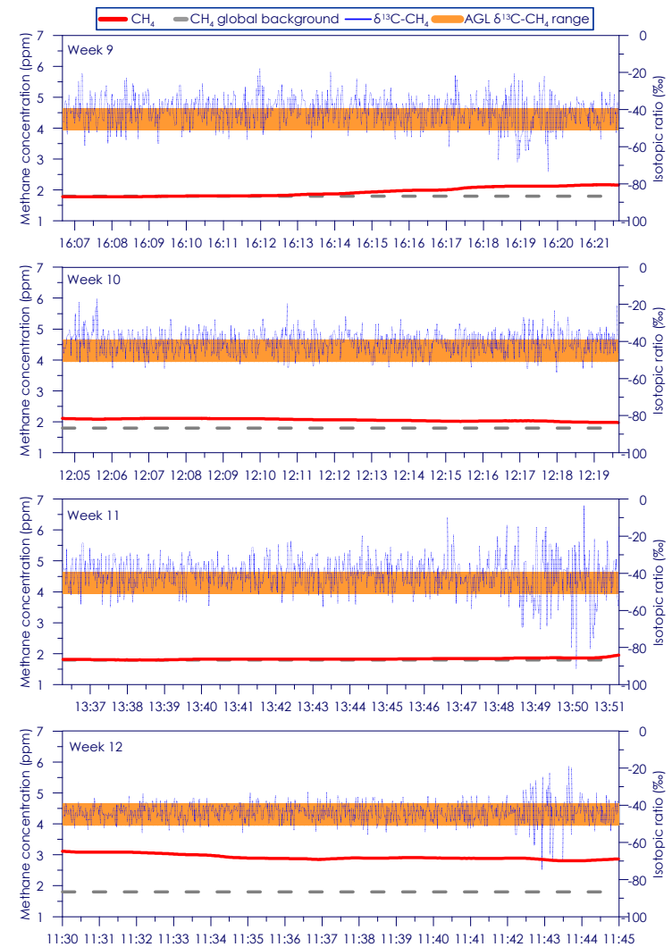
Figure C - 12: Time series of CH 4 concentration and isotopic ratio for Site 2 Weeks 9 - 12
