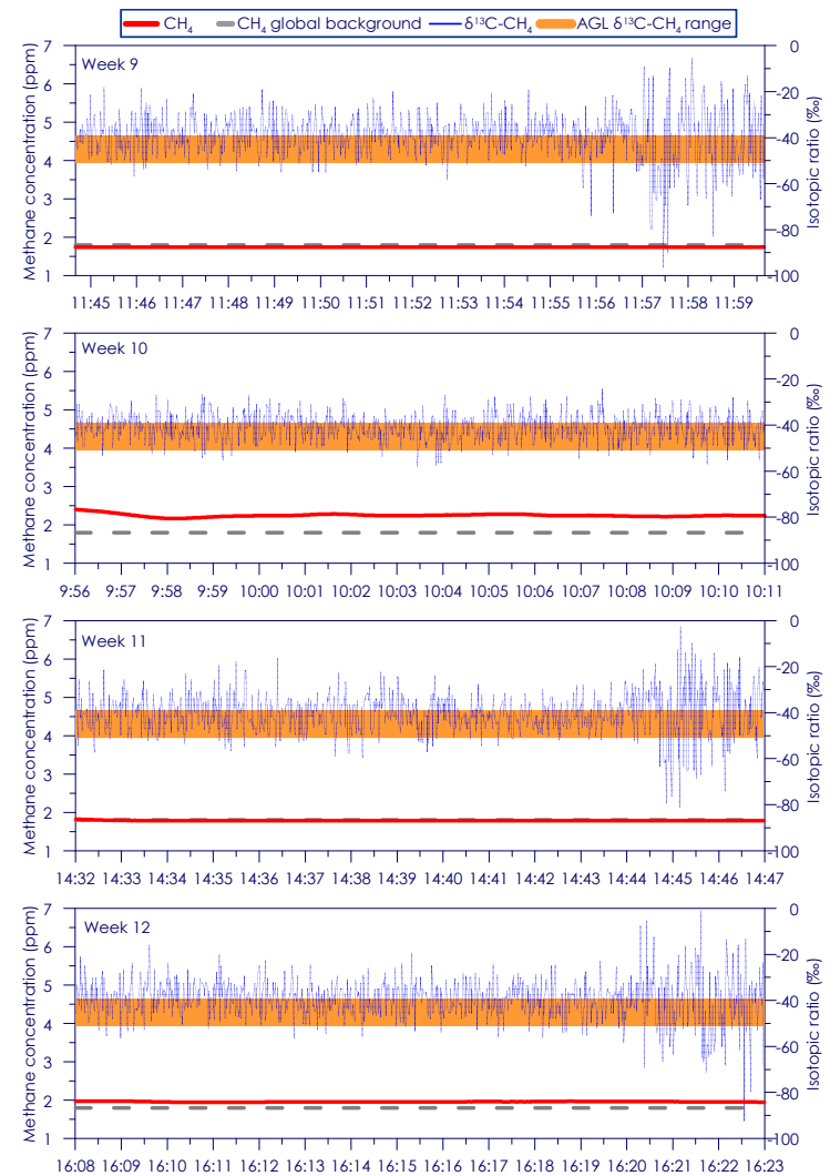
Figure C - 84: Time series of CH 4 concentration and isotopic ratio for Site 14 Weeks 9 - 12
