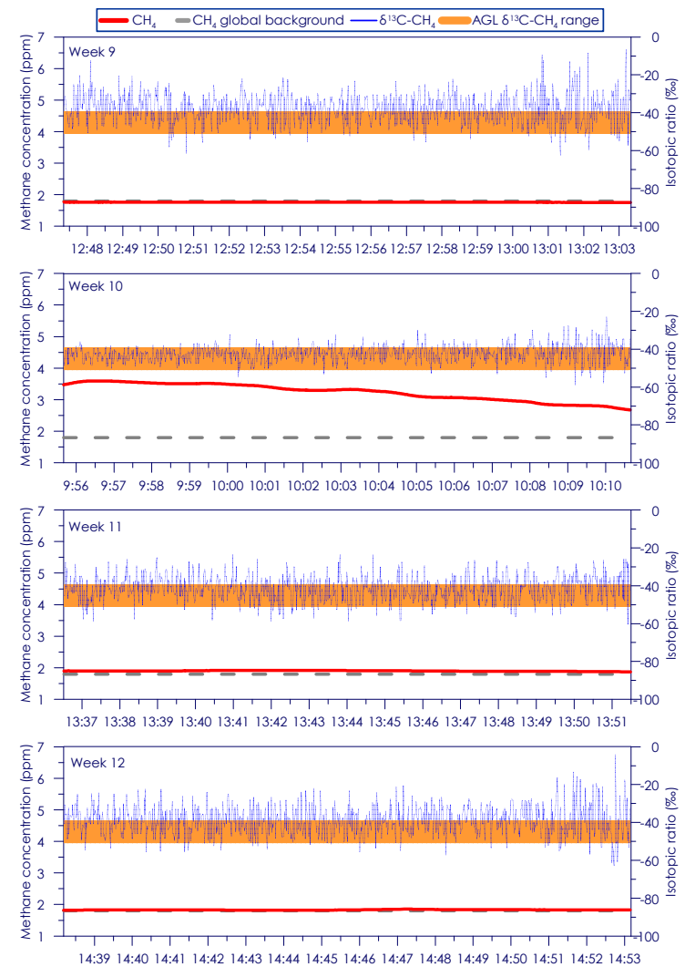
Figure C - 144: Time series of CH 4 concentration and isotopic ratio for Site 24 Weeks 9 - 12
