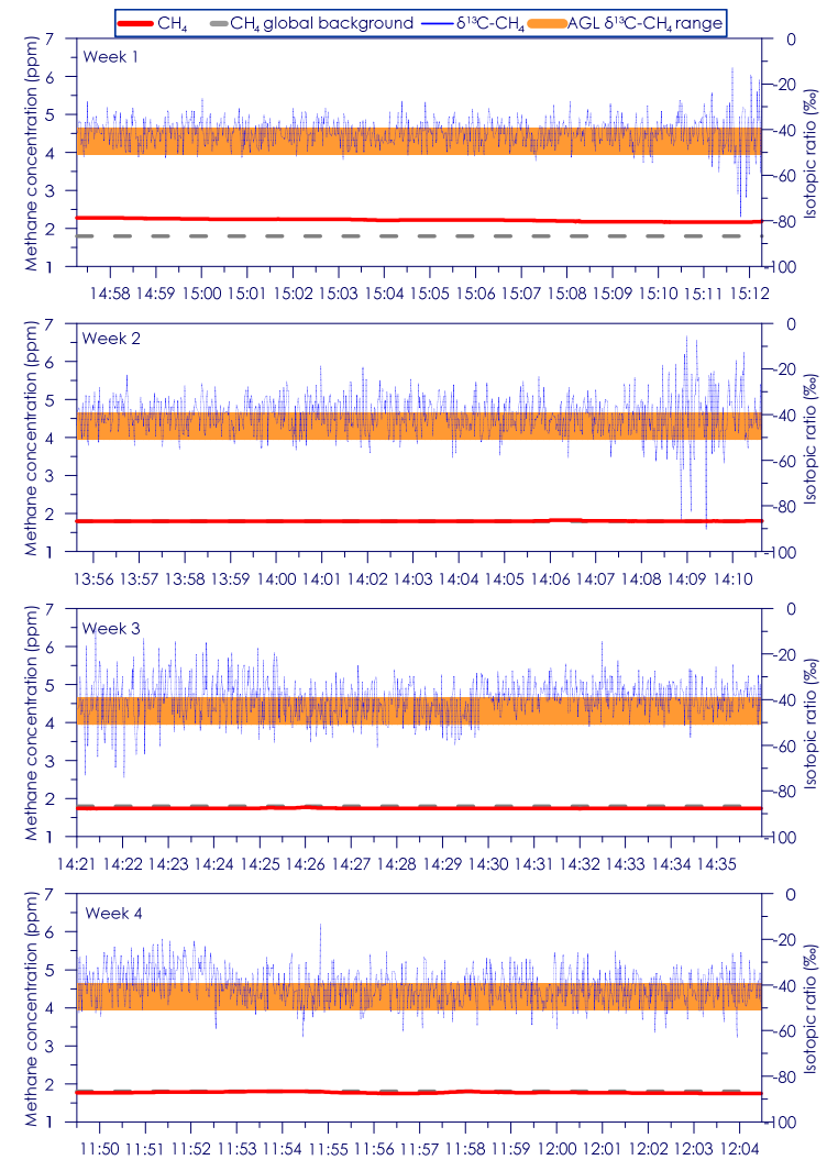
Figure C - 128: Time series of CH 4 concentration and isotopic ratio for Site 22 Weeks 1 - 4
