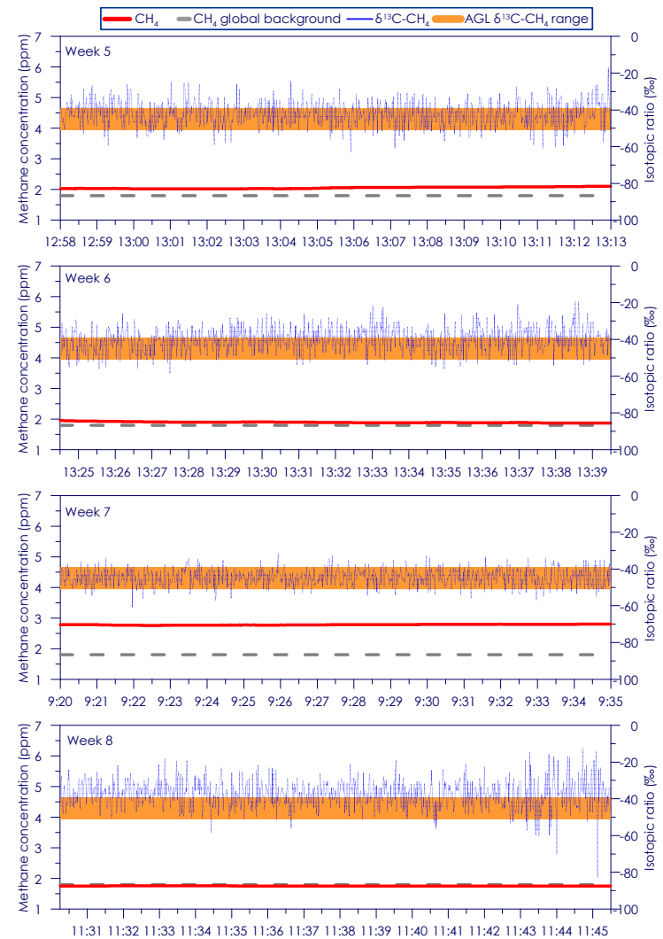
Figure C - 142: Time series of CH 4 concentration and isotopic ratio for Site 24 Weeks 5 - 8
