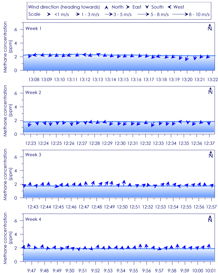
Figure C - 91: Time series of CH 4 concentration, wind speed and wind direction for Site 16 Weeks 1 - 4
