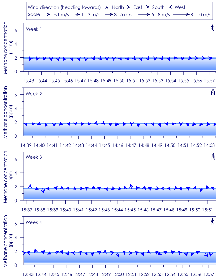
Figure C - 13: Time series of CH 4 concentration, wind speed and wind direction for Site 3 Weeks 1 - 4
