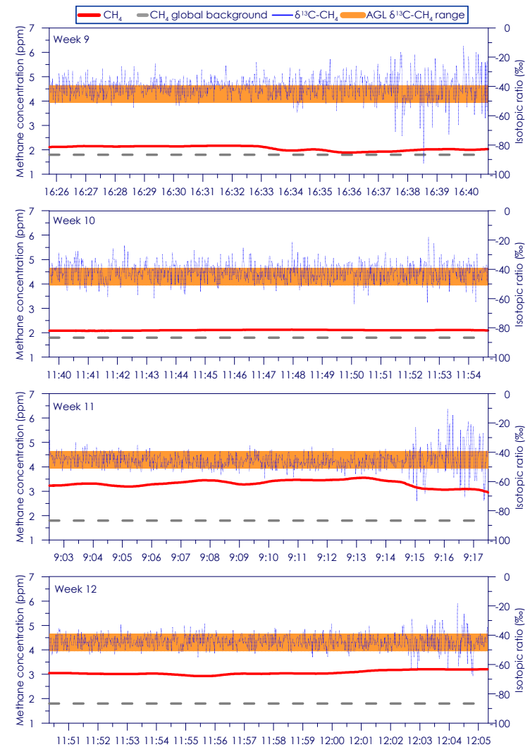
Figure C - 6: Time series of CH 4 concentration and isotopic ratio for Site 1 Weeks 9 - 12
