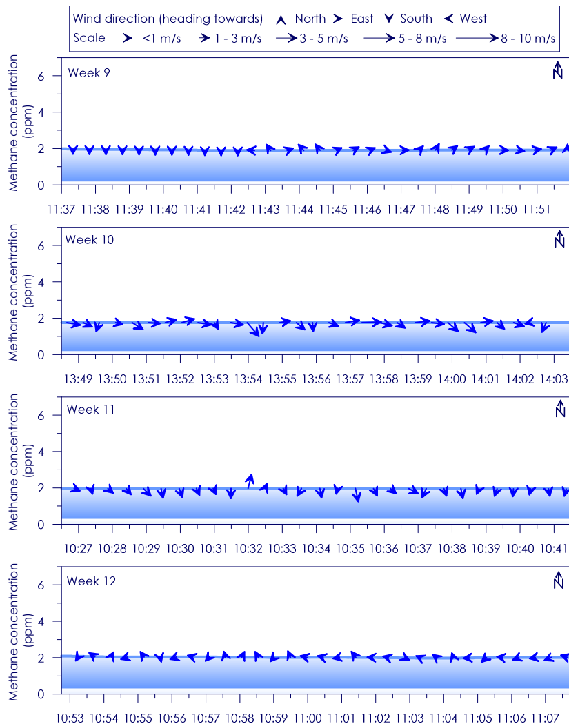
Figure C - 149: Time series of CH 4 concentration, wind speed and wind direction for Site 25 Weeks 9 - 12
