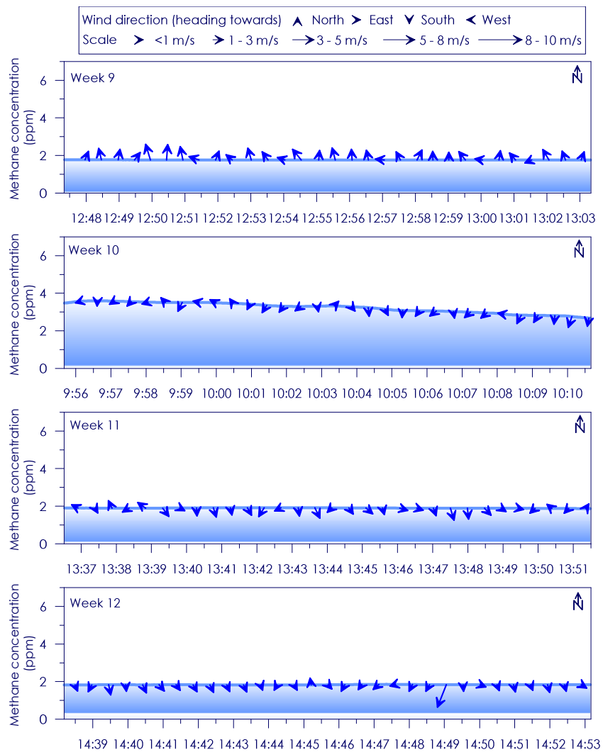
Figure C - 143: Time series of CH 4 concentration, wind speed and wind direction for Site 24 Weeks 9 - 12
