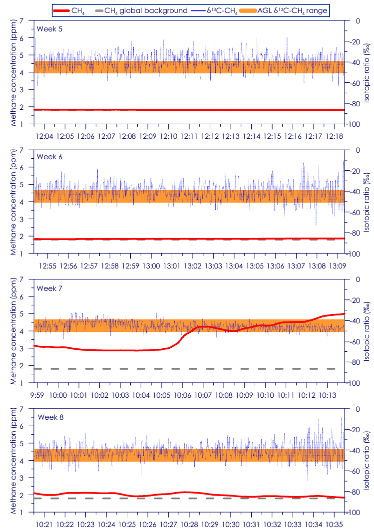
Figure C - 52: Time series of CH 4 concentration and isotopic ratio for Site 9 Weeks 5 - 8
