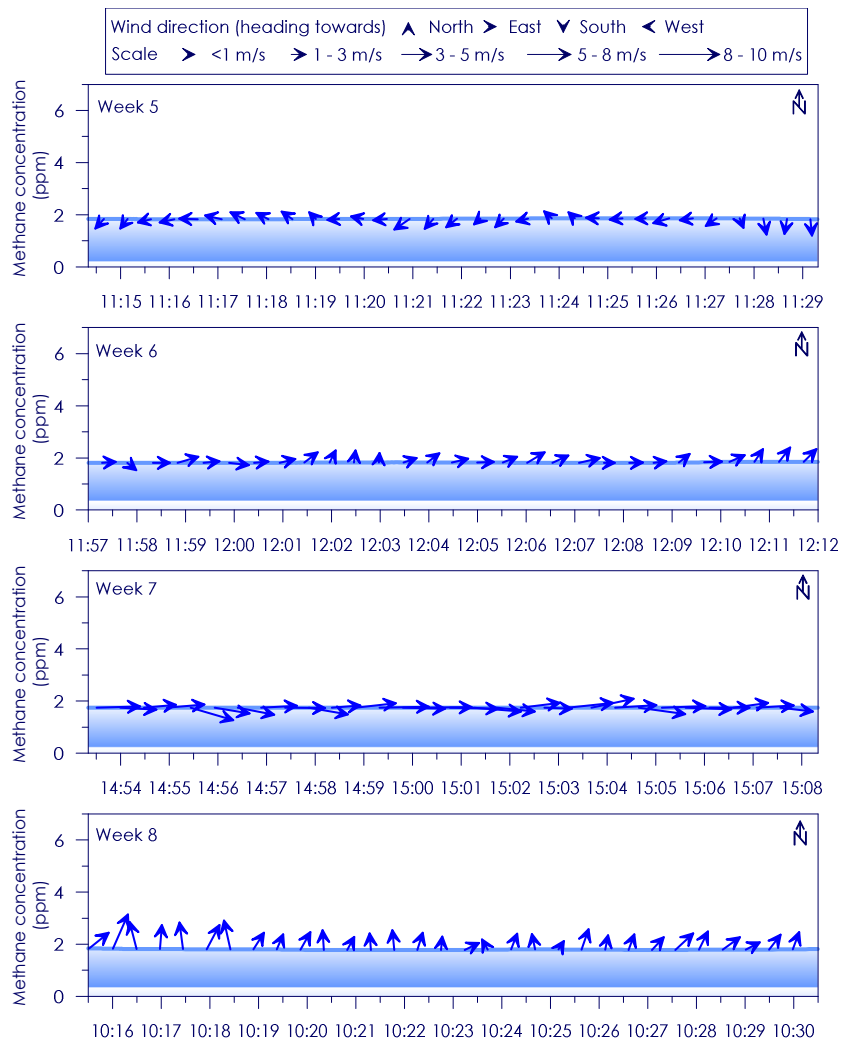
Figure C - 129: Time series of CH 4 concentration, wind speed and wind direction for Site 22 Weeks 5- 8
