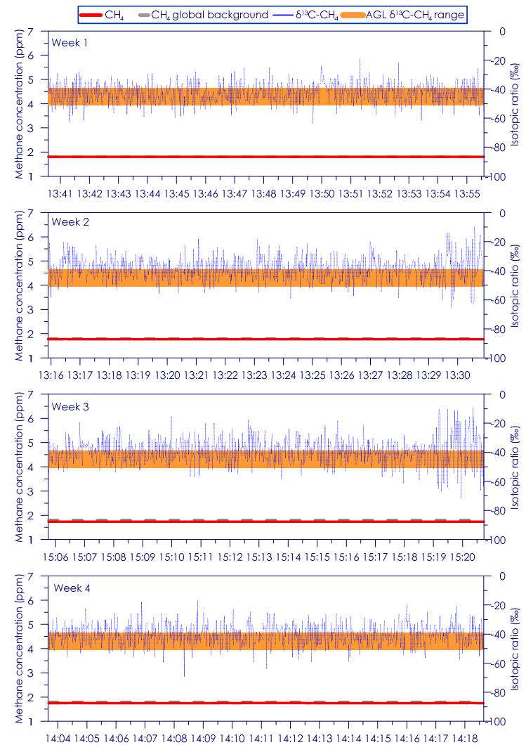
Figure C - 122: Time series of CH 4 concentration and isotopic ratio for Site 21 Weeks 1 - 4
