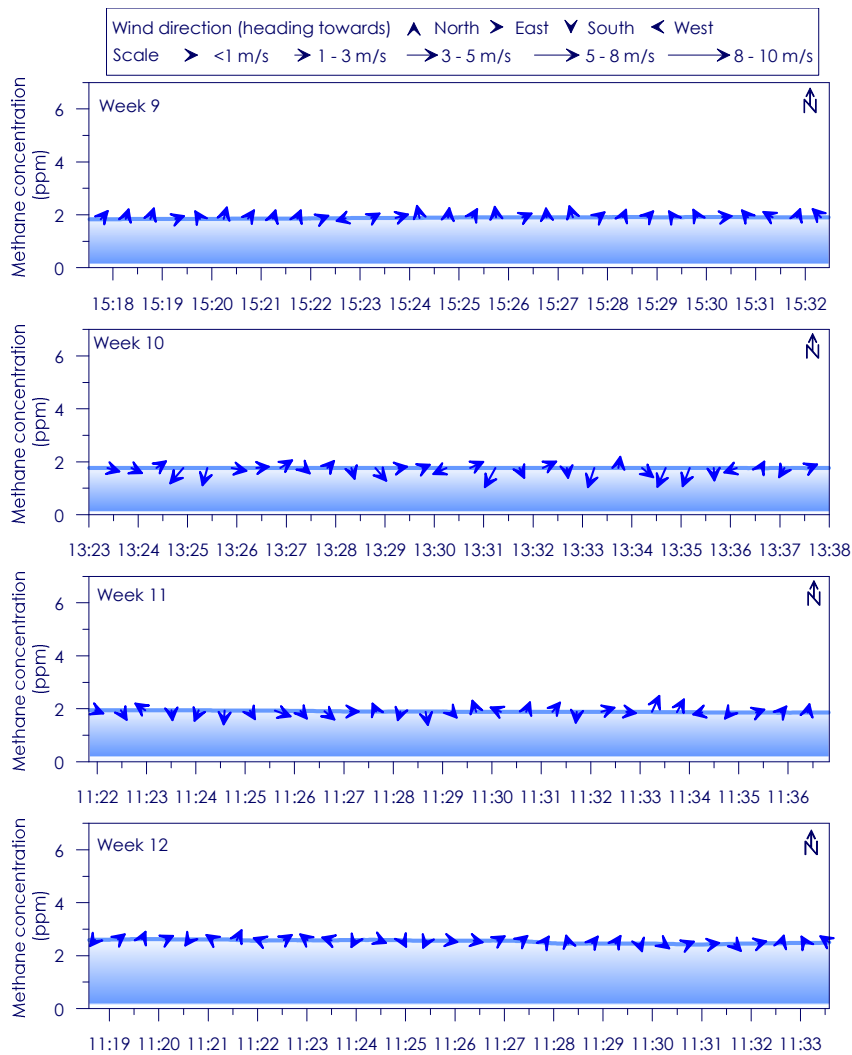
Figure C - 125: Time series of CH 4 concentration, wind speed and wind direction for Site 21 Weeks 9 - 12
