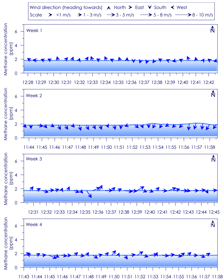
Figure C - 67: Time series of CH 4 concentration, wind speed and wind direction for Site 12 Weeks 1 - 4
