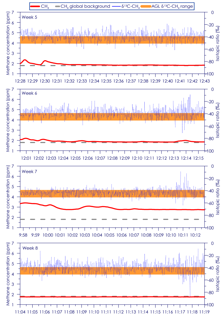
Figure C - 46: Time series of CH 4 concentration and isotopic ratio for Site 8 Weeks 5 - 8
