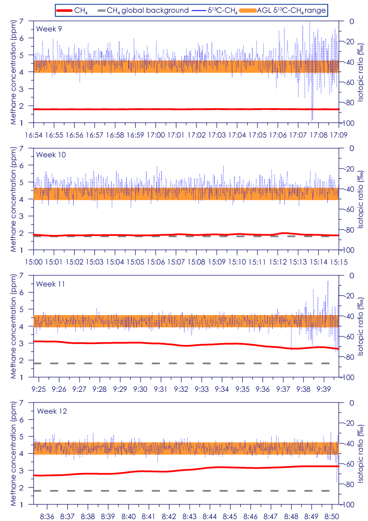
Figure C - 120: Time series of CH 4 concentration and isotopic ratio for Site 20 Weeks 9 - 12
