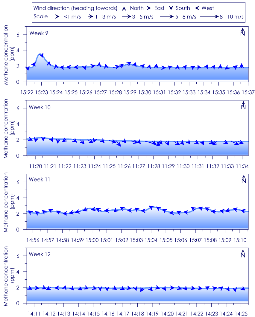
Figure C - 47: Time series of CH 4 concentration, wind speed and wind direction for Site 8 Weeks 9 - 12
