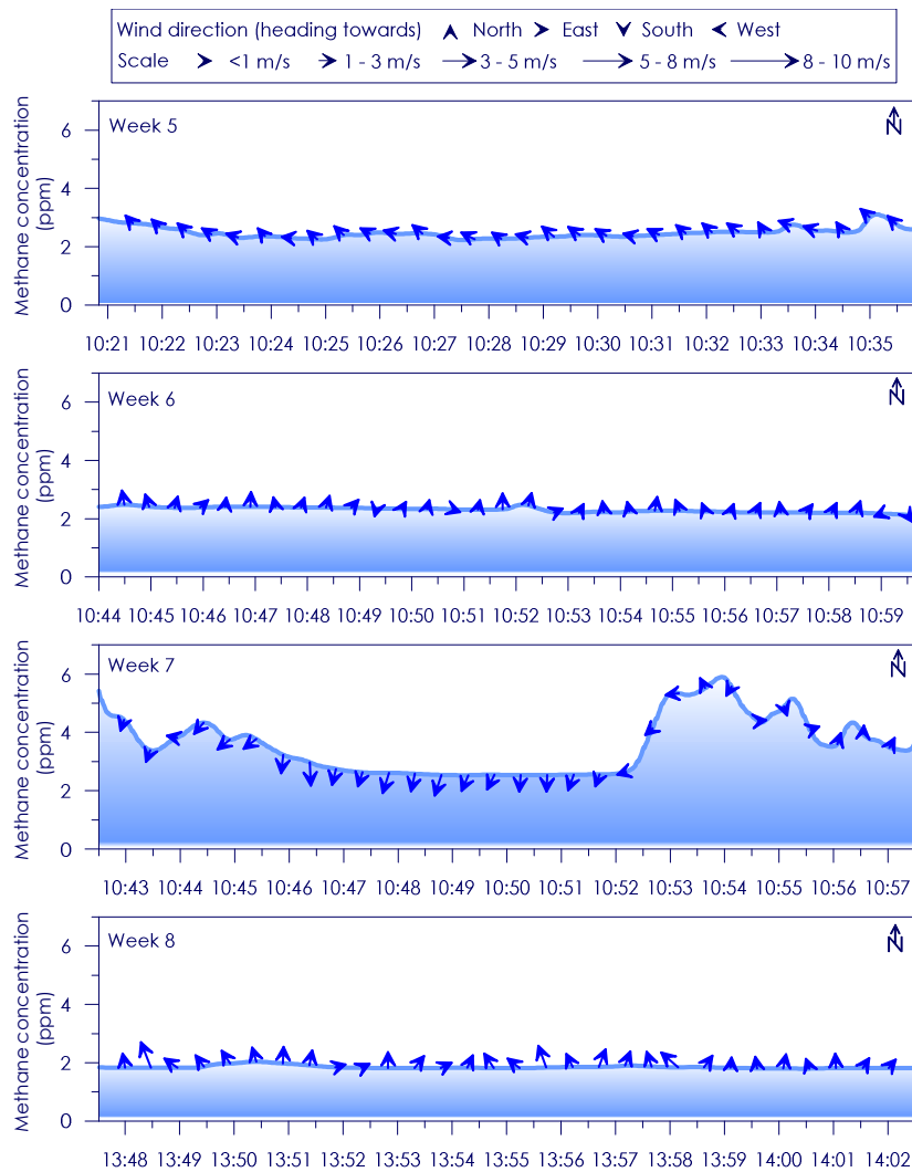
Figure C - 63: Time series of CH 4 concentration, wind speed and wind direction for Site 11 Weeks 5- 8
