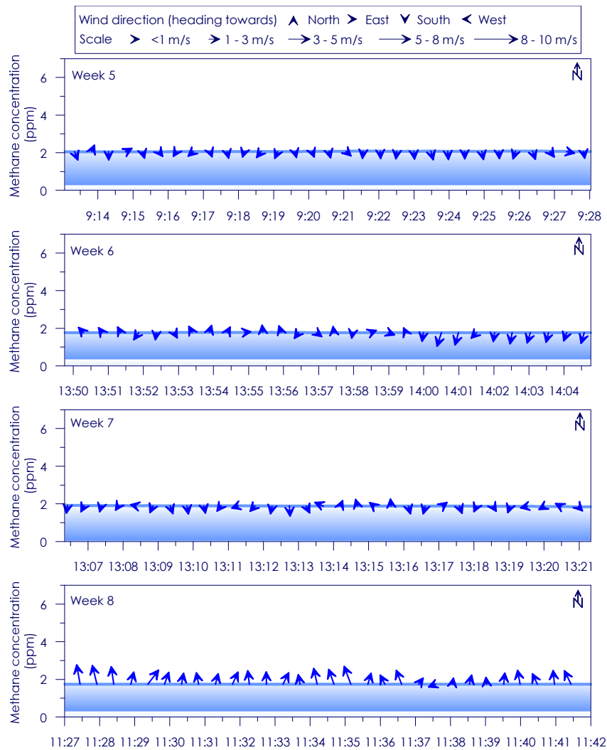
Figure C - 21: Time series of CH 4 concentration, wind speed and wind direction for Site 4 Weeks 5 - 8
