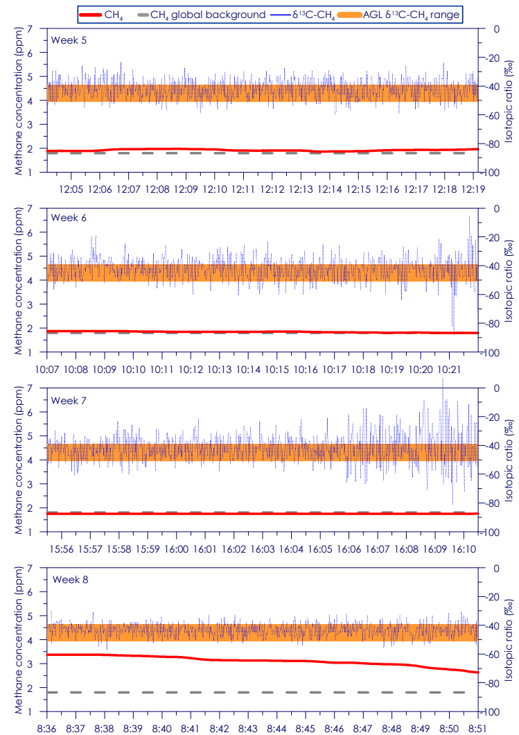
Figure C - 112: Time series of CH 4 concentration and isotopic ratio for Site 19 Weeks 5 - 8
