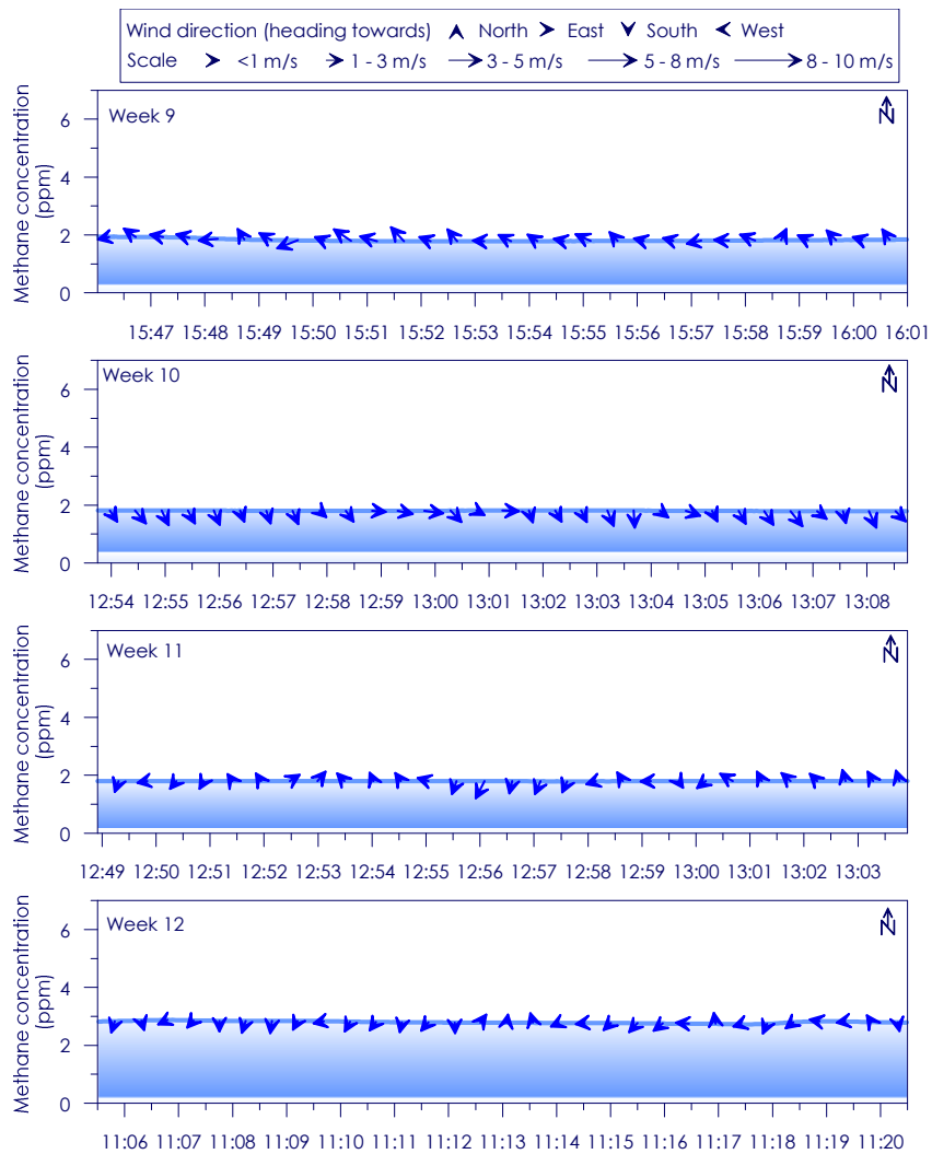
Figure C - 107: Time series of CH 4 concentration, wind speed and wind direction for Site 18 Weeks 9 - 12
