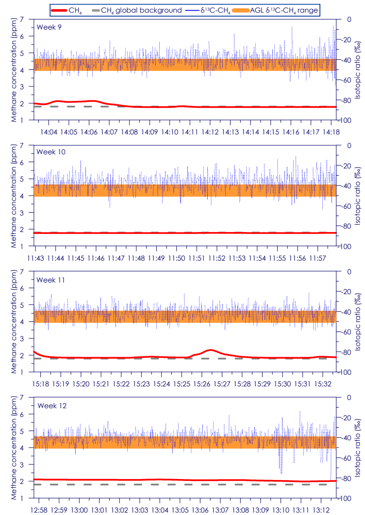
Figure C - 42: Time series of CH 4 concentration and isotopic ratio for Site 7 Weeks 9 - 12
