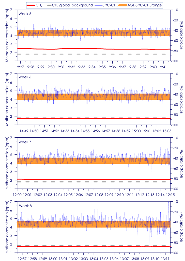
Figure C - 124: Time series of CH 4 concentration and isotopic ratio for Site 21 Weeks 5 - 8
