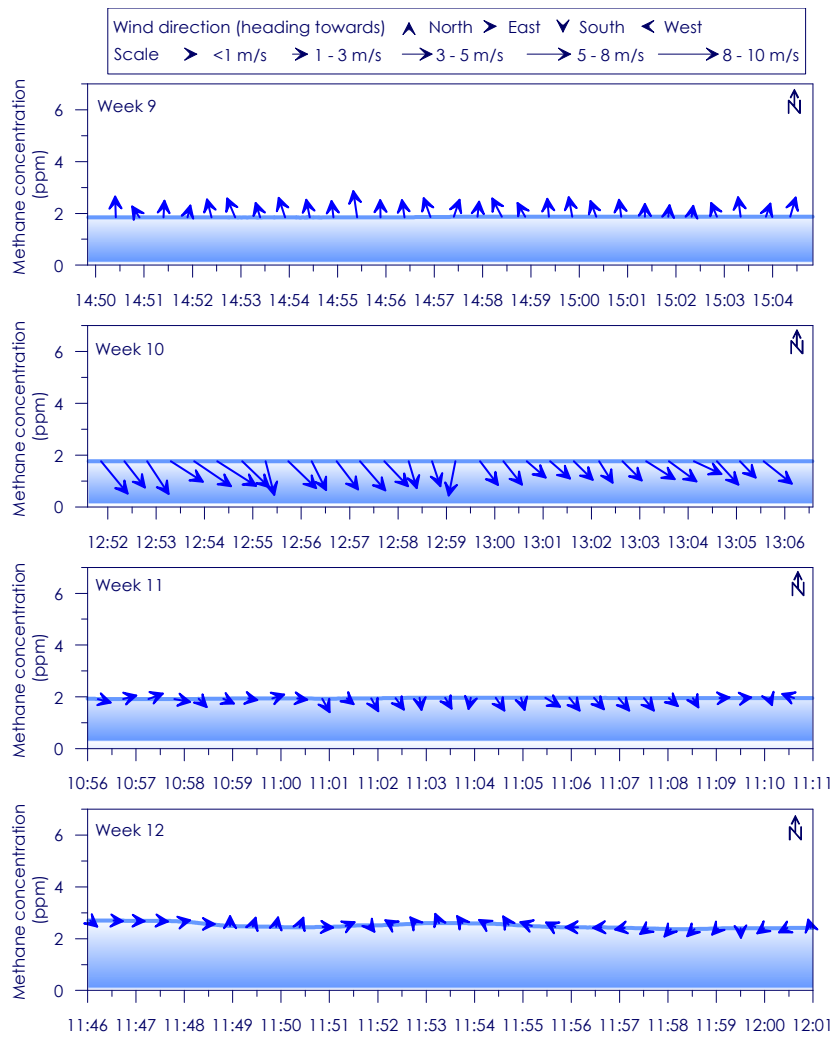
Figure C - 35: Time series of CH 4 concentration, wind speed and wind direction for Site 6 Weeks 9 - 12
