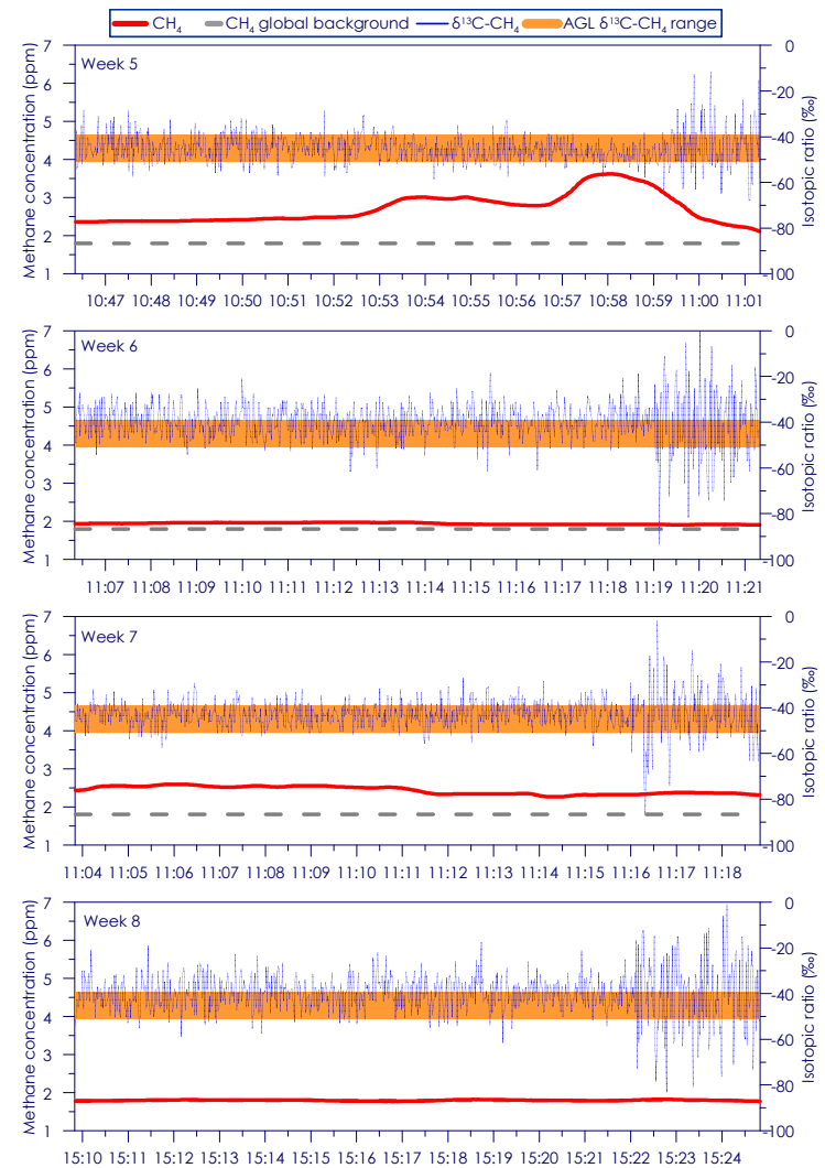
Figure C - 70: Time series of CH 4 concentration and isotopic ratio for Site 12 Weeks 5 - 8
