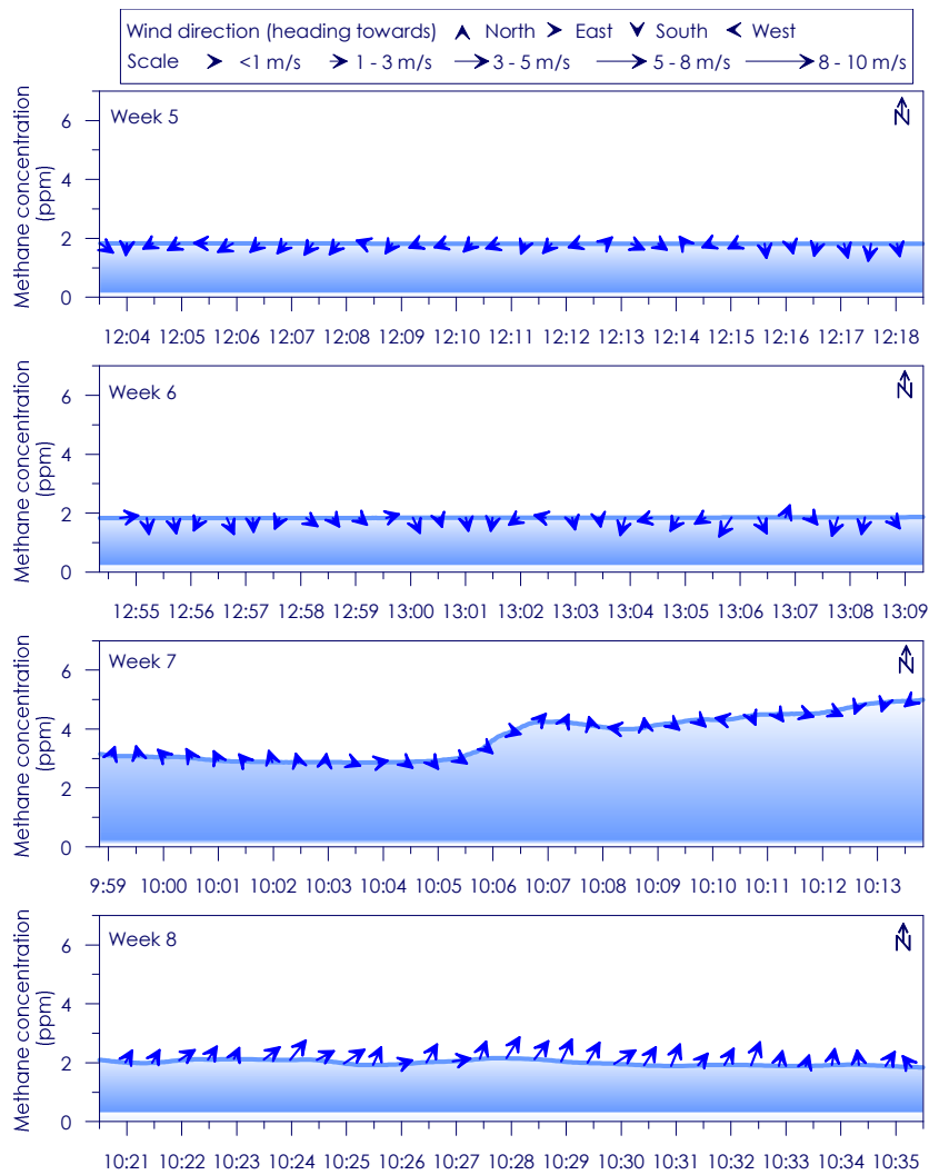
Figure C - 51: Time series of CH 4 concentration, wind speed and wind direction for Site 9 Weeks 5- 8
