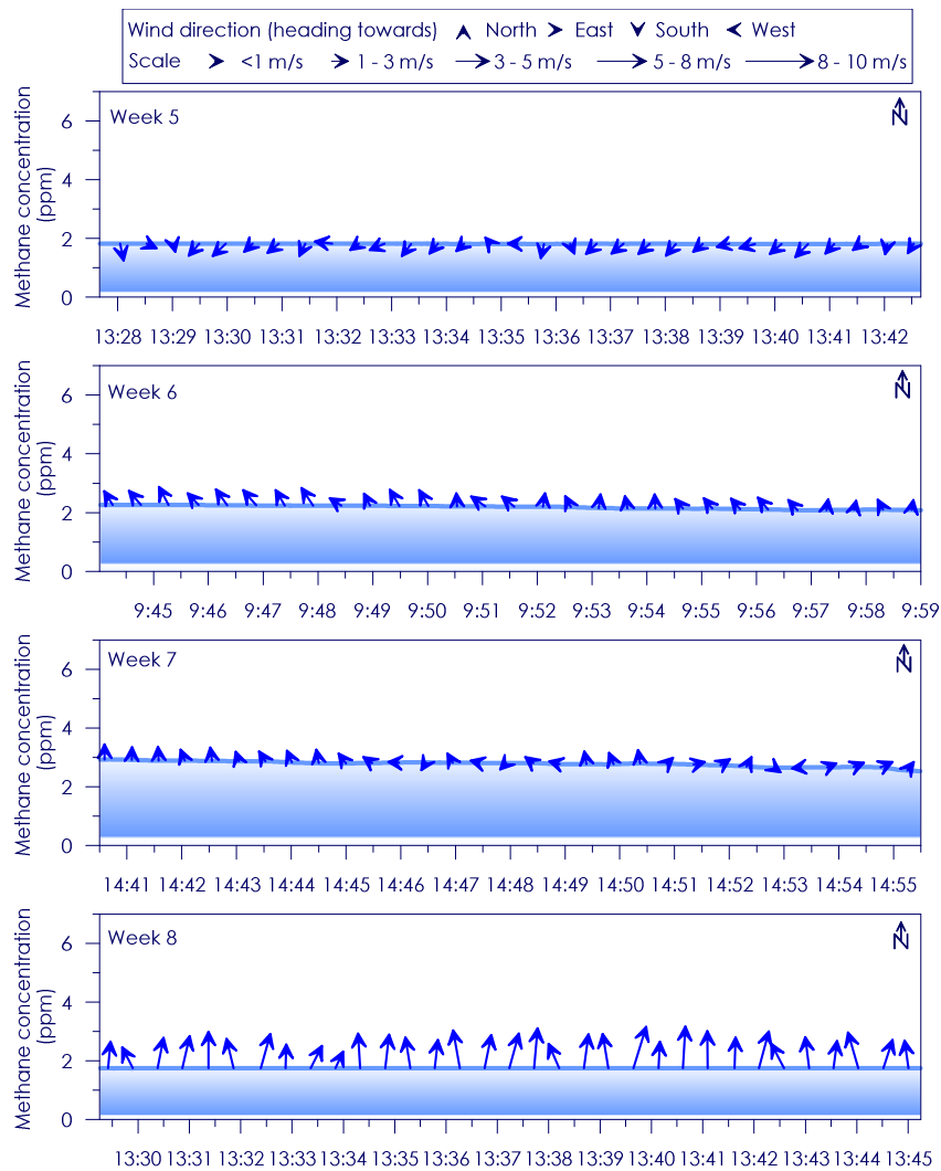
Figure C - 87: Time series of CH 4 concentration, wind speed and wind direction for Site 15 Weeks 5 - 8
