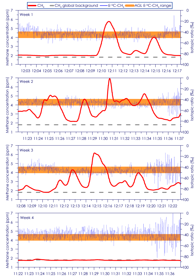
Figure C - 62: Time series of CH 4 concentration and isotopic ratio for Site 11 Weeks 1 - 4
