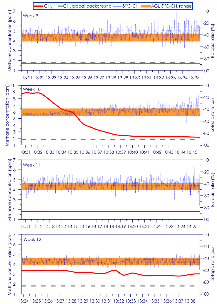
Figure C - 54: Time series of CH 4 concentration and isotopic ratio for Site 9 Weeks 9 - 12
