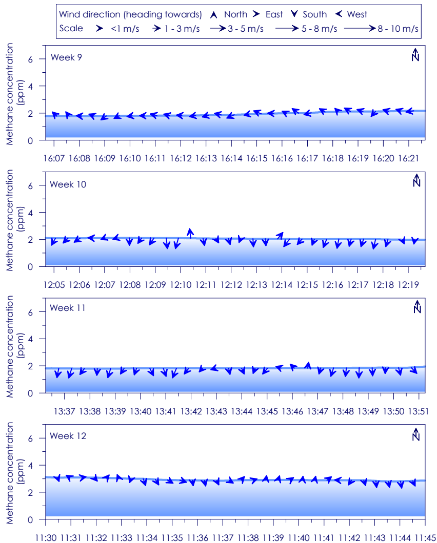
Figure C - 11: Time series of CH 4 concentration, wind speed and wind direction for Site 2 Weeks 9 - 12
