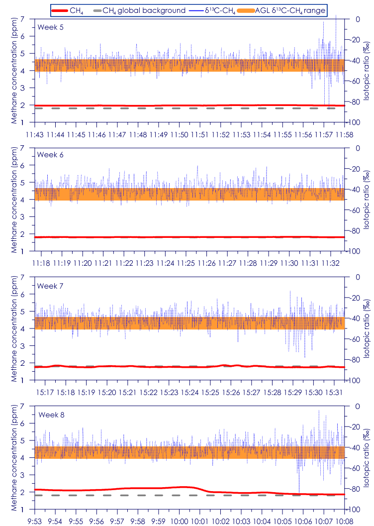
Figure C - 10: Time series of CH 4 concentration and isotopic ratio for Site 2 Weeks 5 - 8
