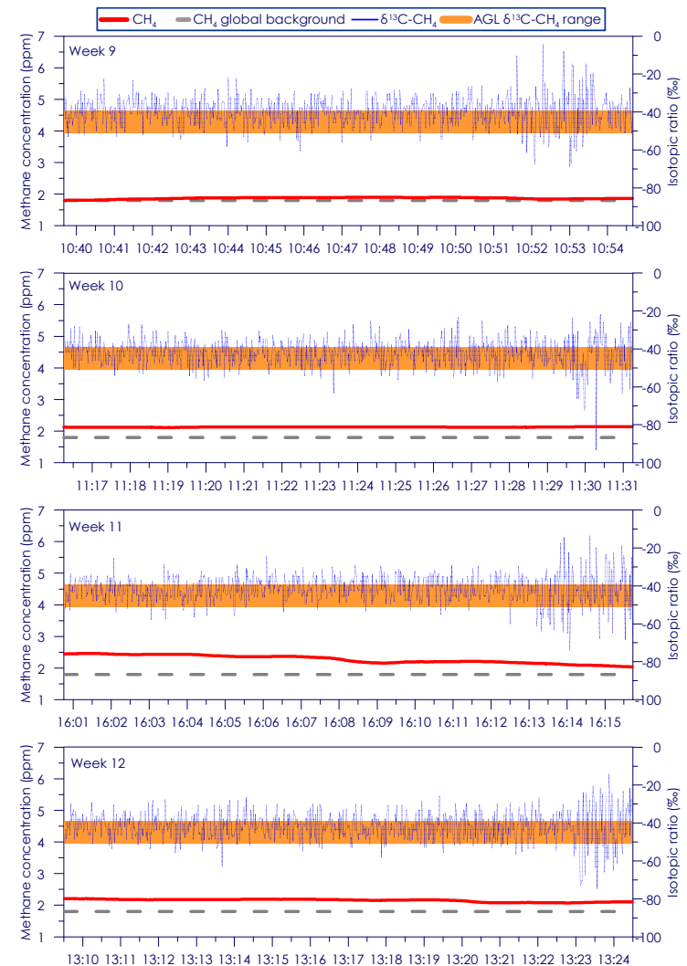
Figure C - 96: Time series of CH 4 concentration and isotopic ratio for Site 16 Weeks 9 - 12
