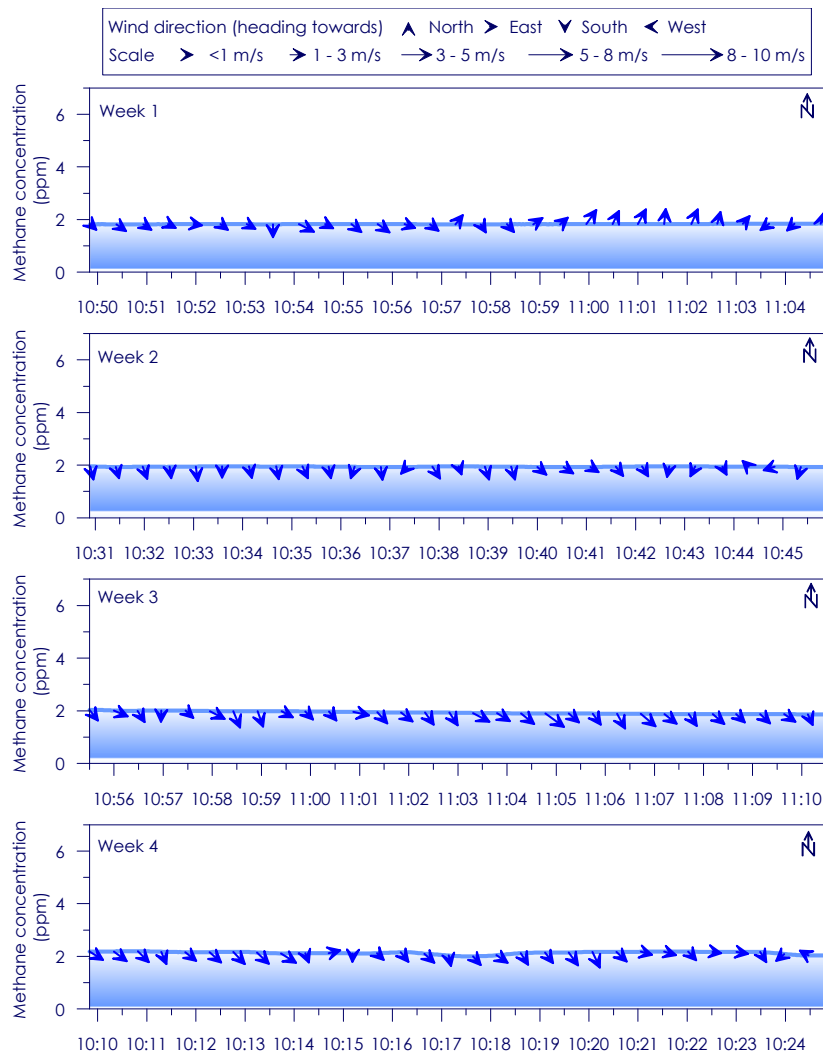
Figure C - 55: Time series of CH 4 concentration, wind speed and wind direction for Site 10 Weeks 1 - 4
