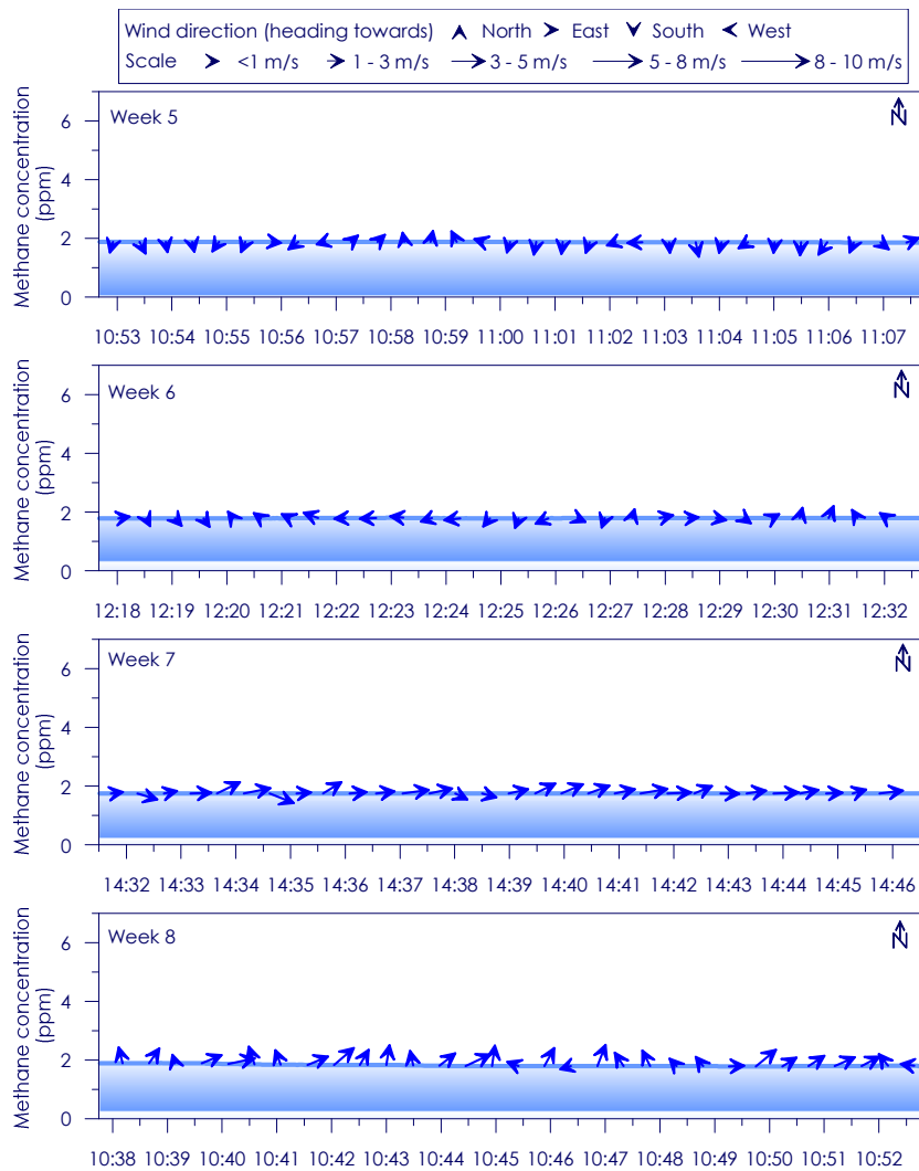
Figure C - 105: Time series of CH 4 concentration, wind speed and wind direction for Site 18 Weeks 5- 8
