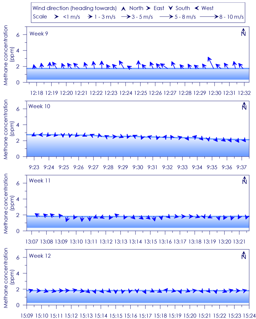
Figure C - 137: Time series of CH 4 concentration, wind speed and wind direction for Site 23 Weeks 9 - 12
