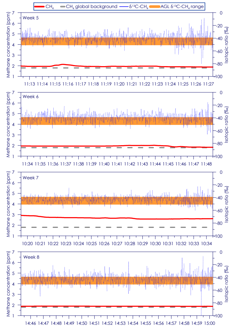
Figure C - 40: Time series of CH 4 concentration and isotopic ratio for Site 7 Weeks 5 - 8
