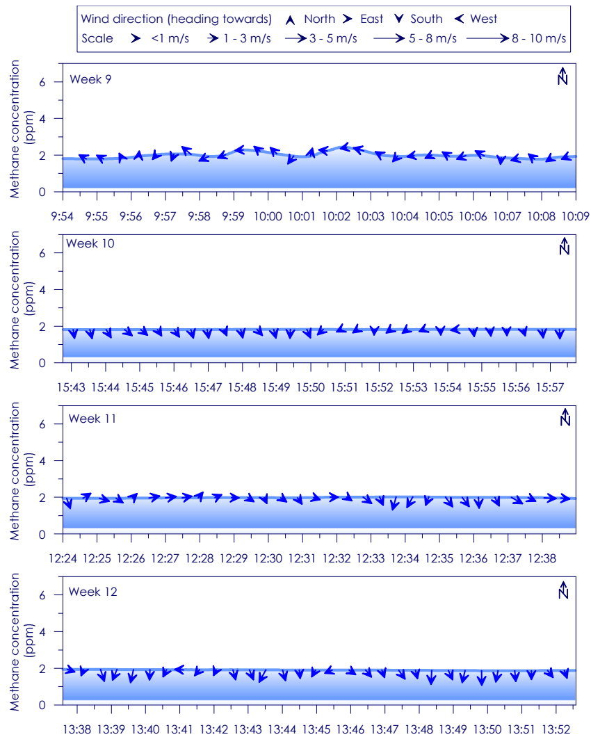
Figure C - 101: Time series of CH 4 concentration, wind speed and wind direction for Site 17 Weeks 9 - 12
