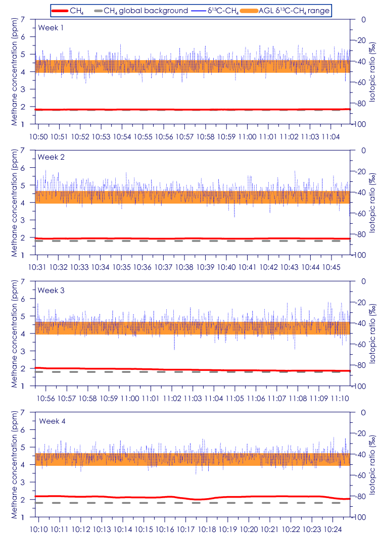
Figure C - 56: Time series of CH 4 concentration and isotopic ratio for Site 10 Weeks 1 - 4
