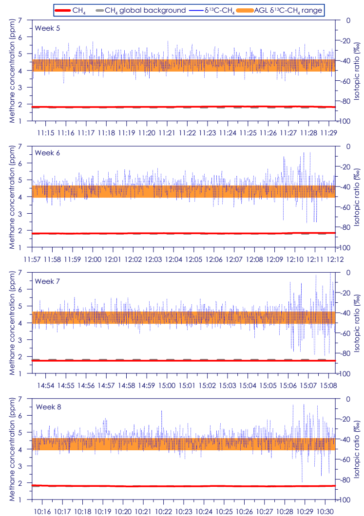
Figure C - 130: Time series of CH 4 concentration and isotopic ratio for Site 22 Weeks 5 - 8
