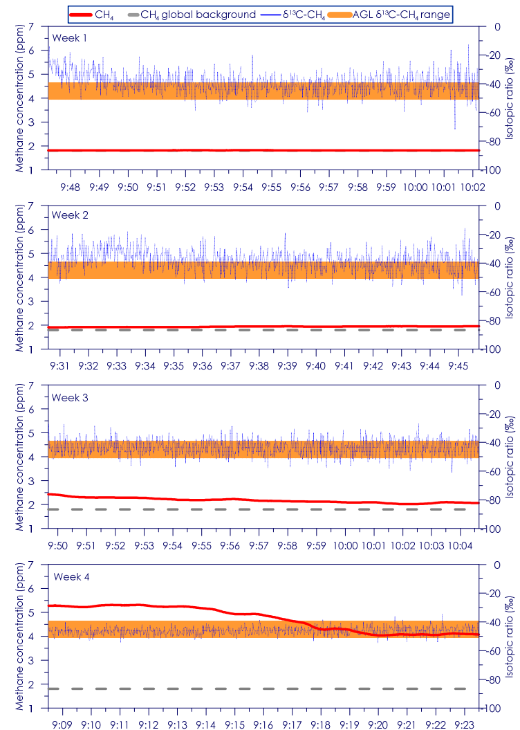
Figure C - 140: Time series of CH 4 concentration and isotopic ratio for Site 24 Weeks 1 - 4
