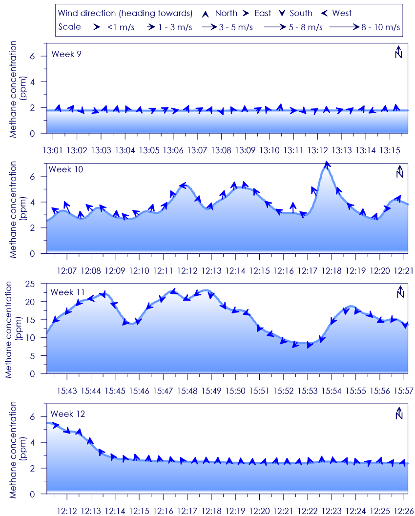
Figure C - 65: Time series of CH 4 concentration, wind speed and wind direction for Site 11 Weeks 9 - 12
