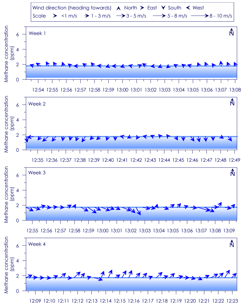
Figure C - 31: Time series of CH 4 concentration, wind speed and wind direction for Site 6 Weeks 1 - 4
