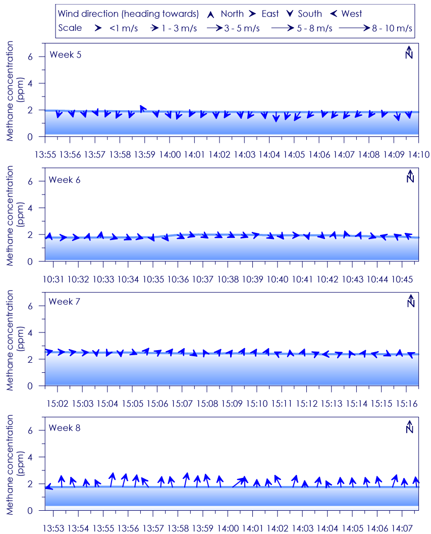
Figure C - 93: Time series of CH 4 concentration, wind speed and wind direction for Site 16 Weeks 5- 8
