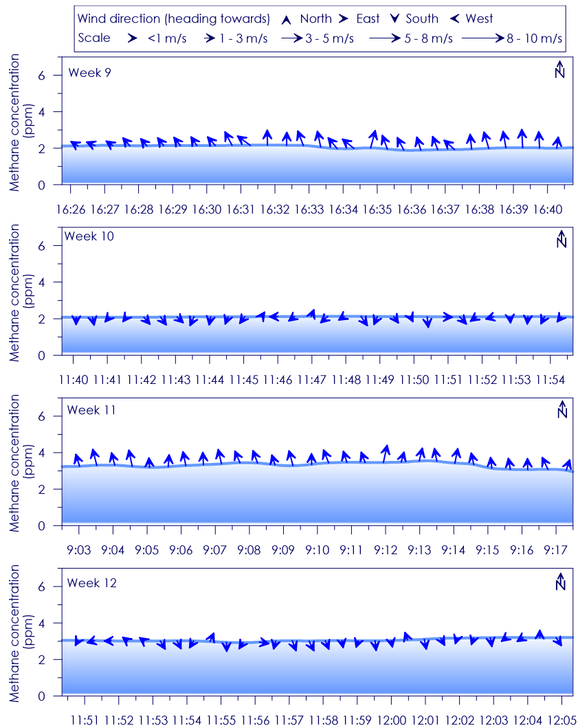
Figure C - 5: Time series of CH 4 concentration, wind speed and wind direction for Site 1 Weeks 9 - 12
