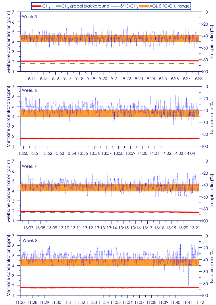
Figure C - 22: Time series of CH 4 concentration and isotopic ratio for Site 4 Weeks 5 - 8
