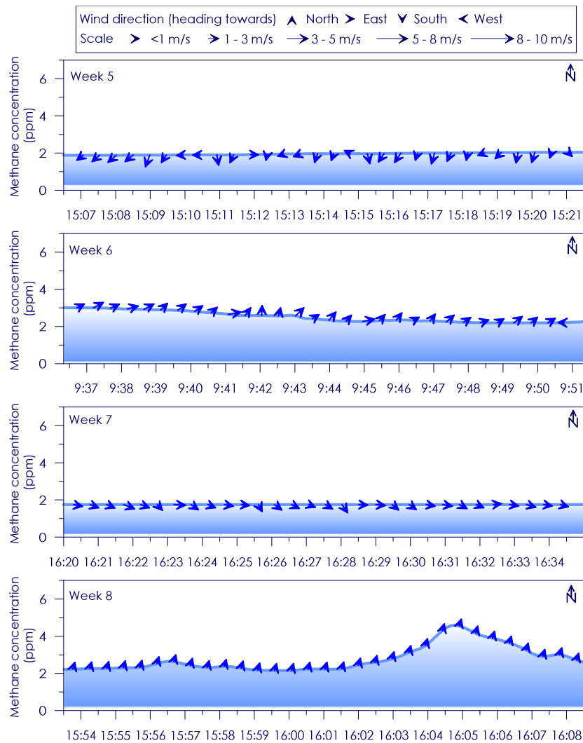
Figure C - 99: Time series of CH 4 concentration, wind speed and wind direction for Site 17 Weeks 5- 8
