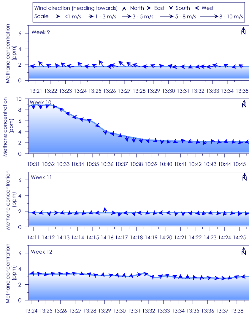
Figure C - 53: Time series of CH 4 concentration, wind speed and wind direction for Site 9 Weeks 9 - 12
