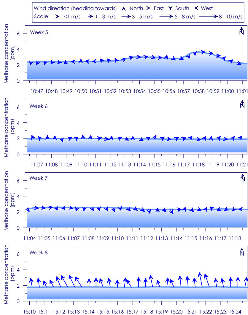
Figure C - 69: Time series of CH 4 concentration, wind speed and wind direction for Site 12 Weeks 5- 8
