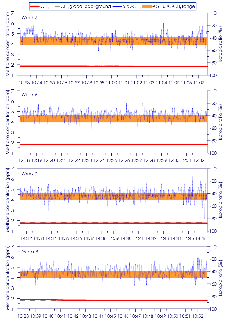
Figure C - 106: Time series of CH 4 concentration and isotopic ratio for Site 18 Weeks 5 - 8
