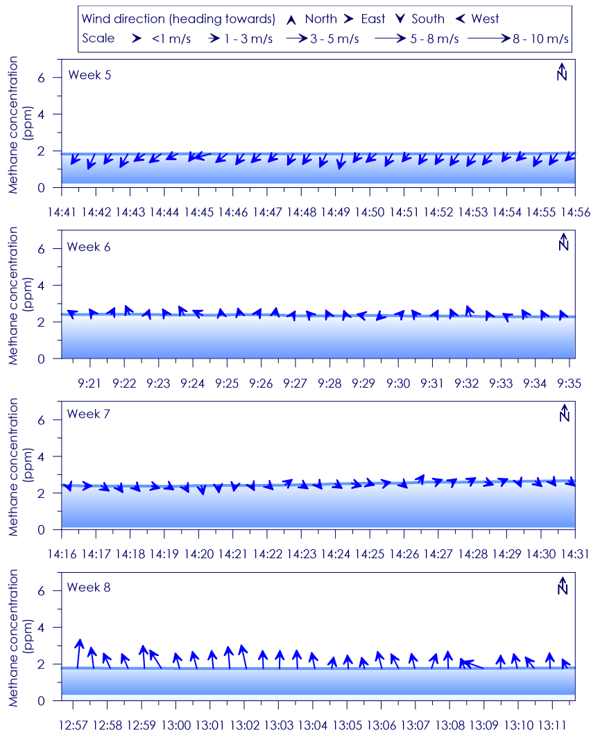
Figure C - 81: Time series of CH 4 concentration, wind speed and wind direction for Site 14 Weeks 5- 8
