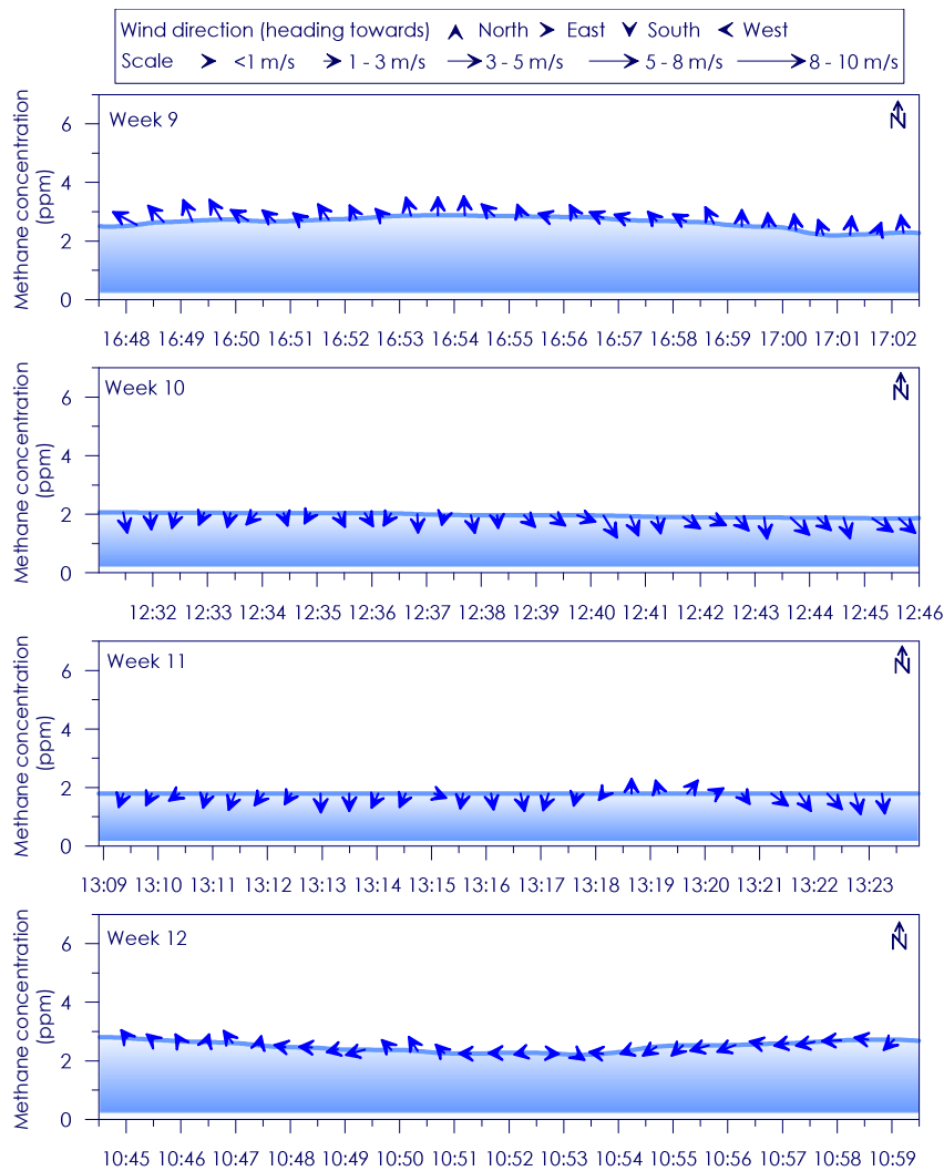
Figure C - 131: Time series of CH 4 concentration, wind speed and wind direction for Site 22 Weeks 9 - 12
