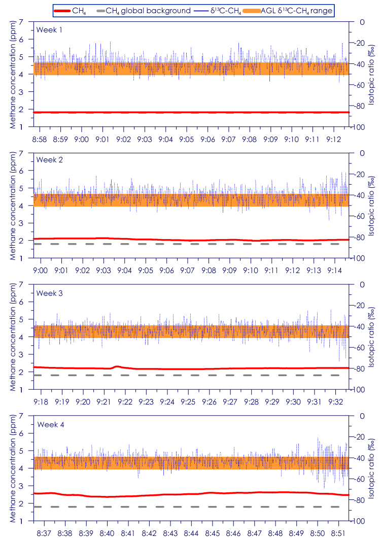
Figure C - 134: Time series of CH 4 concentration and isotopic ratio for Site 23 Weeks 1 - 4
