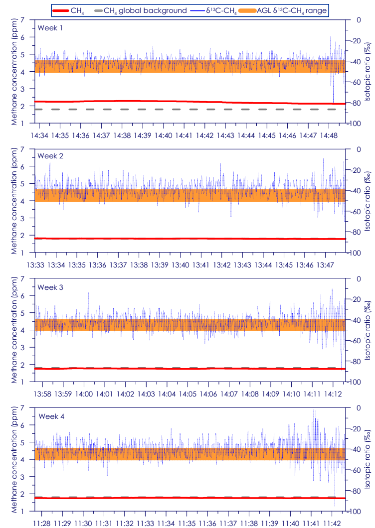
Figure C - 8: Time series of CH 4 concentration and isotopic ratio for Site 2 Weeks 1 - 4
