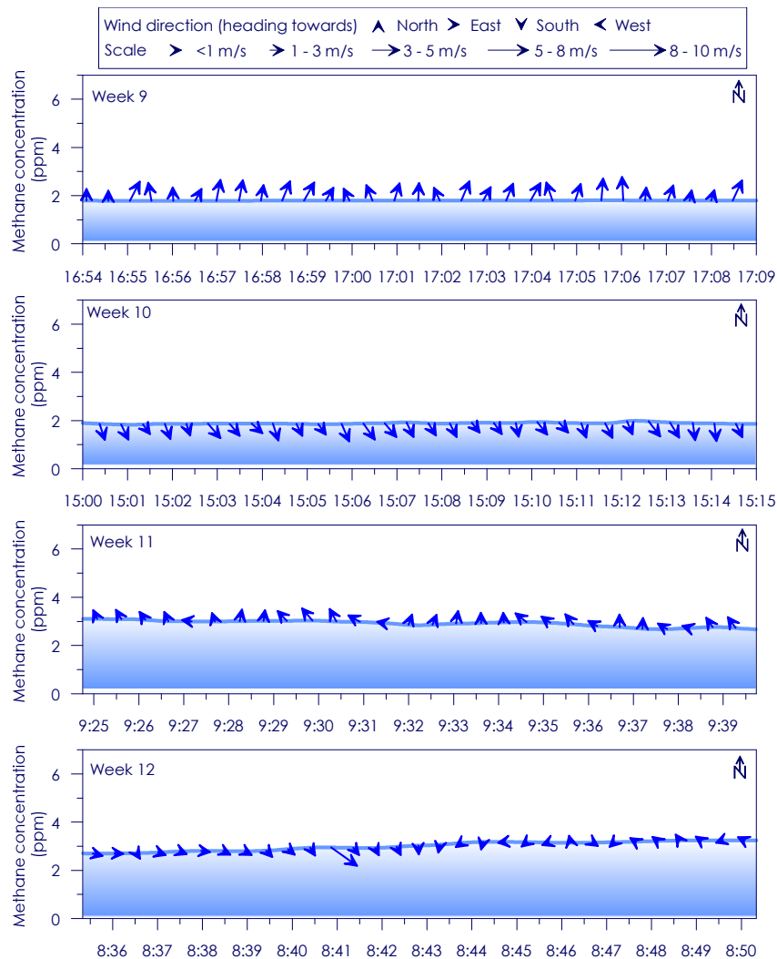
Figure C - 119: Time series of CH 4 concentration, wind speed and wind direction for Site 20 Weeks 9 - 12
