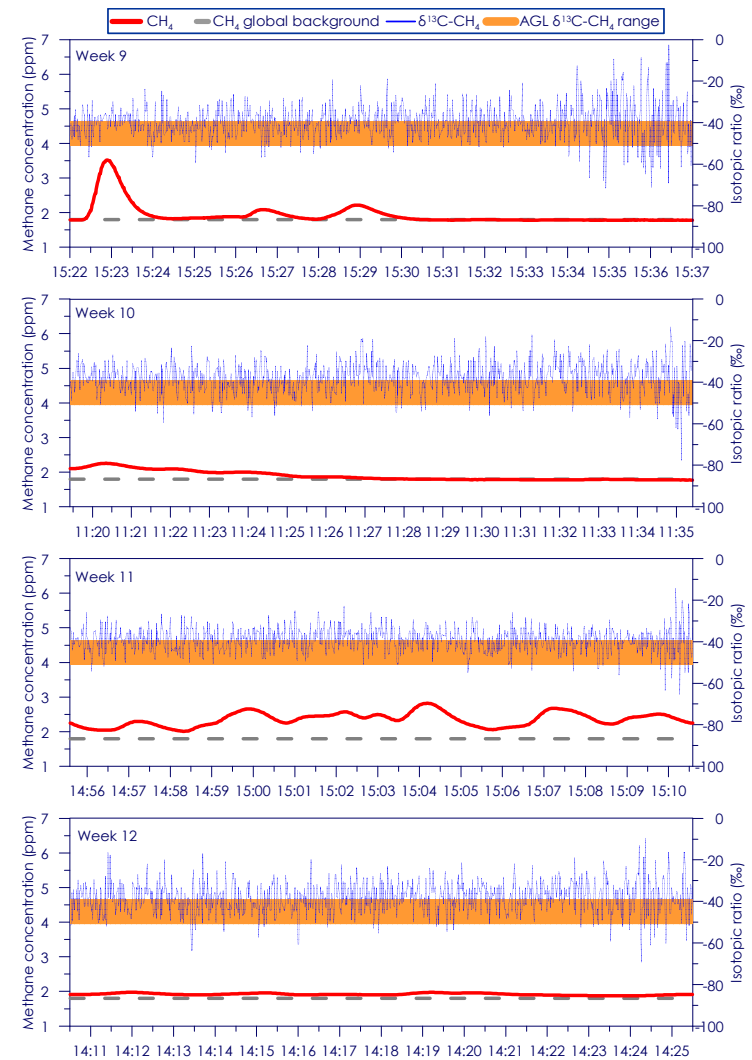
Figure C - 48: Time series of CH 4 concentration and isotopic ratio for Site 8 Weeks 9 - 12
