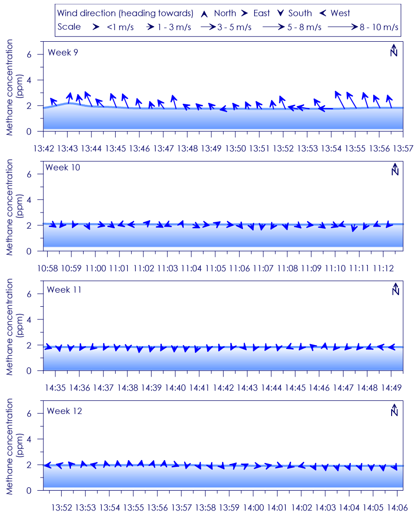
Figure C - 59: Time series of CH 4 concentration, wind speed and wind direction for Site 10 Weeks 9 - 12
