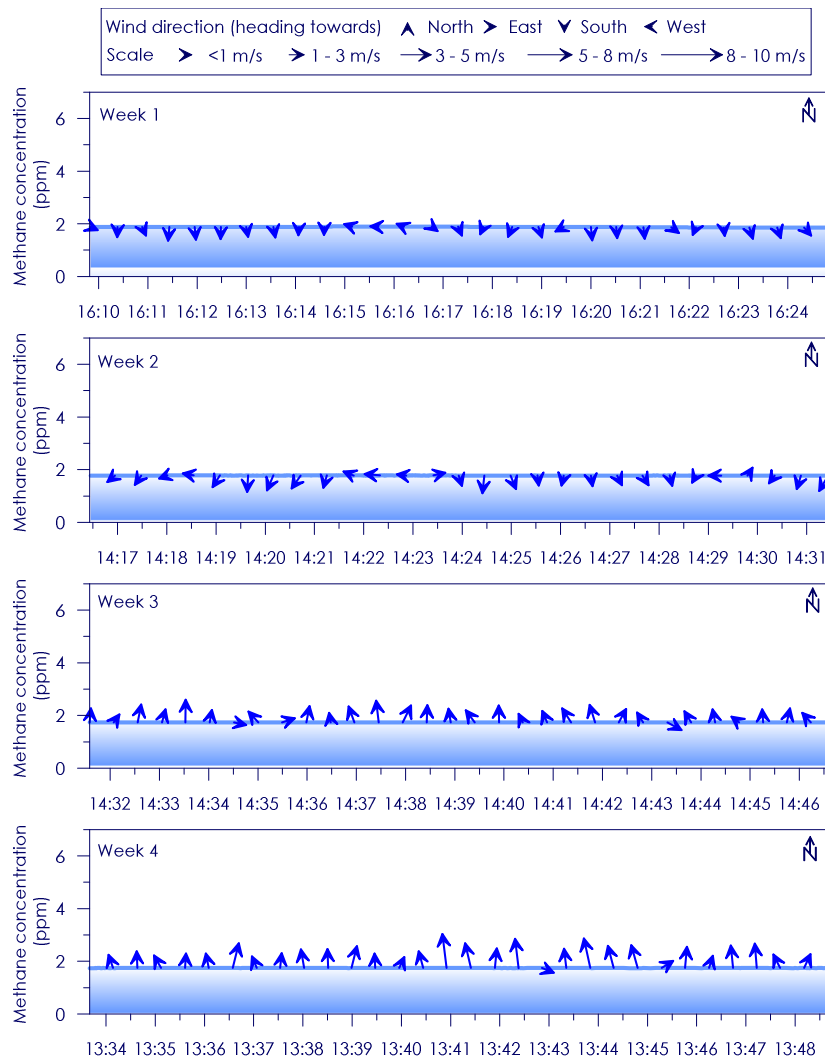
Figure C - 19: Time series of CH 4 concentration, wind speed and wind direction for Site 4 Weeks 1 - 4
