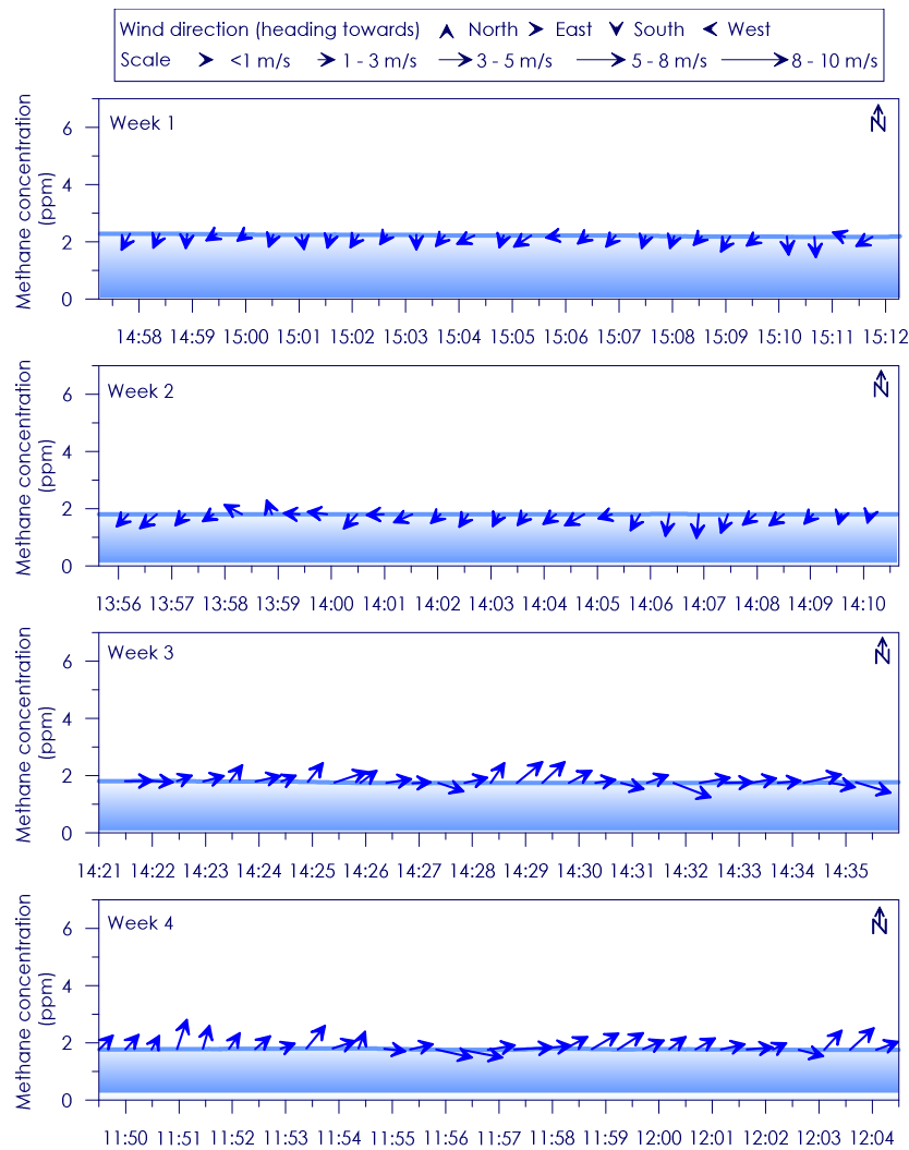
Figure C - 127: Time series of CH 4 concentration, wind speed and wind direction for Site 22 Weeks 1 - 4
