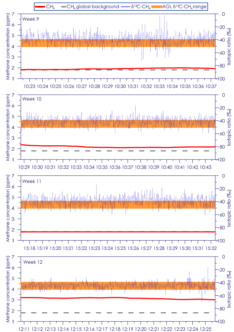
Figure C - 114: Time series of CH 4 concentration and isotopic ratio for Site 19 Weeks 9 - 12
