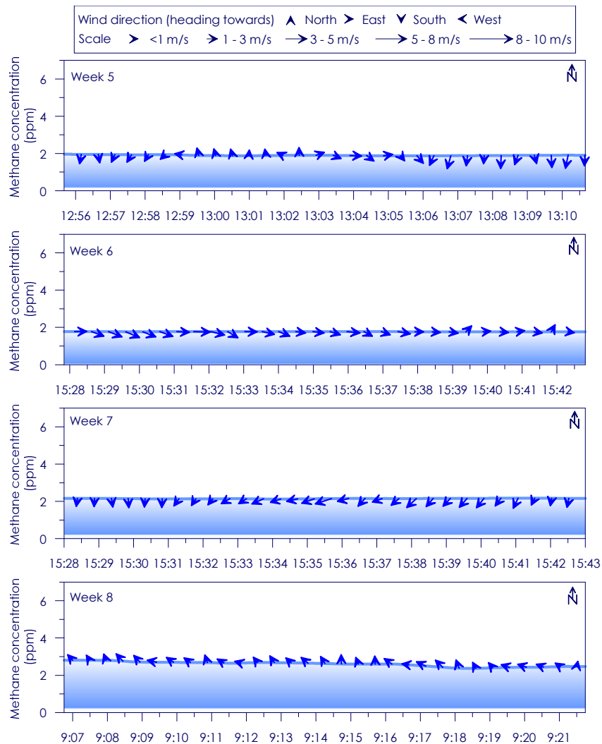
Figure C - 117: Time series of CH 4 concentration, wind speed and wind direction for Site 20 Weeks 5- 8
