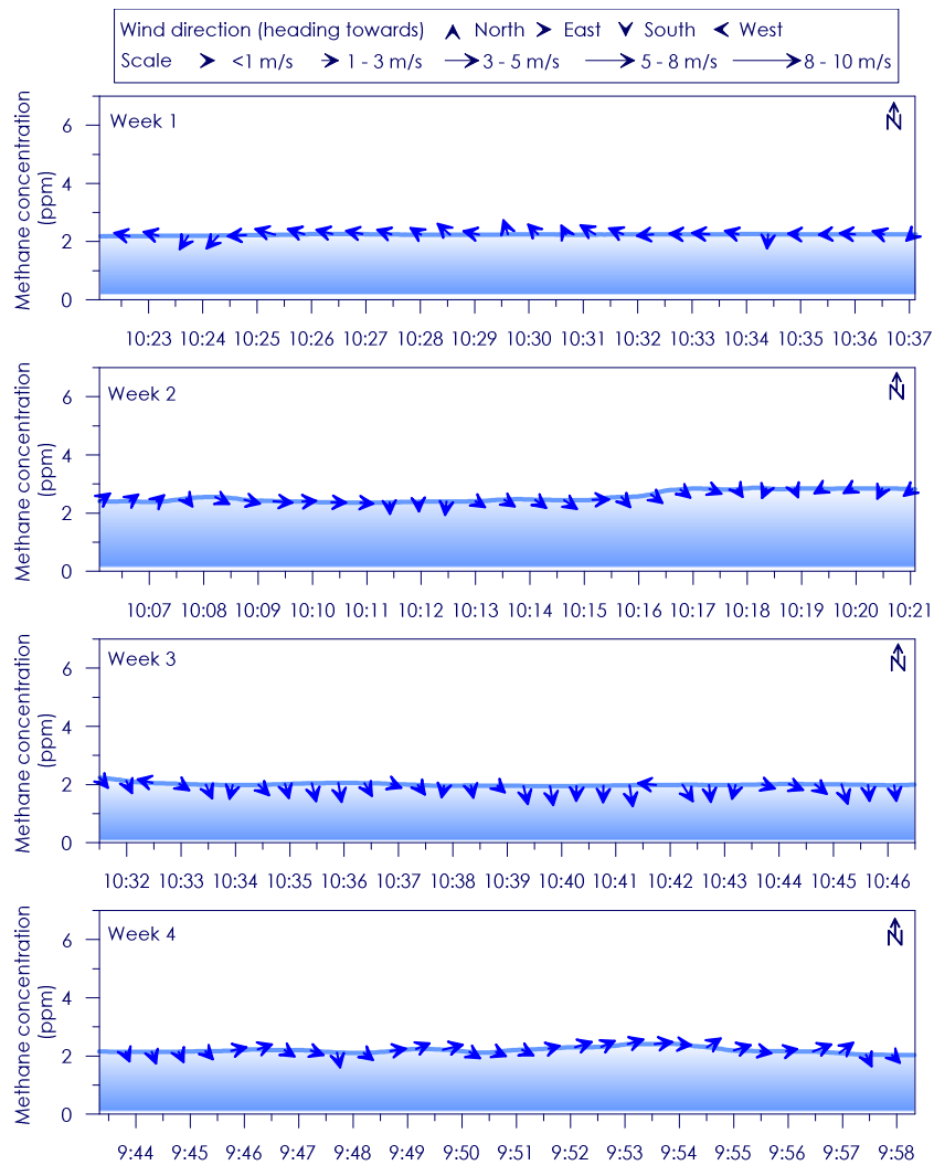
Figure C - 49: Time series of CH 4 concentration, wind speed and wind direction for Site 9 Weeks 1 - 4
