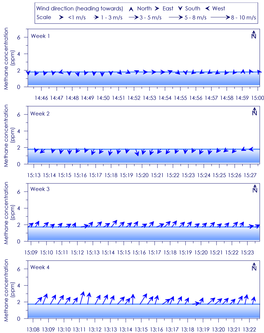
Figure C - 25: Time series of CH 4 concentration, wind speed and wind direction for Site 5 Weeks 1 - 4
