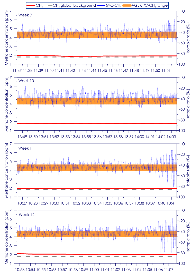
Figure C - 150: Time series of CH 4 concentration and isotopic ratio for Site 25 Weeks 9 - 12
