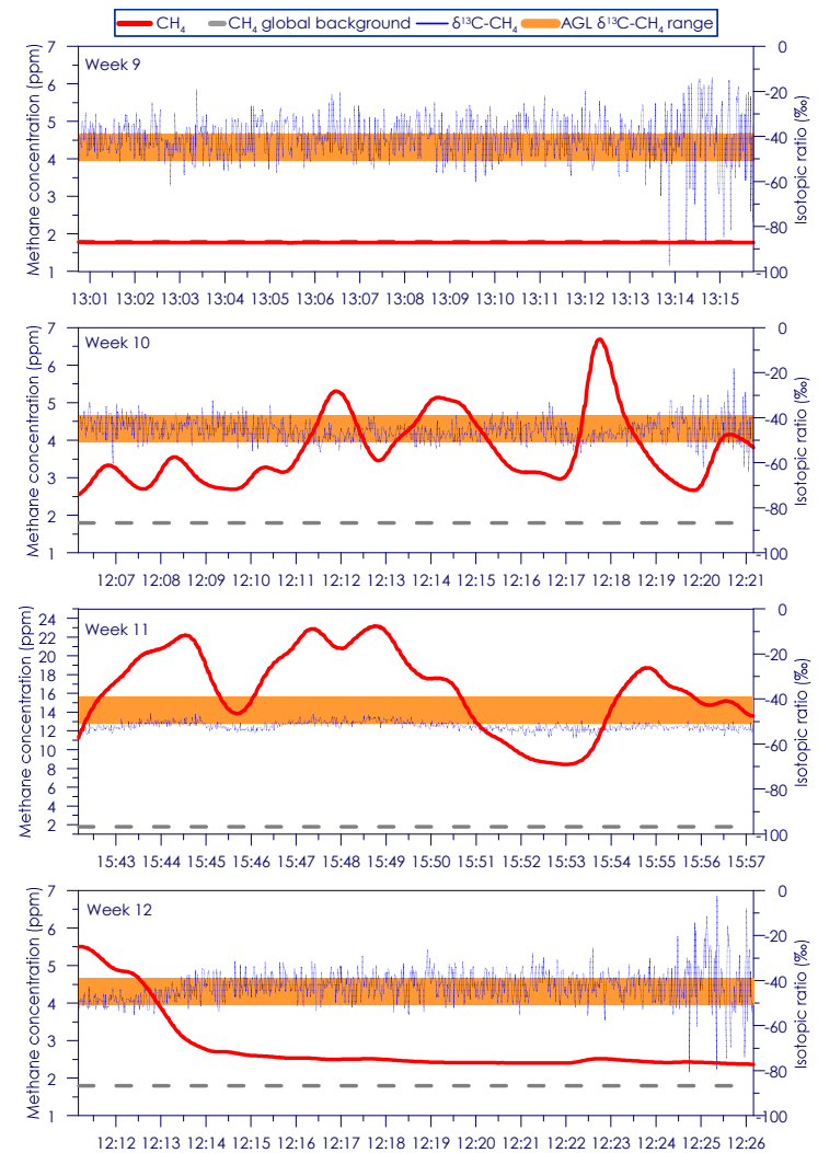
Figure C - 66: Time series of CH 4 concentration and isotopic ratio for Site 11 Weeks 9 - 12
