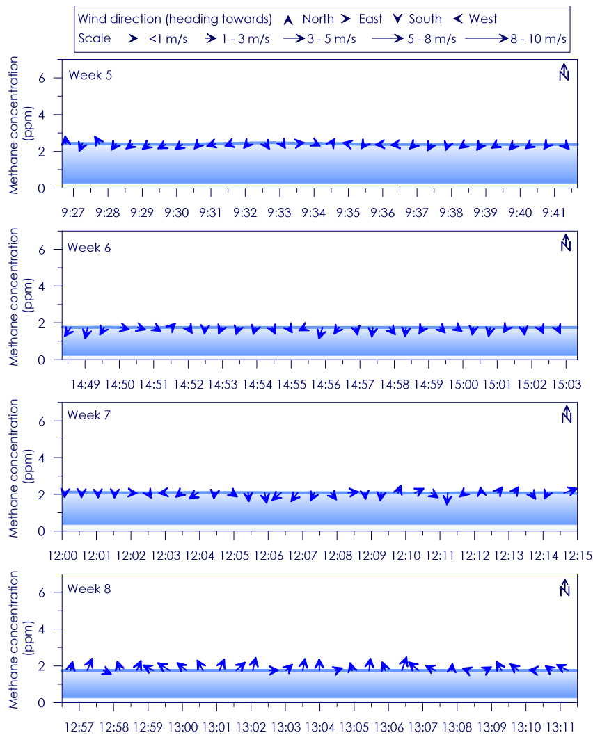
Figure C - 123: Time series of CH 4 concentration, wind speed and wind direction for Site 21 Weeks 5- 8
