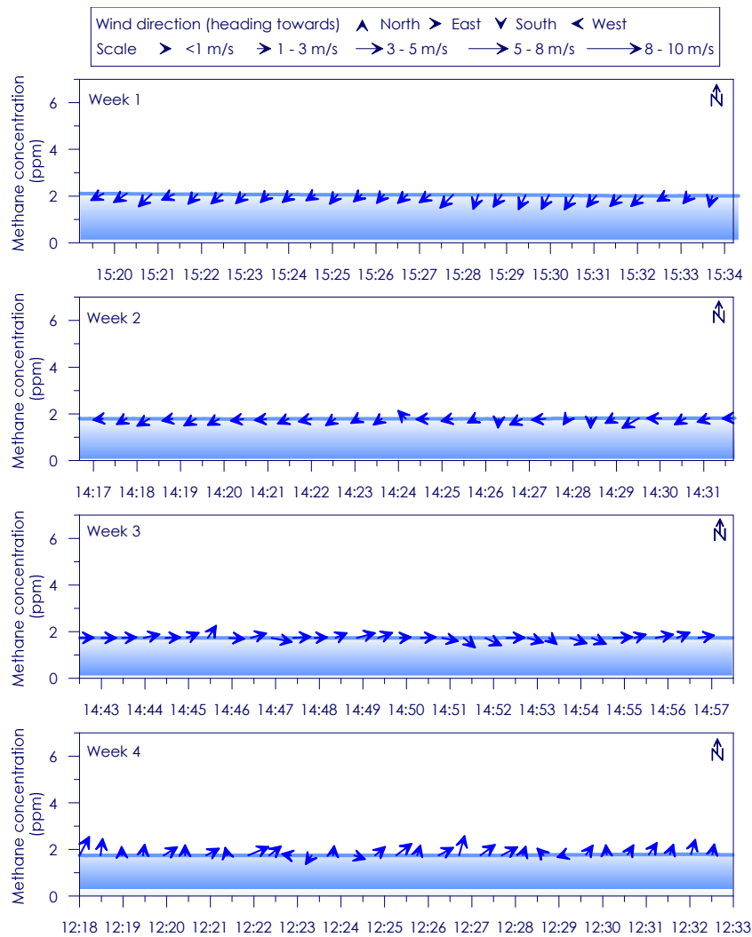
Figure C - 103: Time series of CH 4 concentration, wind speed and wind direction for Site 18 Weeks 1 - 4
