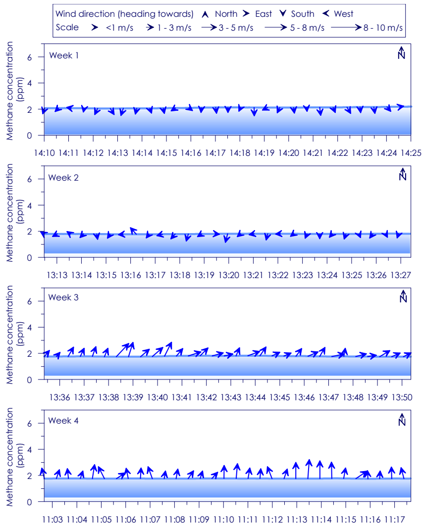
Figure C - 1: Time series of CH 4 concentration, wind speed and wind direction for Site 1 Weeks 1 - 4
