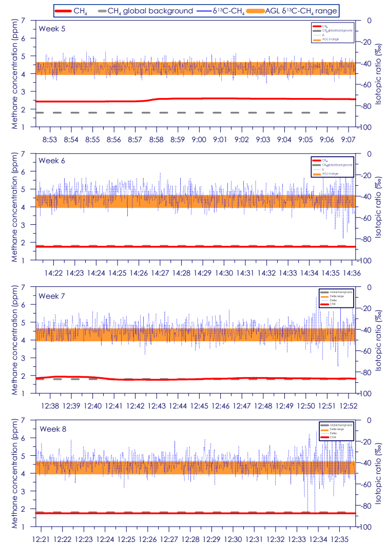
Figure C - 148: Time series of CH 4 concentration and isotopic ratio for Site 25 Weeks 5 - 8
