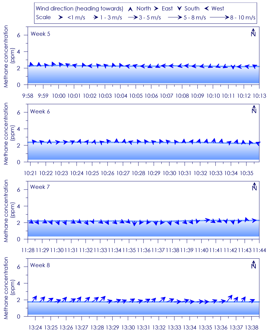
Figure C - 33: Time series of CH 4 concentration, wind speed and wind direction for Site 6 Weeks 5 - 8
