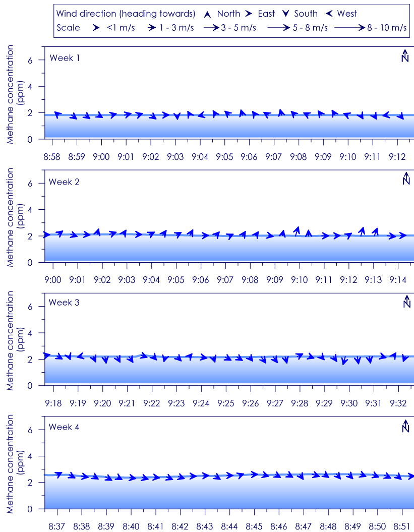
Figure C - 133: Time series of CH 4 concentration, wind speed and wind direction for Site 23 Weeks 1 - 4
