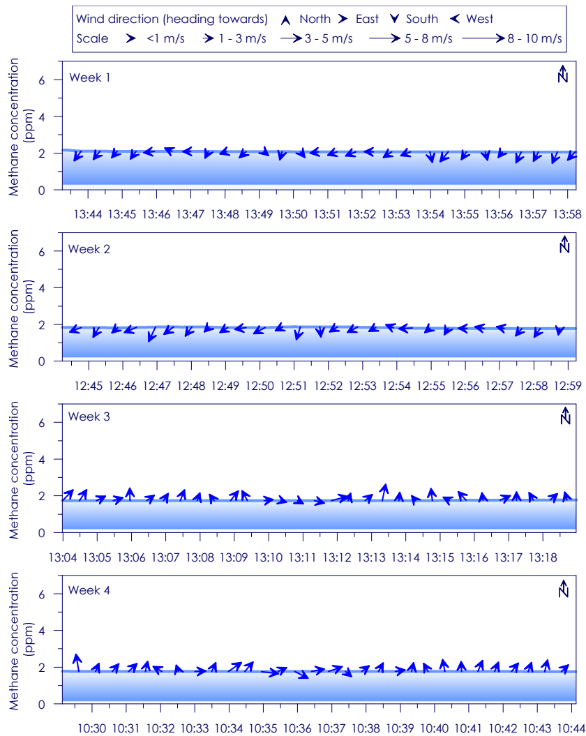
Figure C - 109: Time series of CH 4 concentration, wind speed and wind direction for Site 19 Weeks 1 - 4
