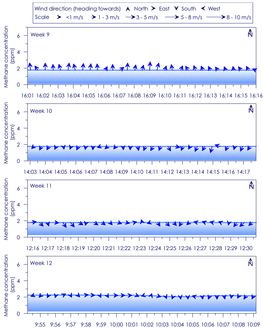
Figure C - 29: Time series of CH 4 concentration, wind speed and wind direction for Site 5 Weeks 9 - 12
