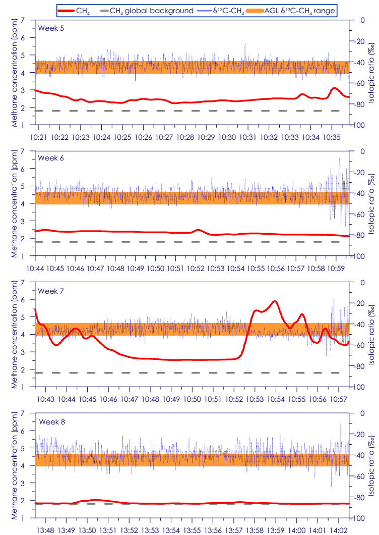
Figure C - 64: Time series of CH 4 concentration and isotopic ratio for Site 11 Weeks 5 - 8
