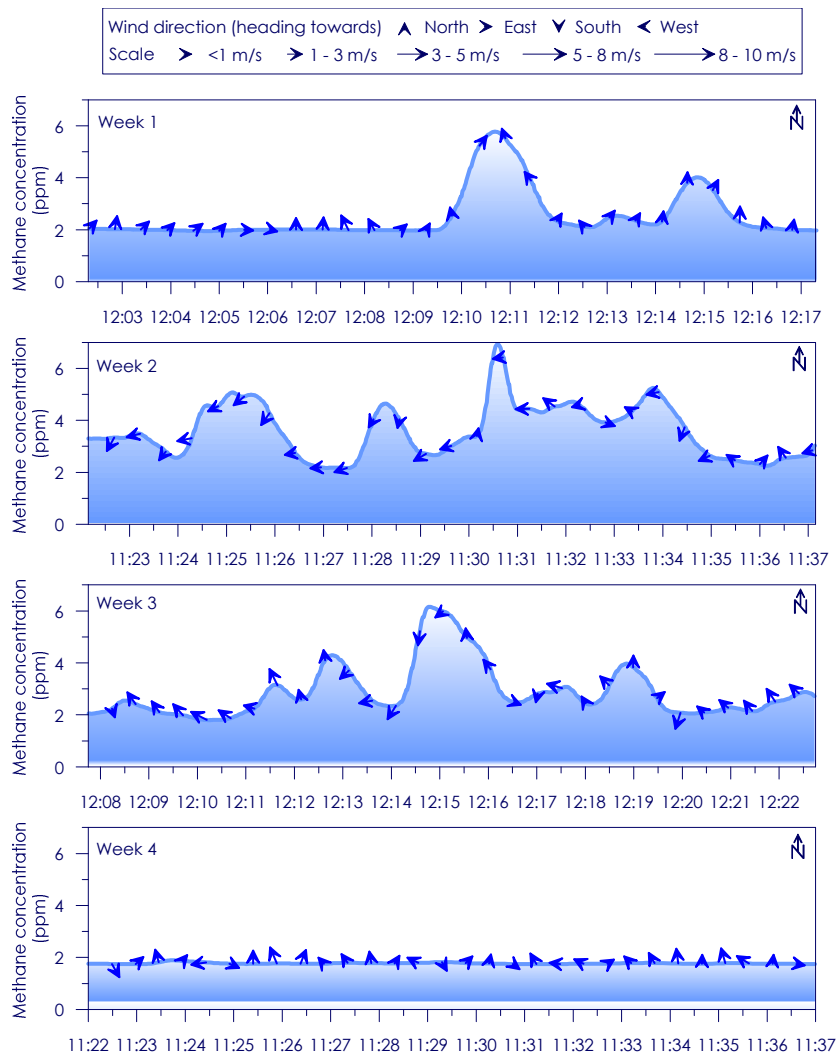
Figure C - 61: Time series of CH 4 concentration, wind speed and wind direction for Site 11 Weeks 1 - 4
