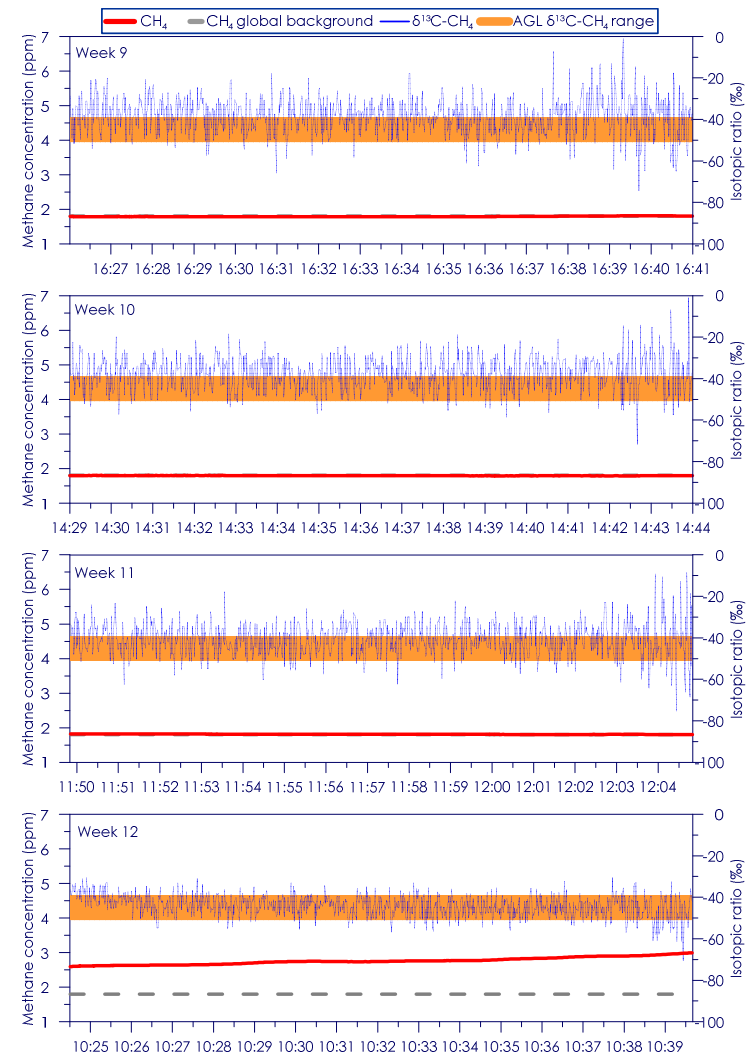
Figure C - 18: Time series of CH 4 concentration and isotopic ratio for Site 3 Weeks 9 - 12
