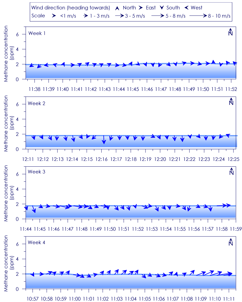
Figure C - 37: Time series of CH 4 concentration, wind speed and wind direction for Site 7 Weeks 1 - 4
