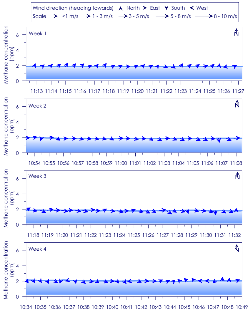
Figure C - 43: Time series of CH 4 concentration, wind speed and wind direction for Site 8 Weeks 1 - 4
