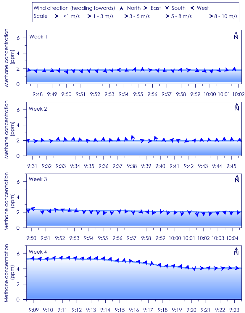
Figure C - 139: Time series of CH 4 concentration, wind speed and wind direction for Site 24 Weeks 1 - 4
