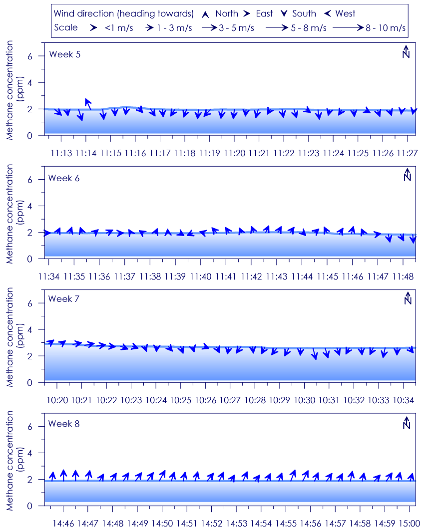
Figure C - 39: Time series of CH 4 concentration, wind speed and wind direction for Site 7 Weeks 5 - 8
