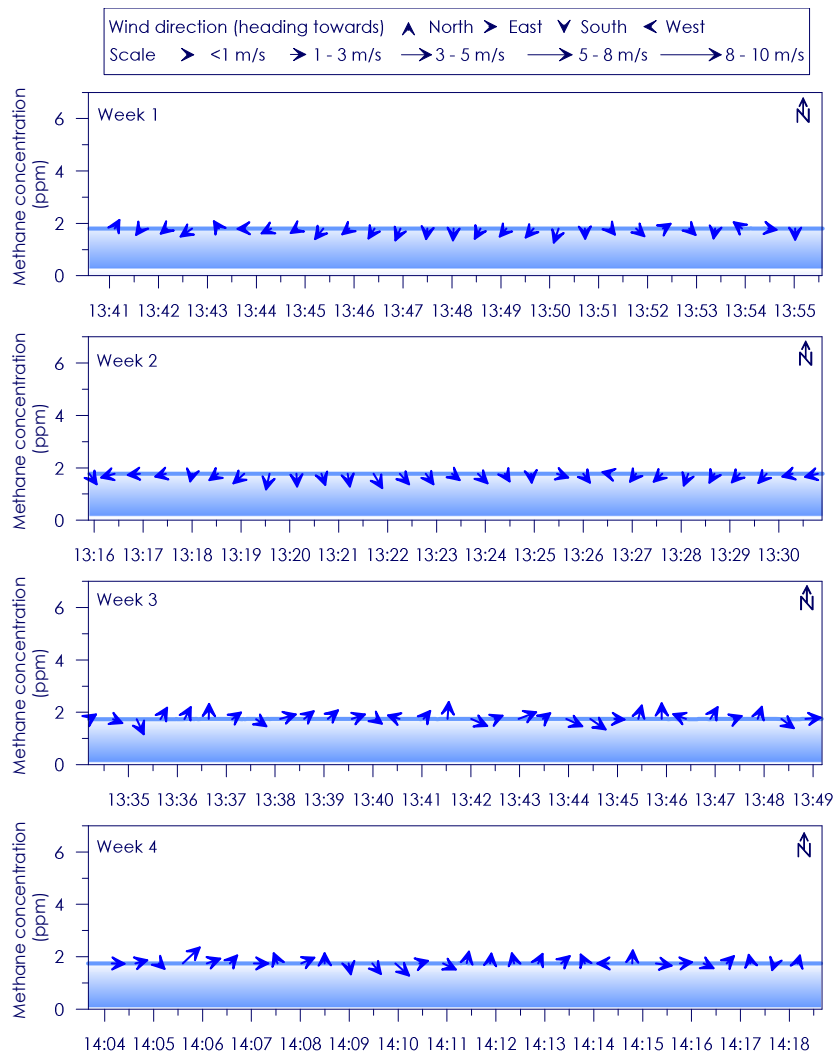
Figure C - 121: Time series of CH 4 concentration, wind speed and wind direction for Site 21 Weeks 1 - 4
