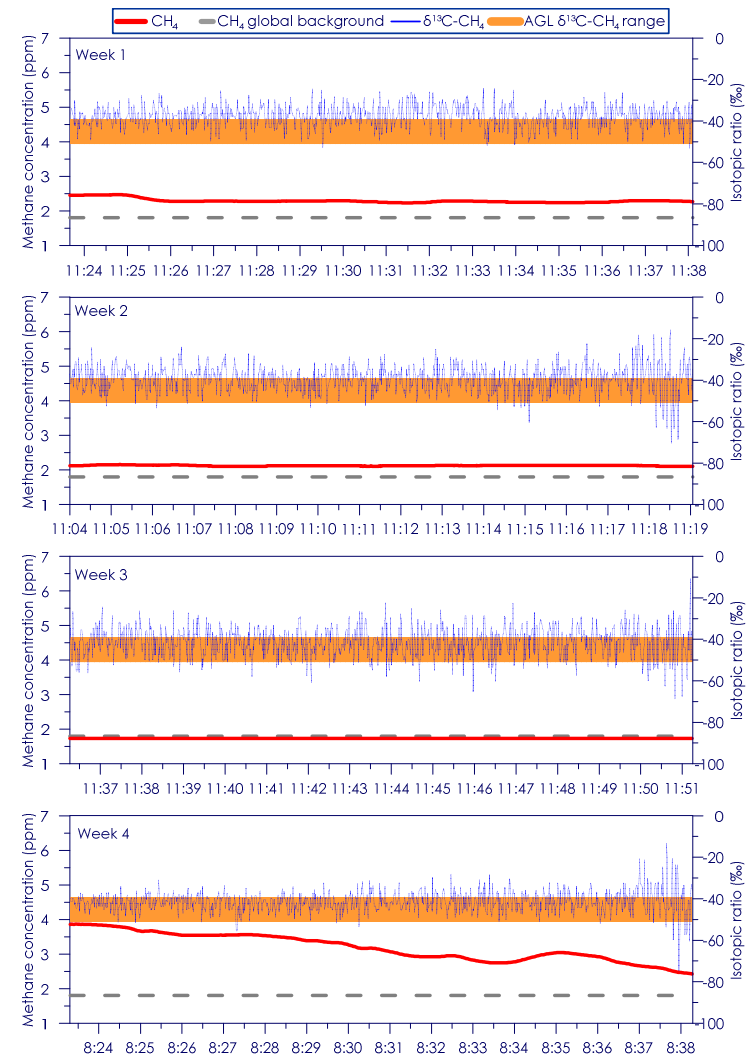
Figure C - 74: Time series of CH 4 concentration and isotopic ratio for Site 13 Weeks 1 - 4
