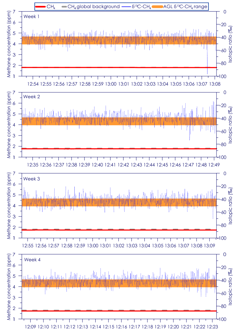
Figure C - 32: Time series of CH 4 concentration and isotopic ratio for Site 6 Weeks 1 - 4
