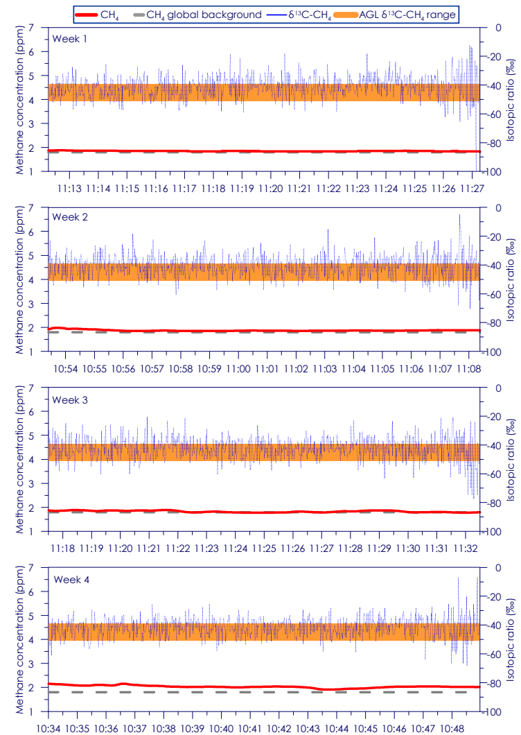
Figure C - 44: Time series of CH 4 concentration and isotopic ratio for Site 8 Weeks 1 - 4
