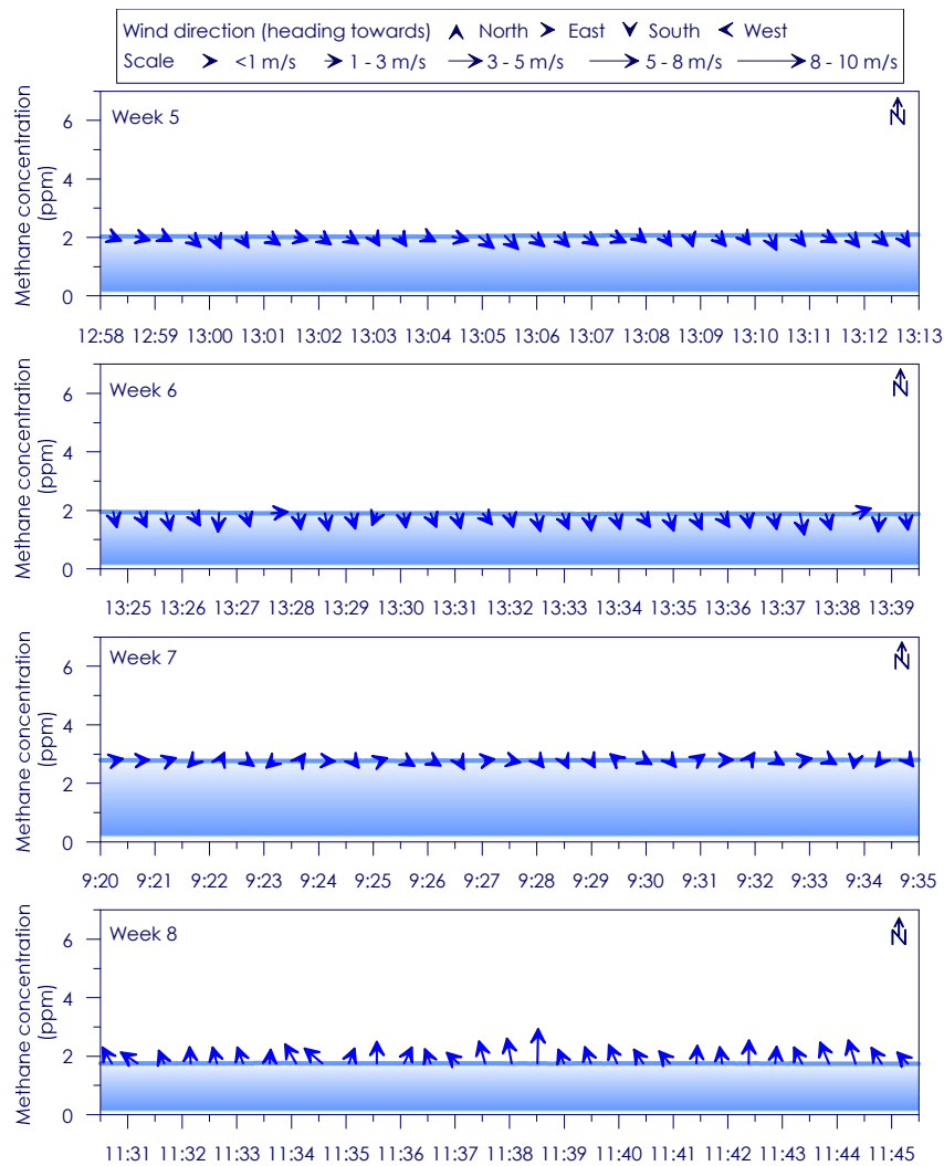
Figure C - 141: Time series of CH 4 concentration, wind speed and wind direction for Site 24 Weeks 5- 8
