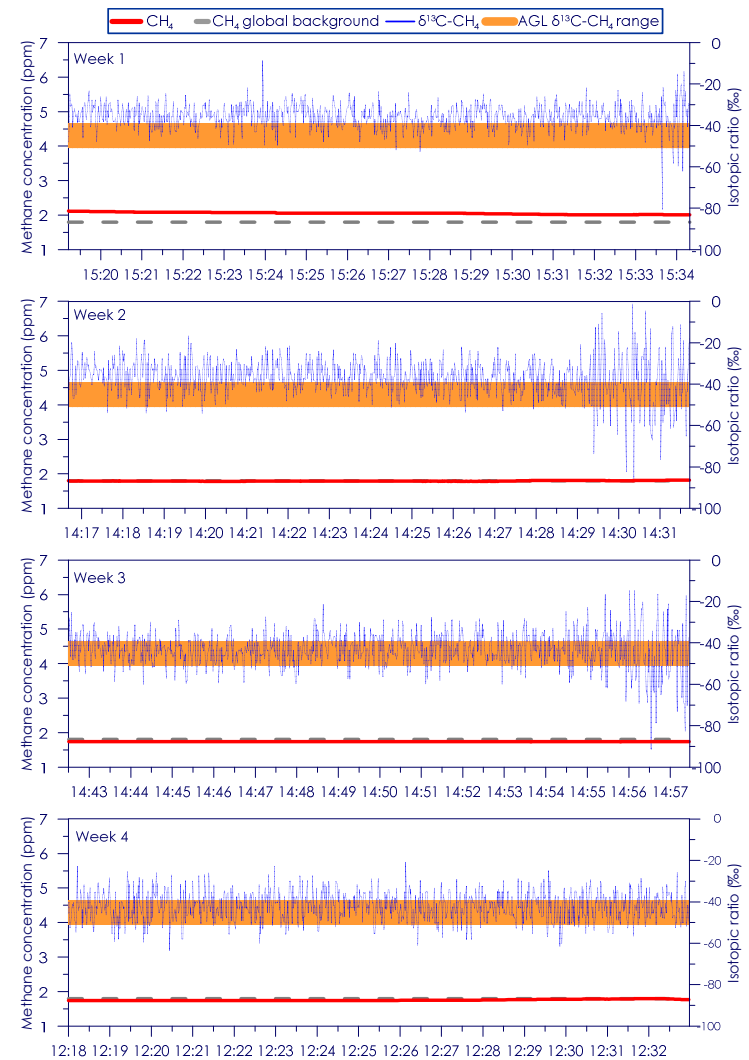
Figure C - 104: Time series of CH 4 concentration and isotopic ratio for Site 18 Weeks 1 - 4
