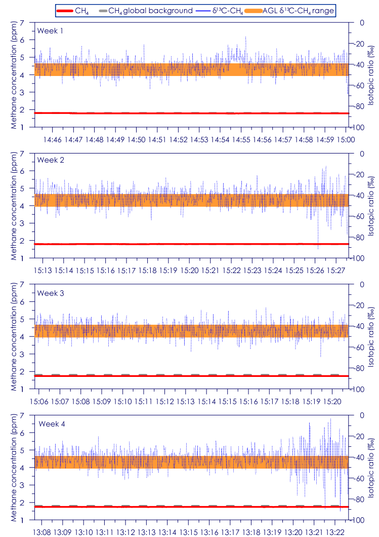
Figure C - 26: Time series of CH 4 concentration and isotopic ratio for Site 5 Weeks 1 - 4
