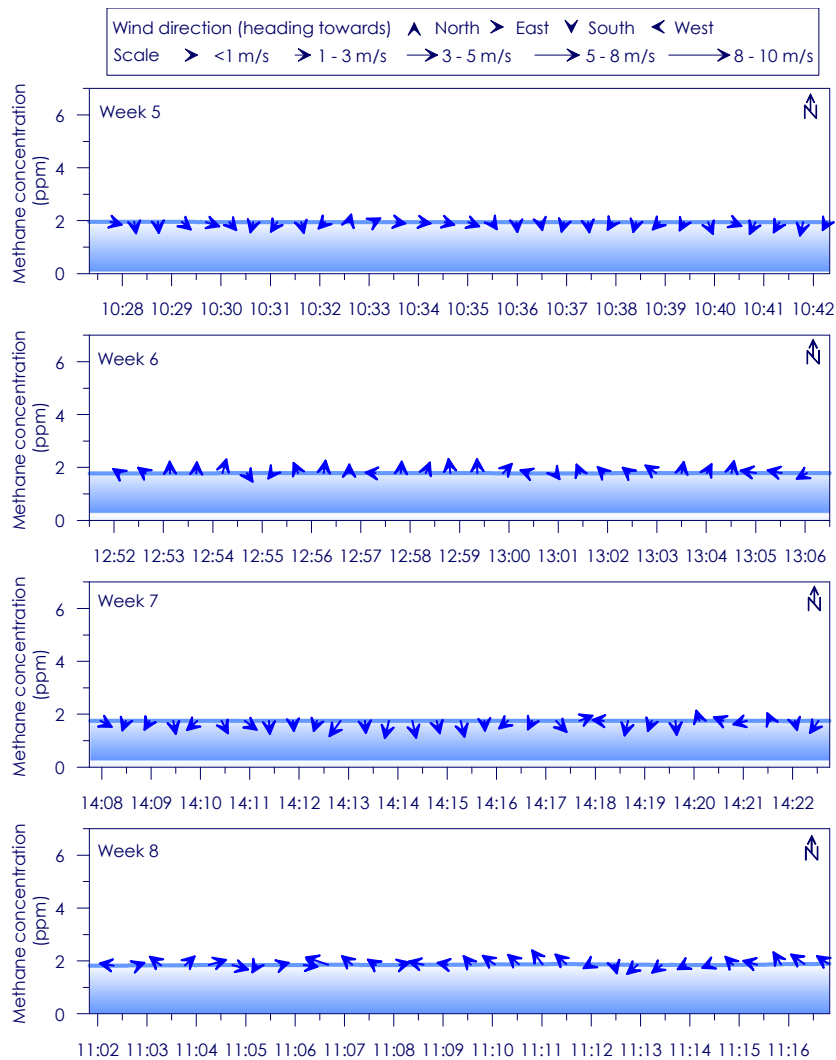
Figure C - 15: Time series of CH 4 concentration, wind speed and wind direction for Site 3 Weeks 5 - 8
