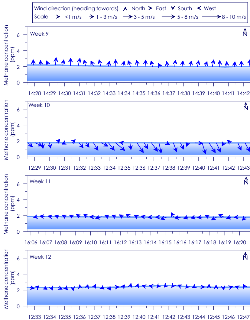
Figure C - 71: Time series of CH 4 concentration, wind speed and wind direction for Site 12 Weeks 9 - 12
