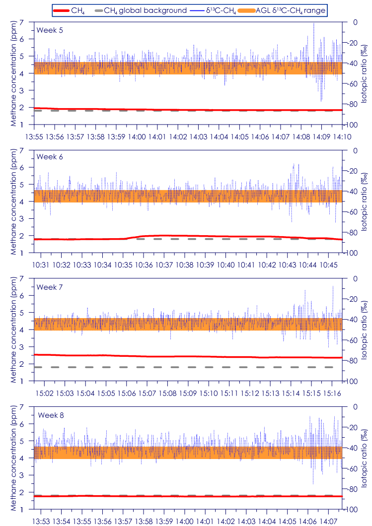
Figure C - 94: Time series of CH 4 concentration and isotopic ratio for Site 16 Weeks 5 - 8
