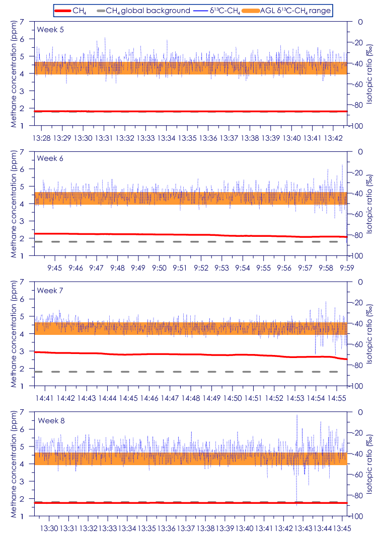
Figure C - 88: Time series of CH 4 concentration and isotopic ratio for Site 15 Weeks 5 - 8
