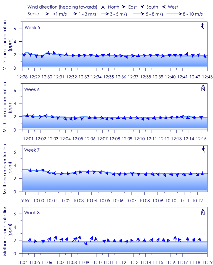
Figure C - 45: Time series of CH 4 concentration, wind speed and wind direction for Site 8 Weeks 5 - 8
