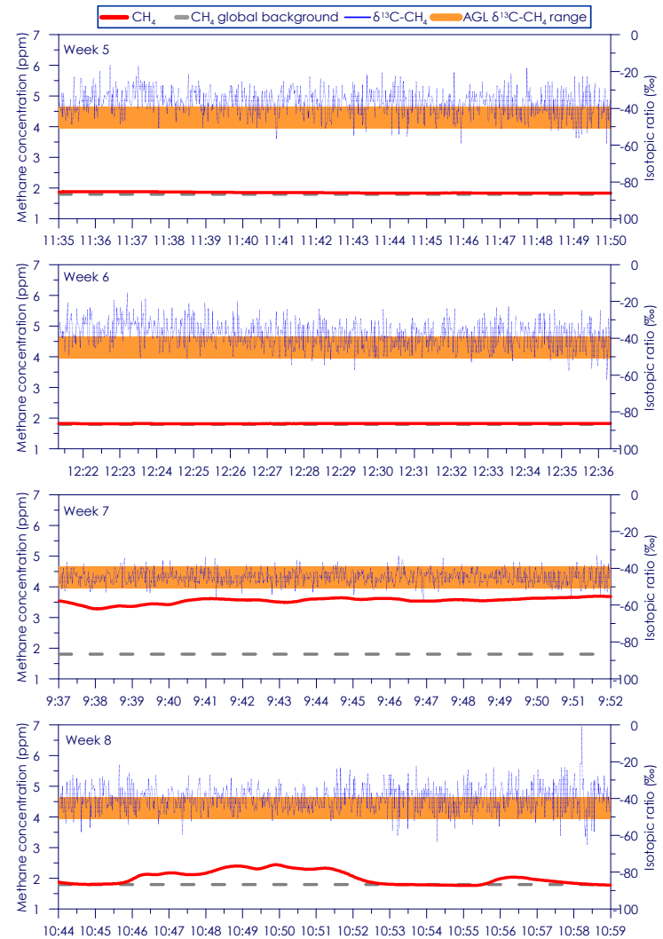
Figure C - 58: Time series of CH 4 concentration and isotopic ratio for Site 10 Weeks 5 - 8
