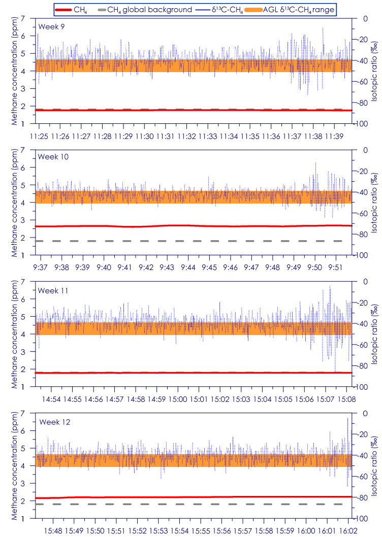
Figure C - 78: Time series of CH 4 concentration and isotopic ratio for Site 13 Weeks 9 - 12
