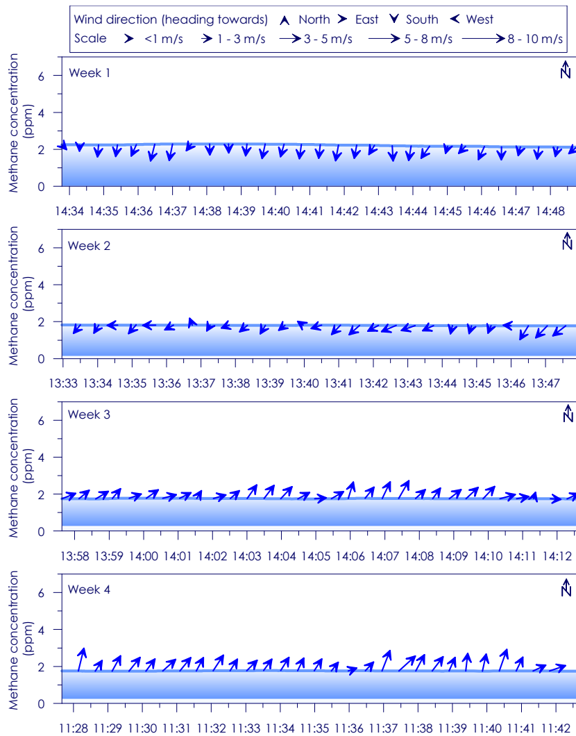
Figure C - 7: Time series of CH 4 concentration, wind speed and wind direction for Site 2 Weeks 1 - 4
