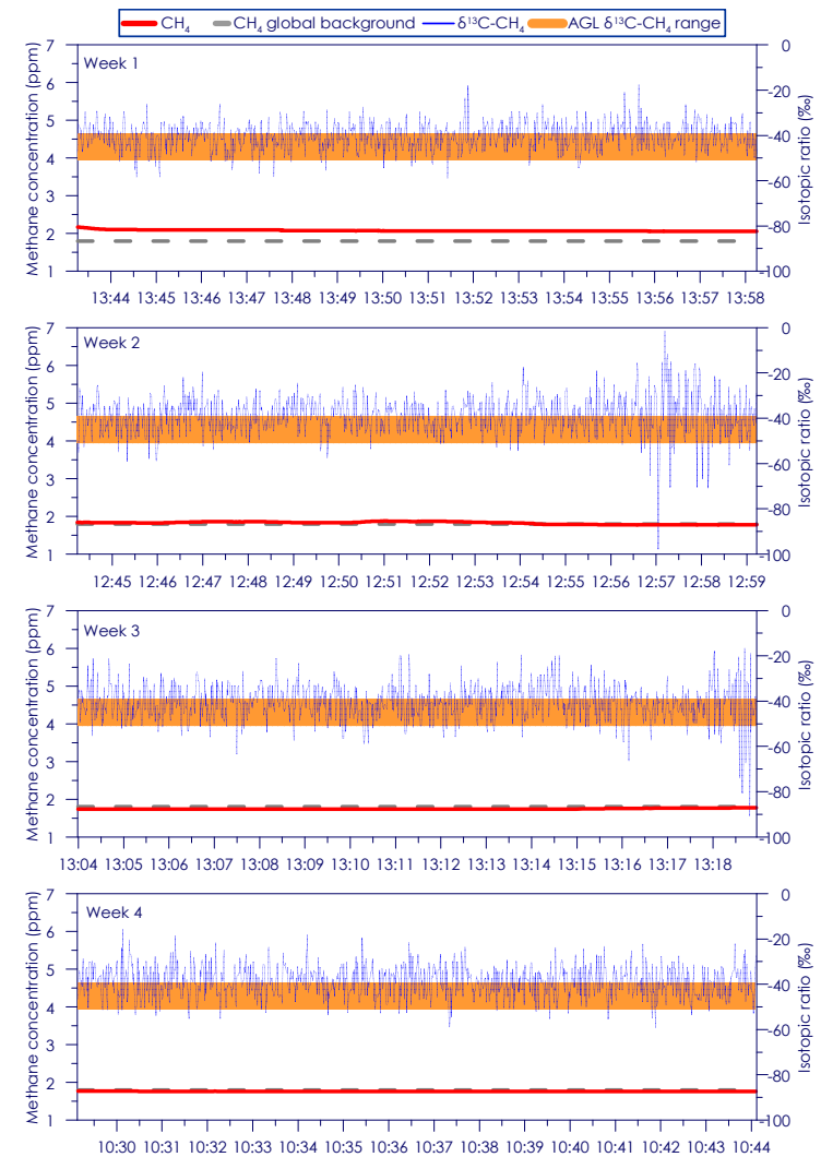
Figure C - 116: Time series of CH 4 concentration and isotopic ratio for Site 20 Weeks 1 - 4
