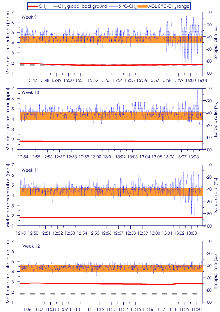
Figure C - 108: Time series of CH 4 concentration and isotopic ratio for Site 18 Weeks 9 - 12
