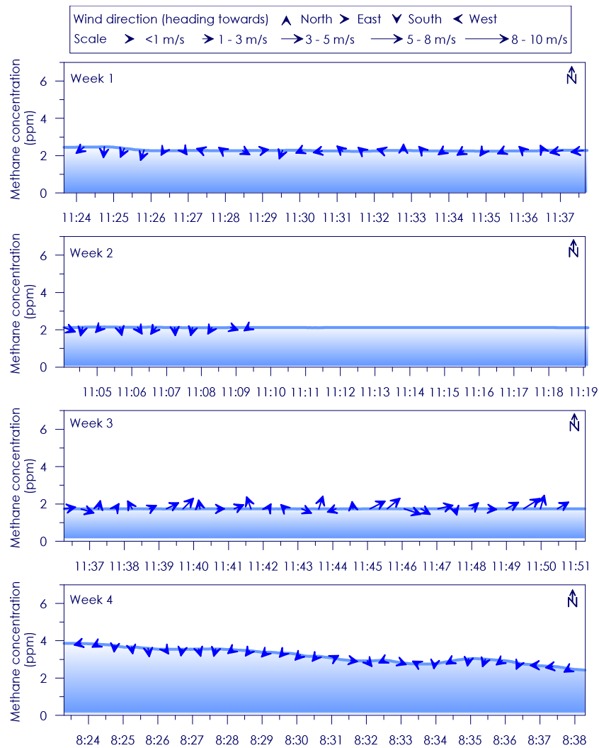
Figure C - 73: Time series of CH 4 concentration, wind speed and wind direction for Site 13 Weeks 1 - 4
