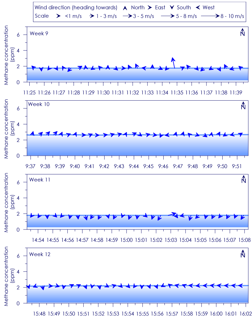
Figure C - 77: Time series of CH 4 concentration, wind speed and wind direction for Site 13 Weeks 9 - 12
