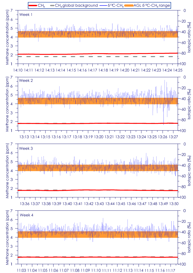
Figure C - 2: Time series of CH 4 concentration and isotopic ratio for Site 1 Weeks 1 - 4
