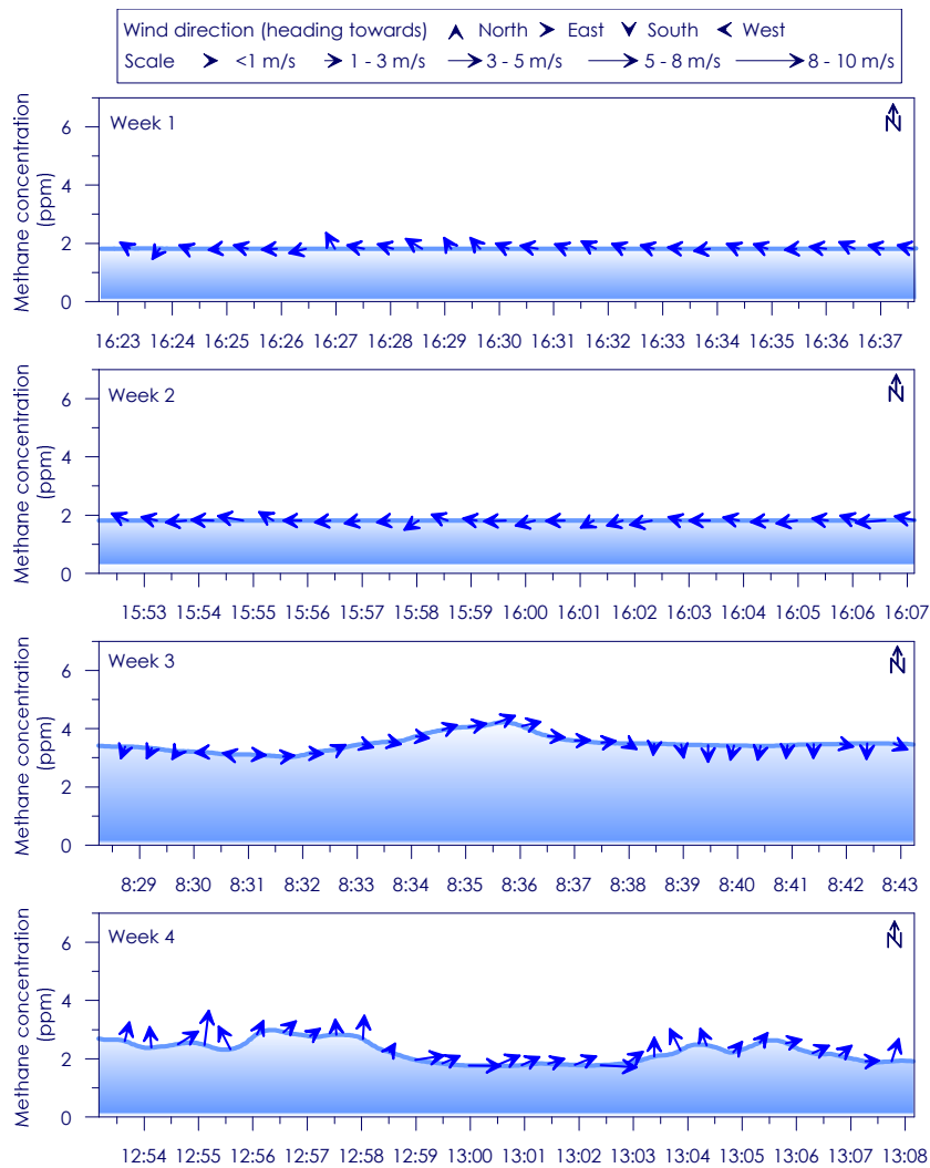
Figure C - 97: Time series of CH 4 concentration, wind speed and wind direction for Site 17 Weeks 1 - 4
