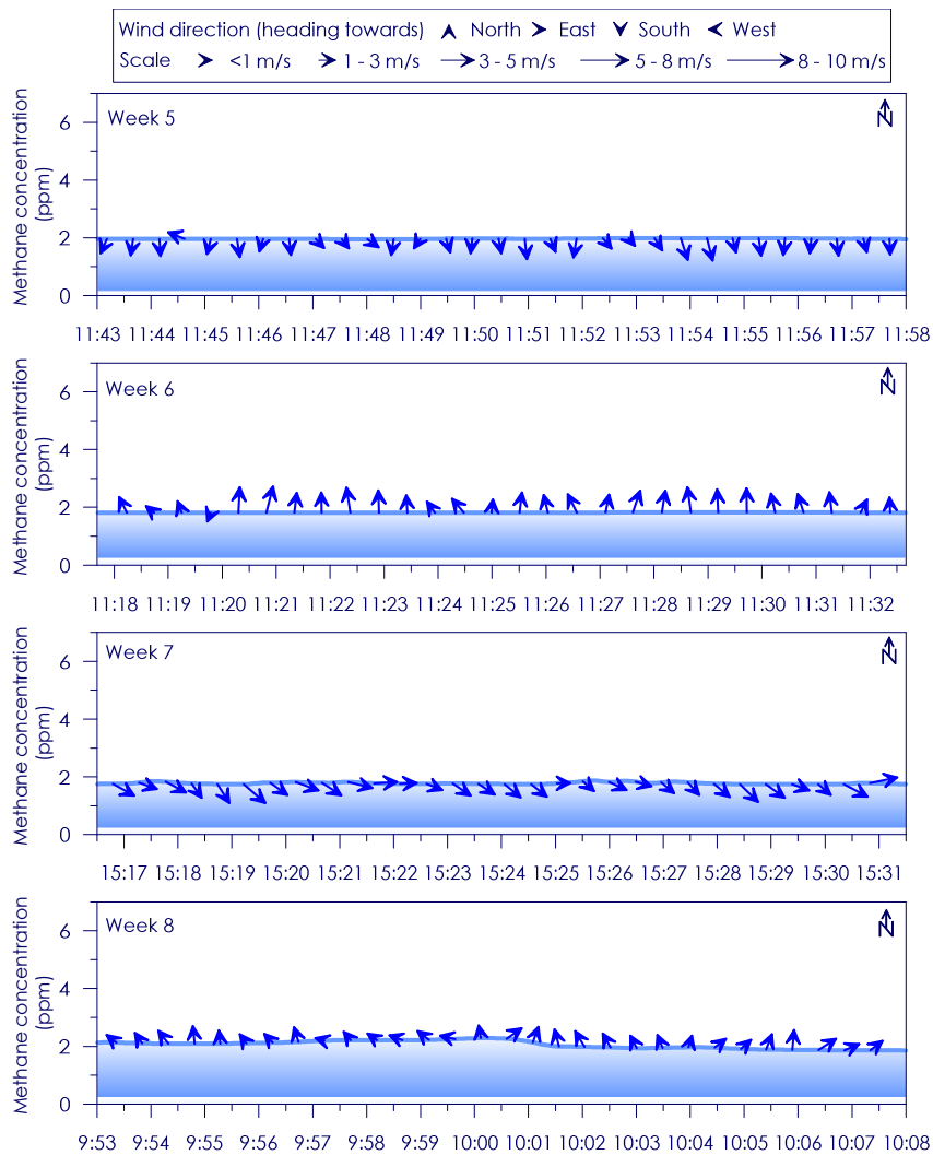
Figure C - 9: Time series of CH 4 concentration, wind speed and wind direction for Site 2 Weeks 5 - 8
