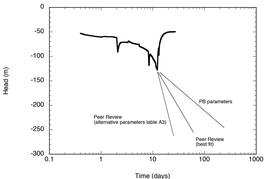
Figure 5.1: Projected drawdown over time for the flow testing showing the projected drawdown using PB’s long time conductivity parameter (their Table 6.5 K=0.005 m/day) and the two sets of parameters derived by the peer reviewer (Table A3).
