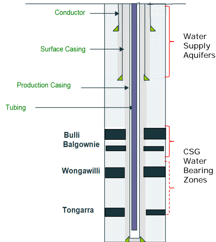
Typical vertical well design
