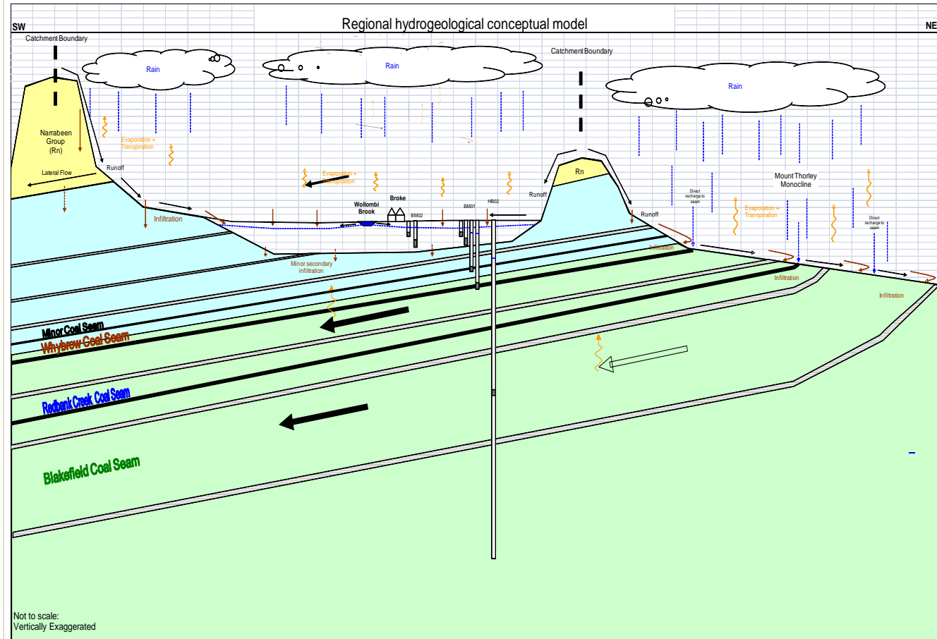
Hunter (Broke) Conceptual Cross sectional model (after PB, 2010)
